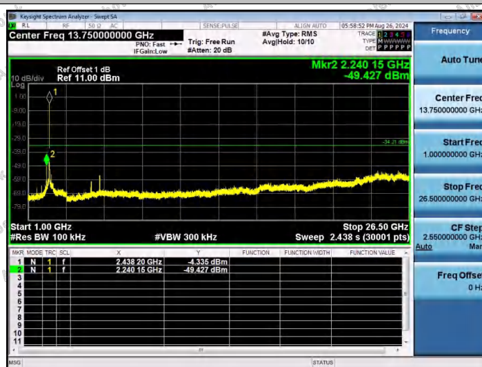
11G-Ant1-2437-1000~26500-PASS
