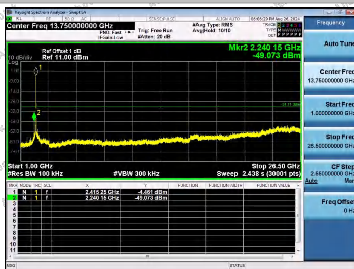
11N20SISO-Ant1-2412-1000~26500-PASS
