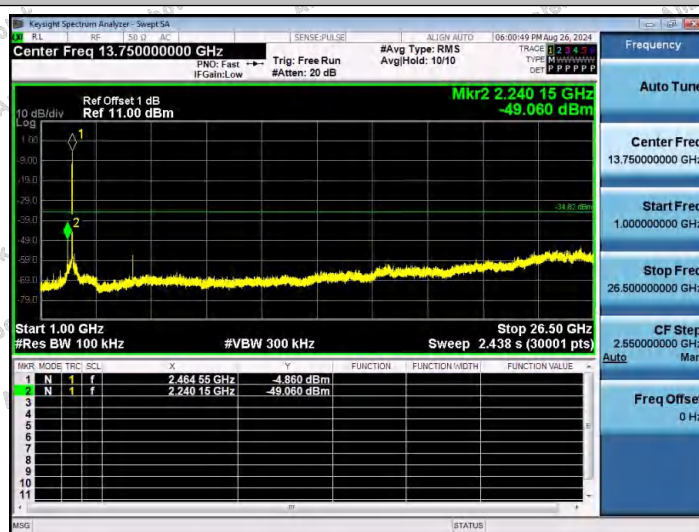
11G-Ant1-2462-1000~26500-PASS
