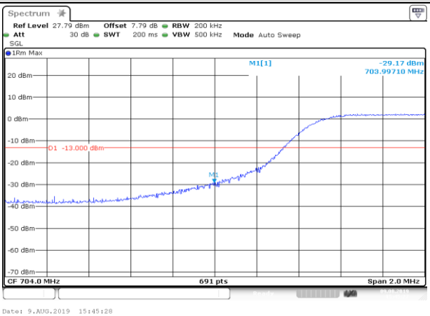
LCH_16QAM_50RB#0
