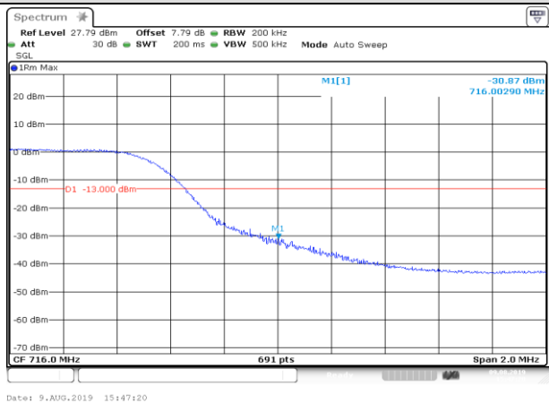
HCH_QPSK_50RB#0
