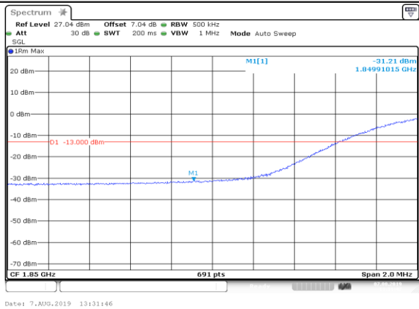
LCH_16QAM_100RB#0
