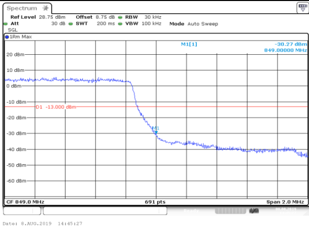
HCH_QPSK_6RB#0
