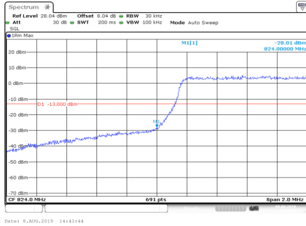
LCH_16QAM_6RB#0
