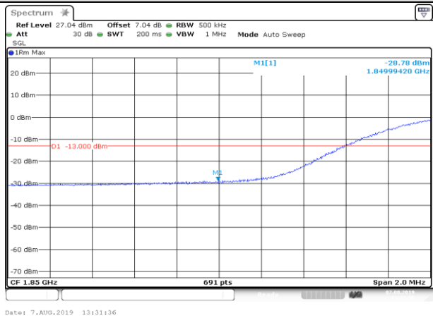
LCH_QPSK_100RB#0
