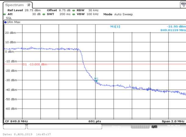
HCH_16QAM_6RB#0
