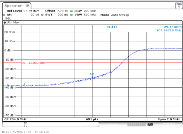
LCH_QPSK_50RB#0
