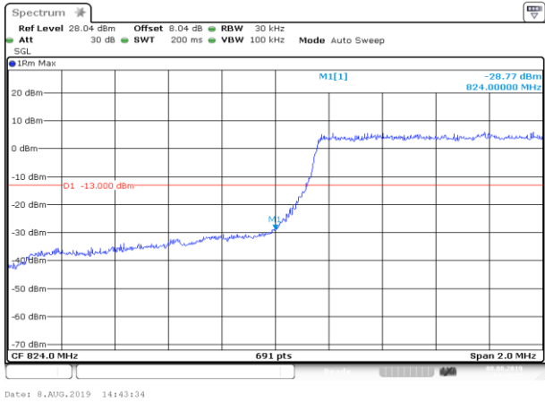
LCH_QPSK_6RB#0
