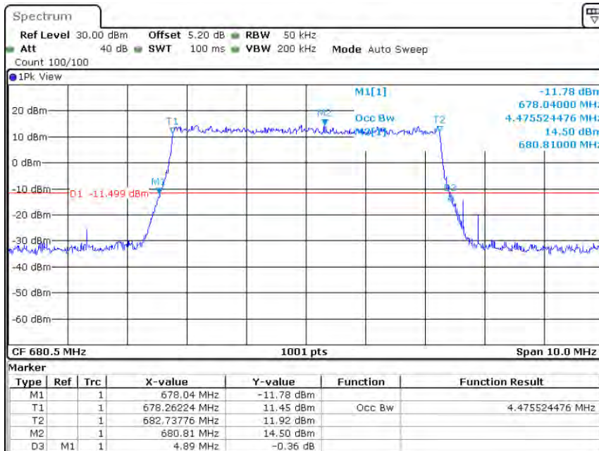
Band71-5MHz-QPSK-133297-25RB#0-4.476
