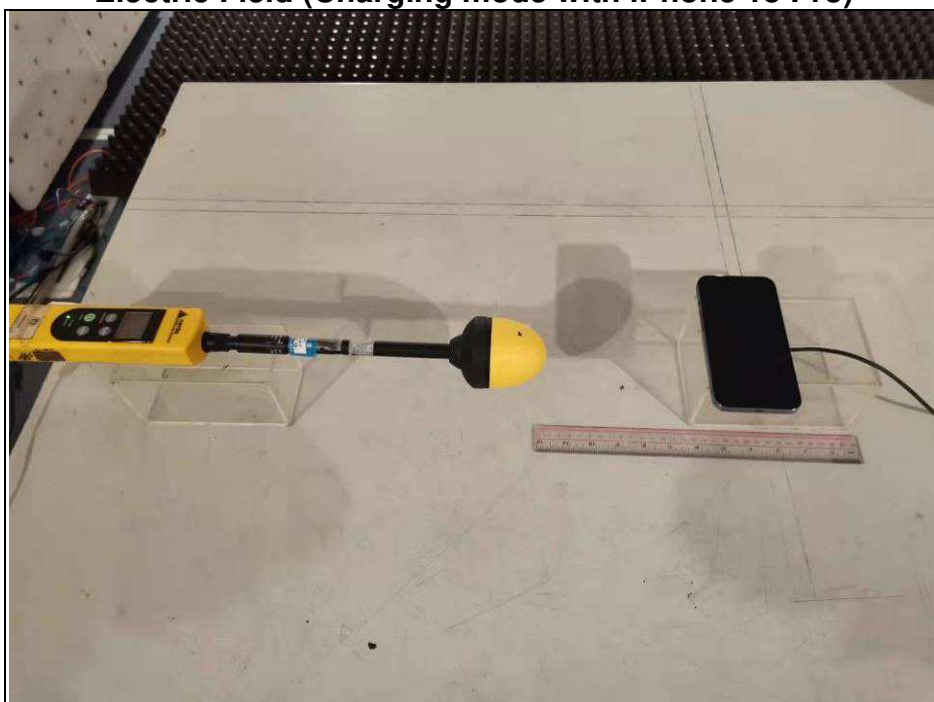
Electric Field (Charging mode with iPhone 13 Pro)
