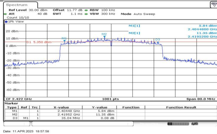
11AX40-CDD_Ant4_2422
