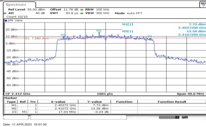
11AX20-CDD_Ant3_2412
