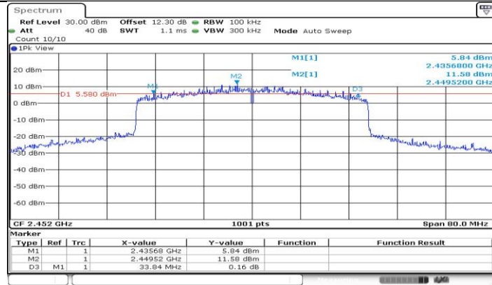
11AX40-CDD_Ant1_2452
