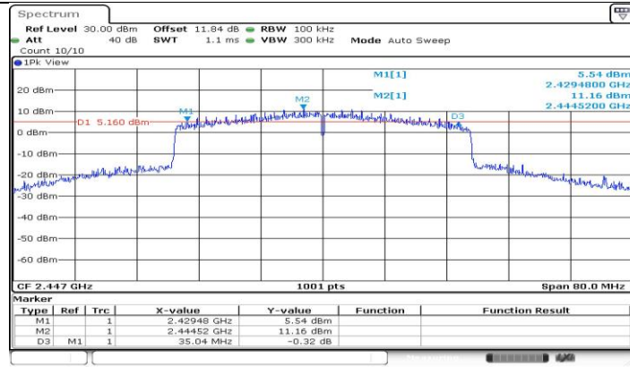
11AX40-CDD_Ant4_2447
