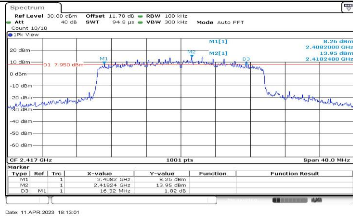
11AX20-CDD_Ant3_2417
