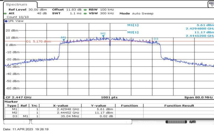
11AX40-CDD_Ant3_2447
