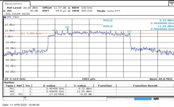
11AX20-CDD_Ant4_2412
