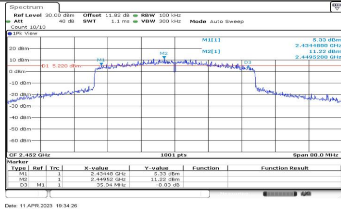
11AX40-CDD_Ant4_2452
