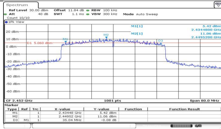
11AX40-CDD_Ant3_2452
