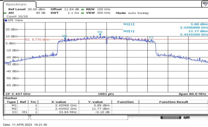
11AX40-CDD_Ant4_2437
