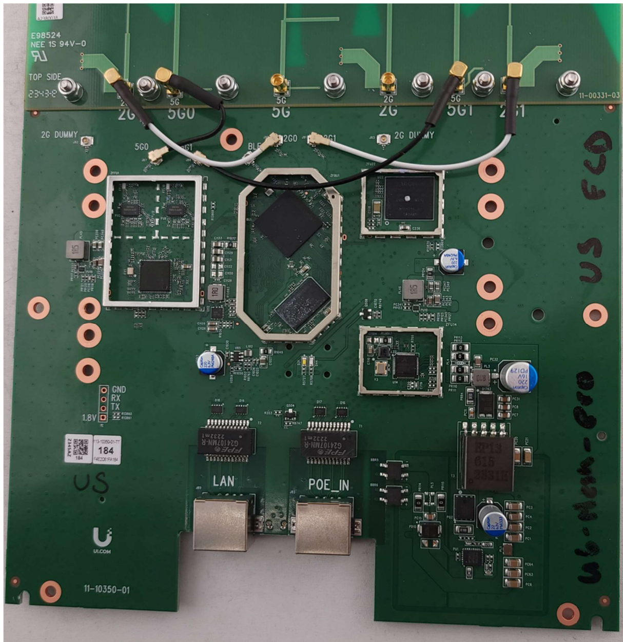
Photograph 2: Internal Front Side of PCB View With Cans Off
