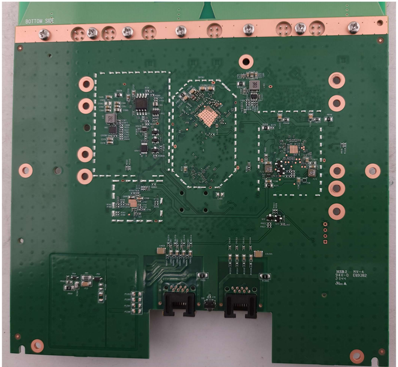
Photograph 3: Internal Back Side of PCB View
