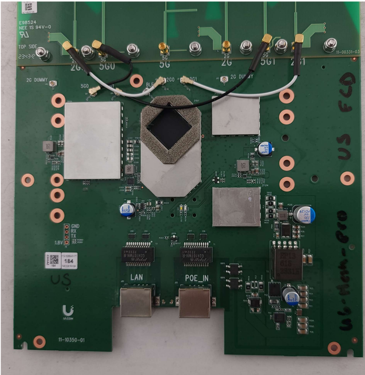
Photograph 1: Internal Front Side of PCB View With Cans On
