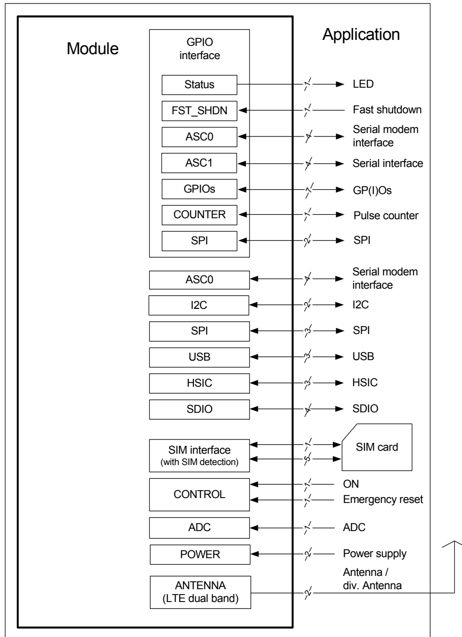
Figure 1: ELS31-US/ELS51-US system overview
