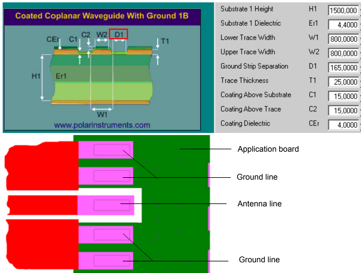
Figure 10: Micro-Stripline on 1.5mm Standard FR4 PCB - example 1
