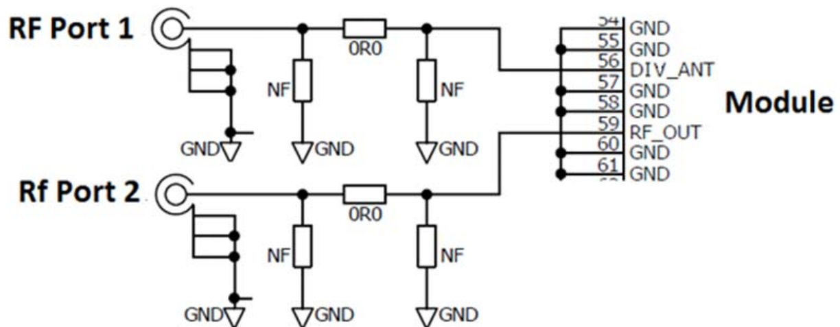
Figure 6: RF interface signals example
