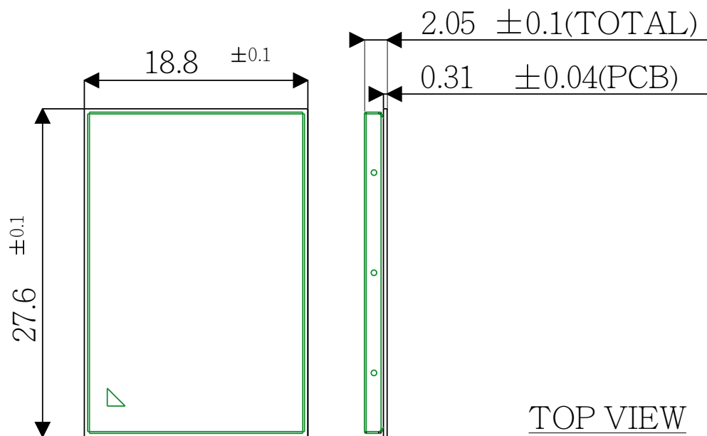
Figure 14: Dimensions of ELS31-US/ELS51-US (all dimensions in mm)
