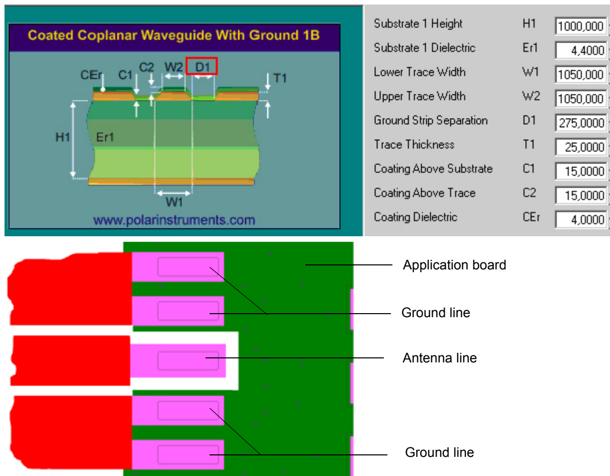
Figure 9: Micro-Stripline on 1.0mm Standard FR4 PCB - example 2
