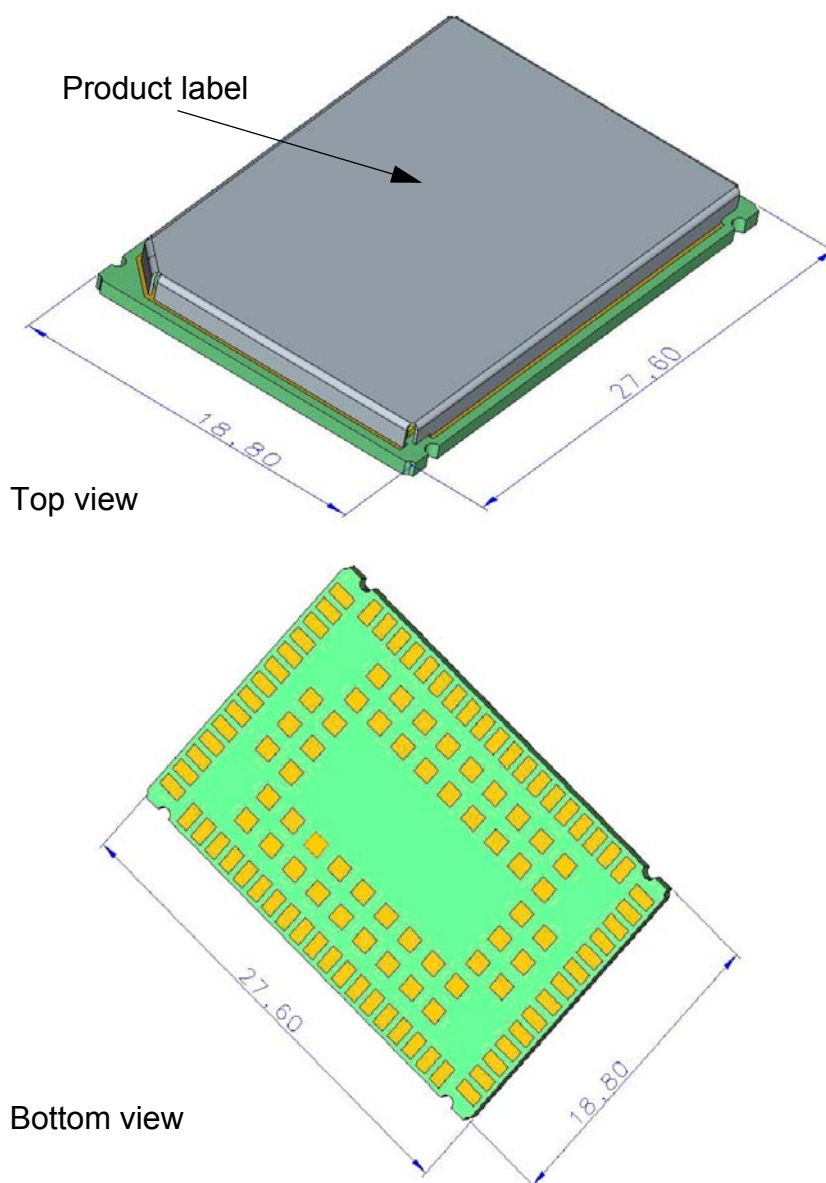
Figure 13: ELS31-US/ELS51-US– top and bottom view
