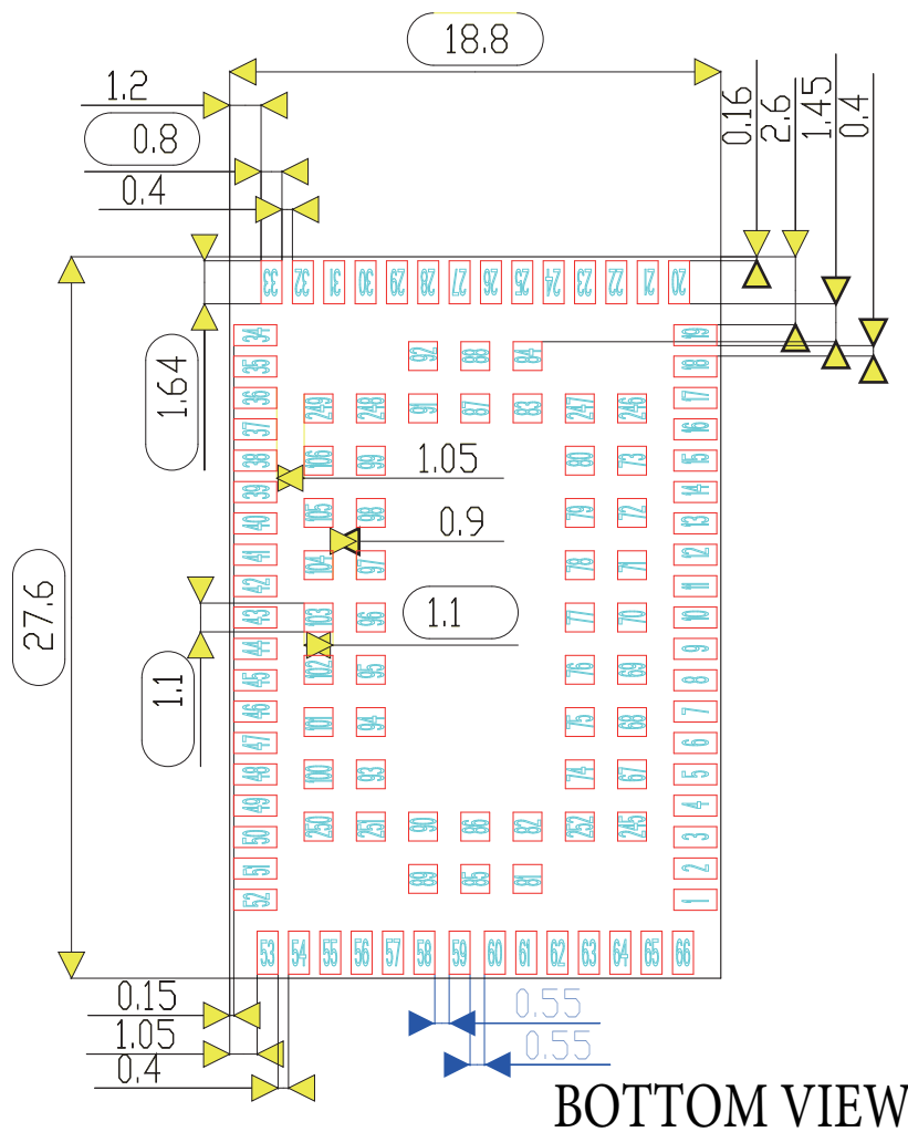
Figure 15: Dimensions of ELS31-US/ELS51-US (all dimensions in mm) - bottom view
