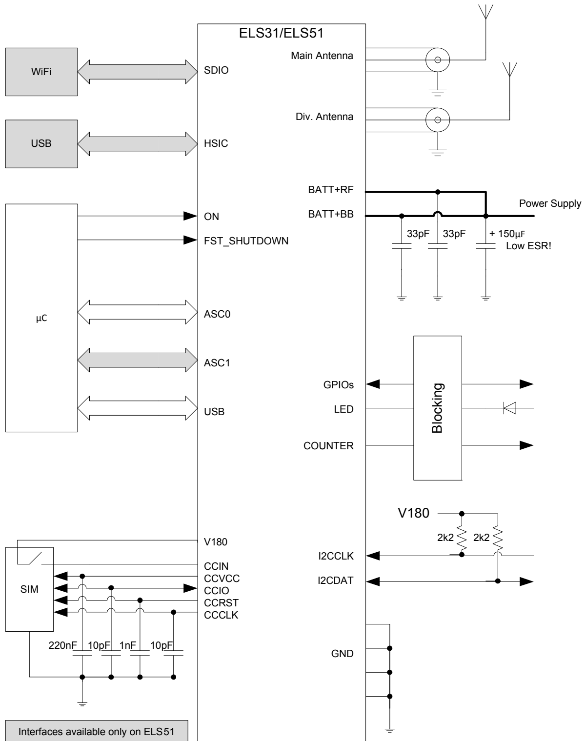
Figure 12: Schematic diagram of ELS31-US/ELS51-US sample application
