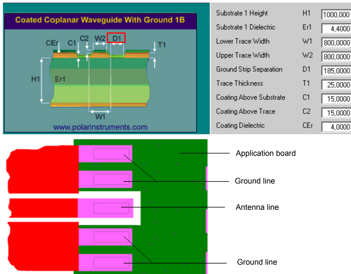
Figure 8: Micro-Stripline on 1.0mm standard FR4 2-layer PCB - example 1
