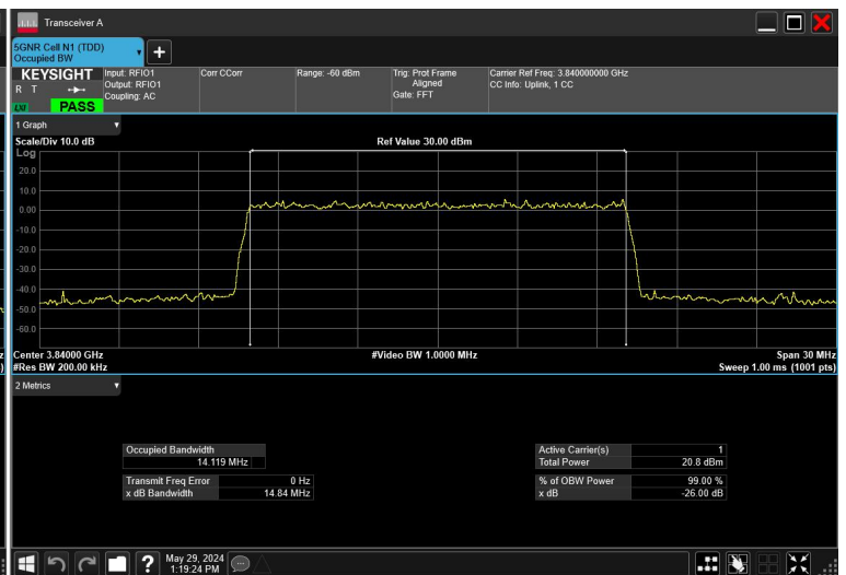
15MHz_15kHz_3840MHz_CP-OFDM 16 QAM_RB79@0
