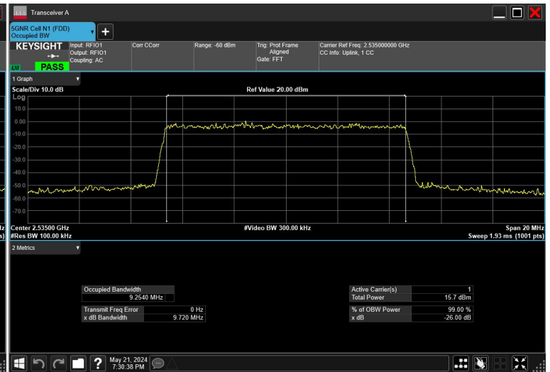
10MHz_15kHz_2535MHz_CP-OFDM 256 QAM_RB52@0
