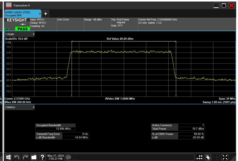
15MHz_15kHz_2535MHz_DFT-s-OFDM 16 QAM_RB75@0
