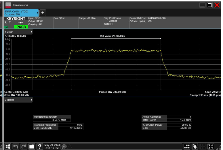
10MHz_30kHz_3840MHz_CP-OFDM 256 QAM_RB24@0
