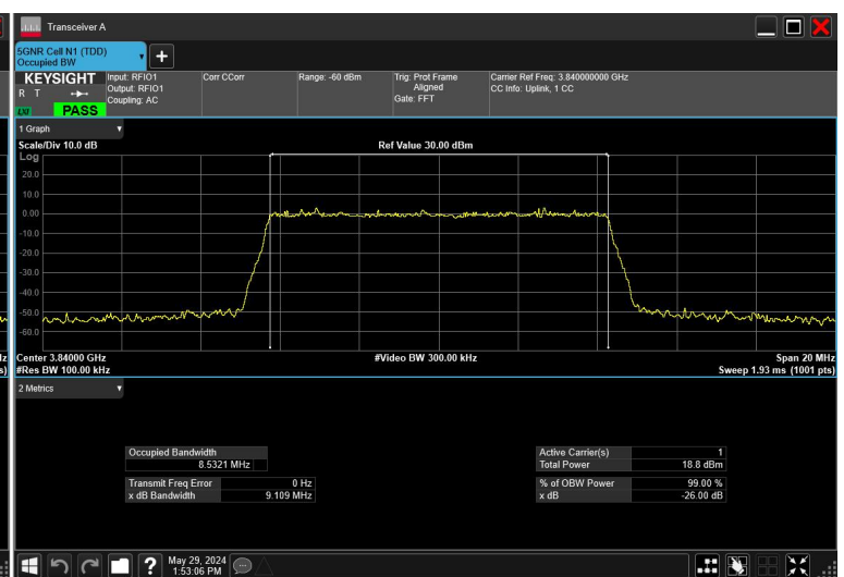
10MHz_30kHz_3840MHz_DFT-s-OFDM 256 QAM_RB24@0
