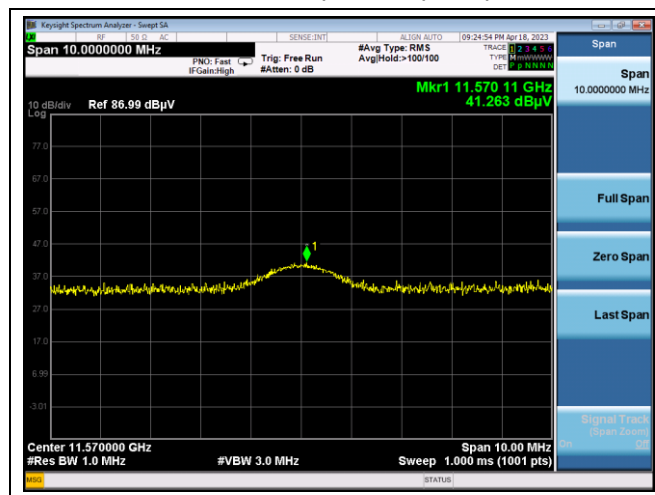
Middle channel 2 nd Spurious (Peak) - Band 3
