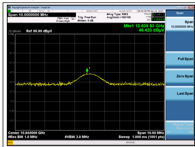
High channel 2 nd Spurious (Peak) - Band 2A
