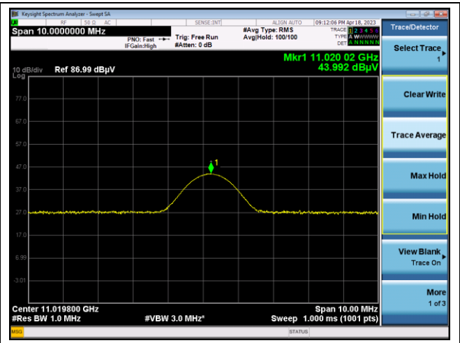
Low channel 2 nd Spurious (Average) - Band 2C
