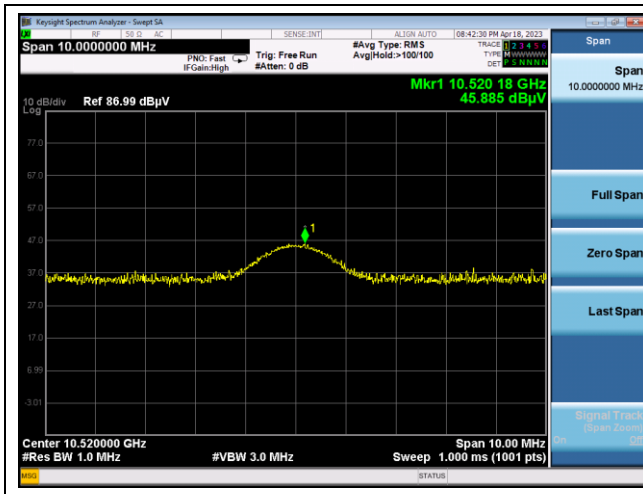
Low channel 2 nd Spurious (Peak) - Band 2A
