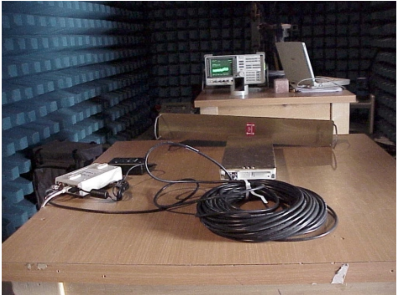
Photo #8 EUT with sector antenna. Radiated emission test
