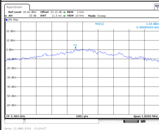
Power Density (dBm/3kHz) Plot Channel 02
