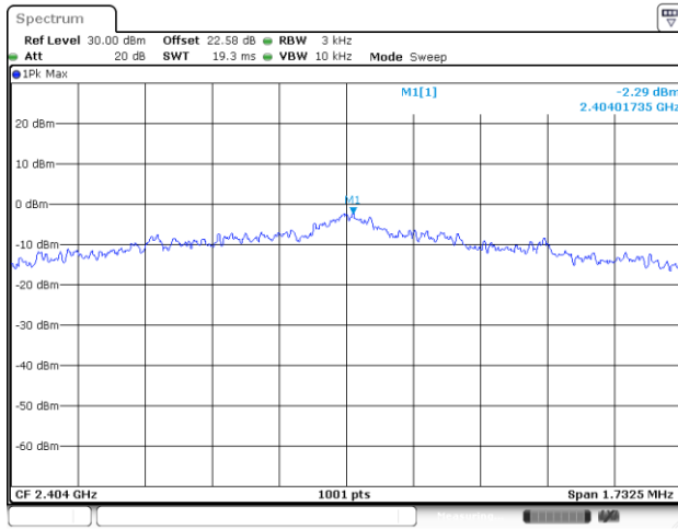
Power Density (dBm/3kHz) Plot Channel 02
