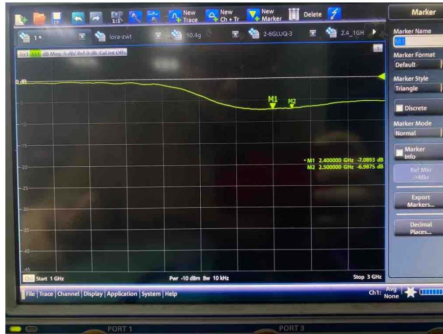
Figure 4.Return Loss
