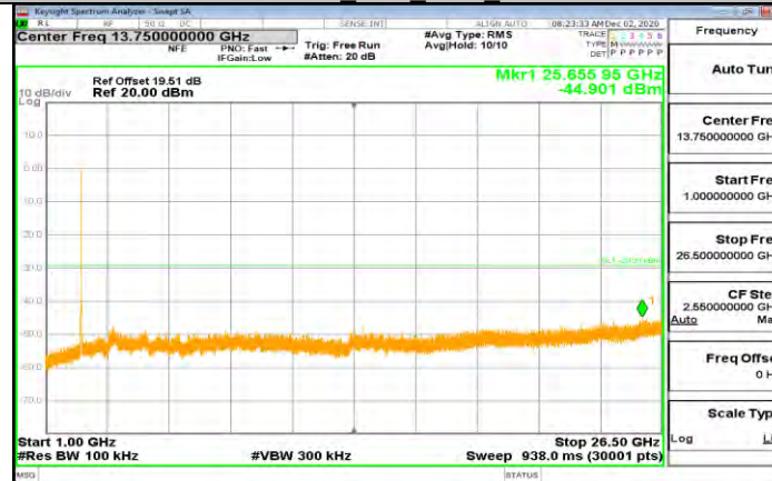
11N20SISO_Ant1_2462_1000~26500
