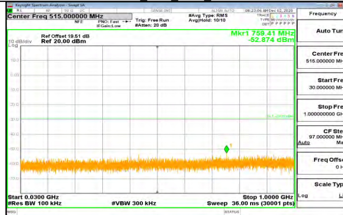
11N20SISO_Ant1_2462_30~1000
