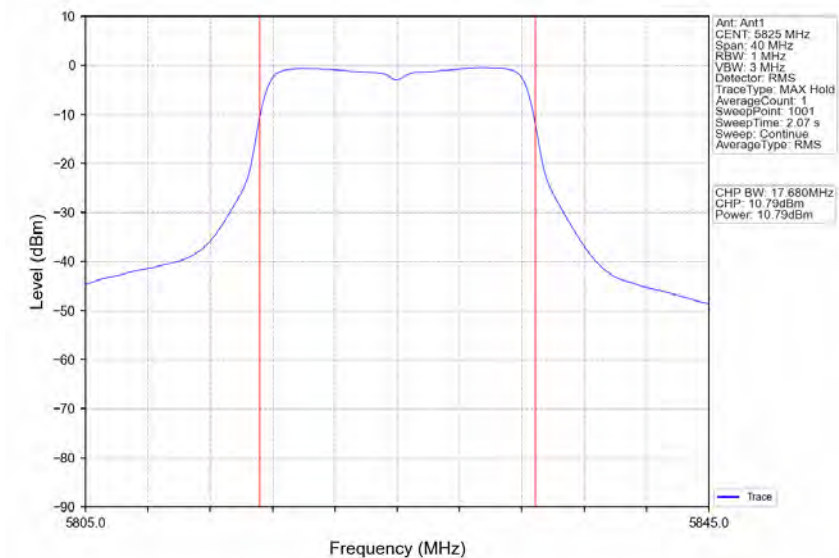
802.11a_HCH_5825MHz_Ant1_NTNV
