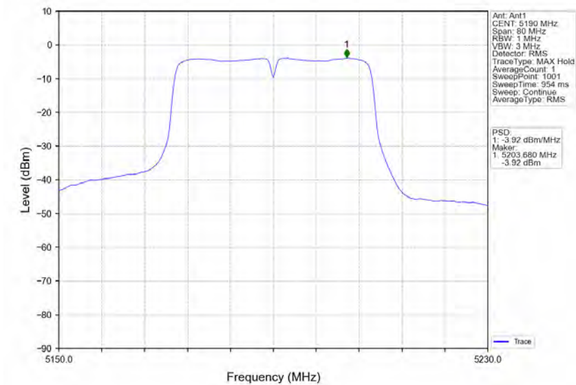
802.11ac(VHT40)_LCH_5190MHz_Ant1_NTNV
