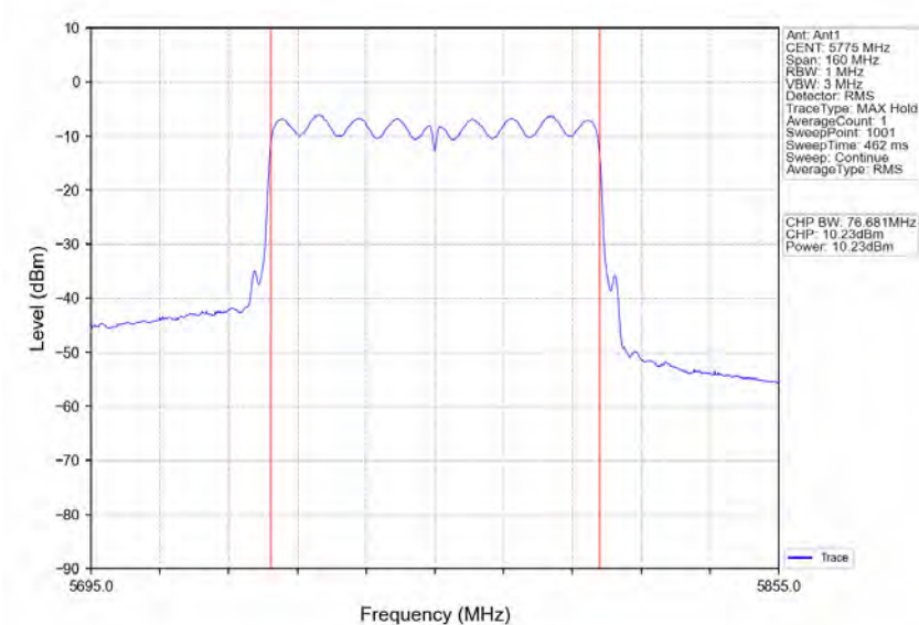
802.11ac(VHT80)_MCH_5775MHz_Ant1_NTNV
