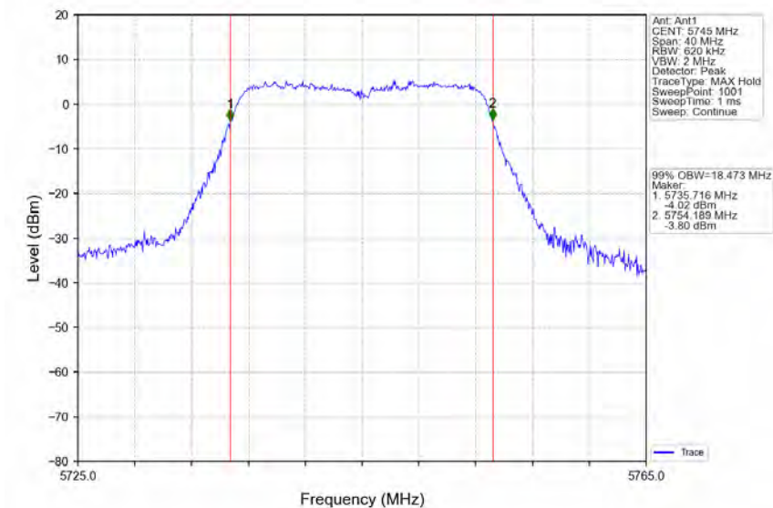
802.11ac(VHT20)_LCH_5745MHz_Ant1_NTNV
