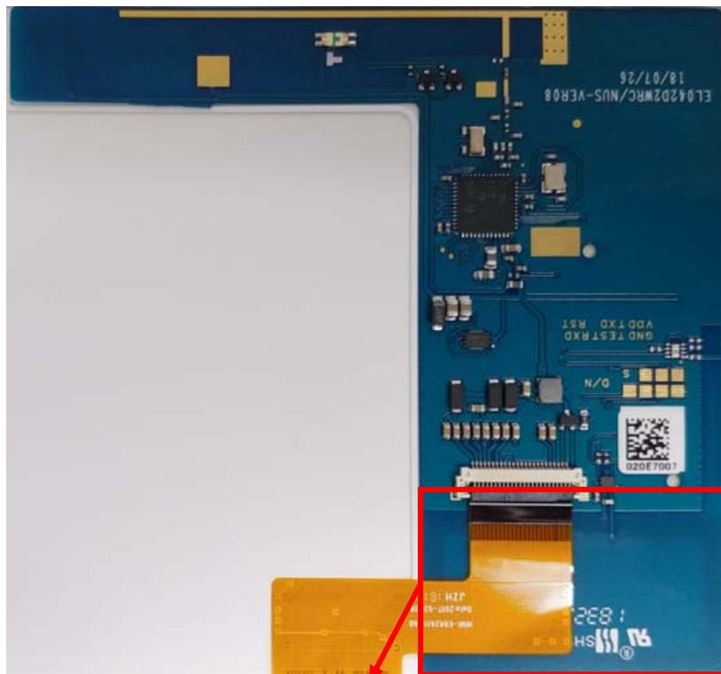
NFC receiving Antenna(RX)
