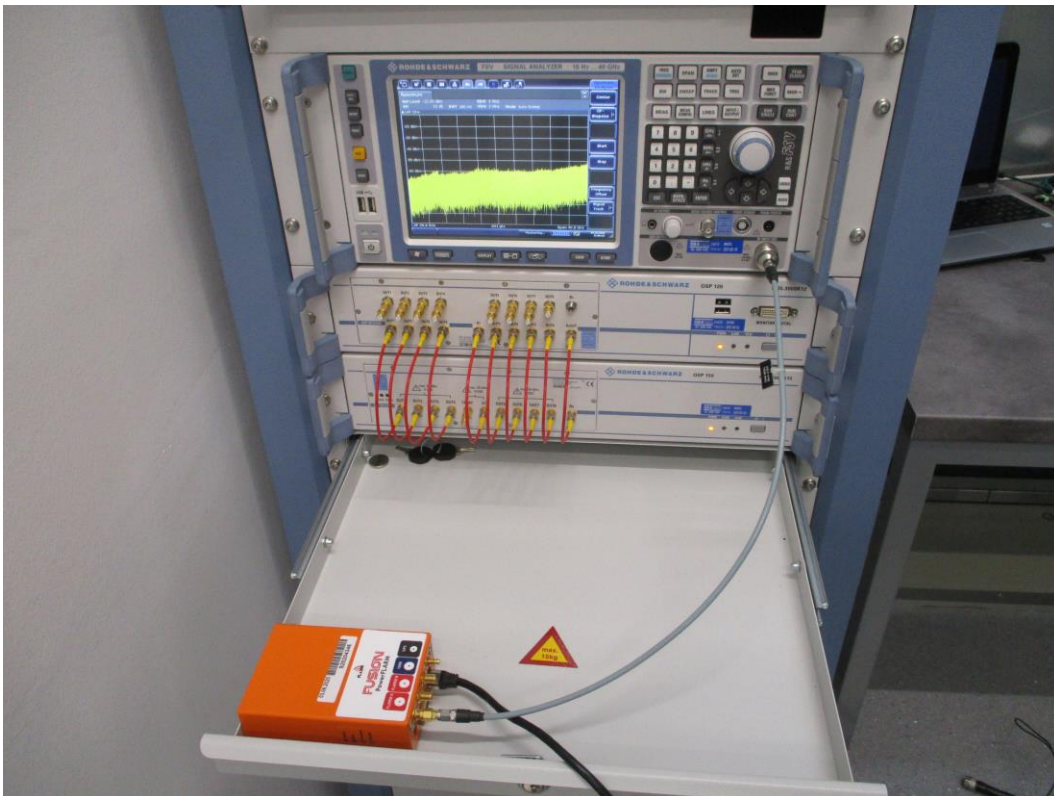
Figure 4: Conducted measurements test setup
