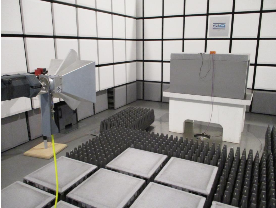
Figure 3: Spurious emission 1-10 GHz
