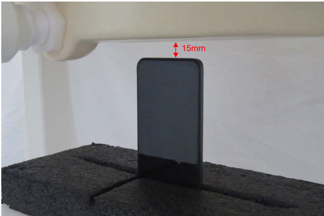
Picture 8: Bottom Edge, the distance from handset to the bottom of the Phantom is 15mm
