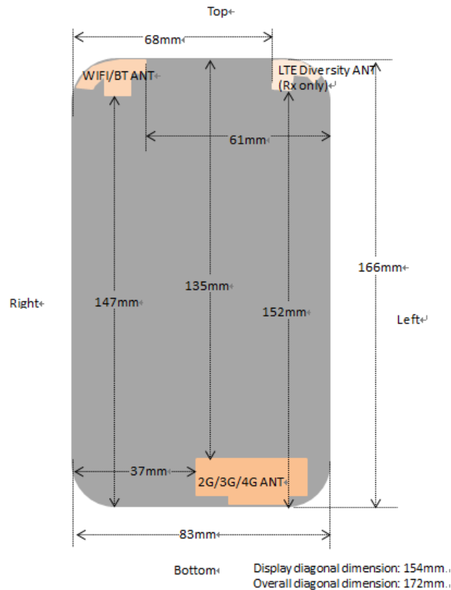
Fig.14.1 EUT Antenna Locations
