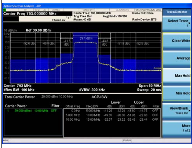
LTE Band 14 QPSK 100%RB 10MHz CH Middle
