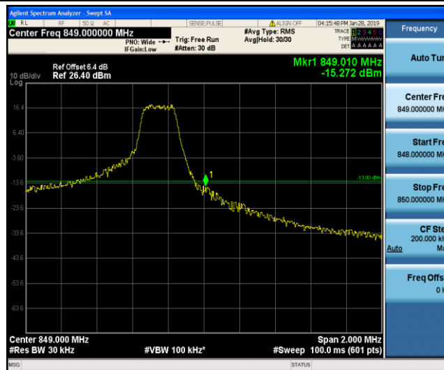
Band5_1.4MHz_QPSK_20643_1RB#5
