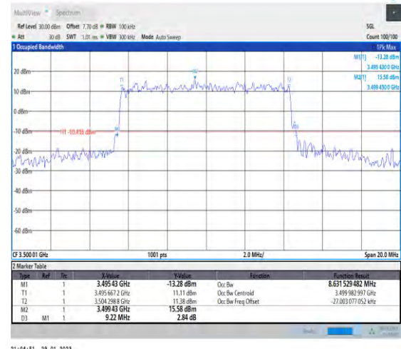
1-N78-3450-3550-30-10-M-1-DFT-QPSK-Outer_Full- 24@0-Ant1-8.632-9.220-≤10-PASS
