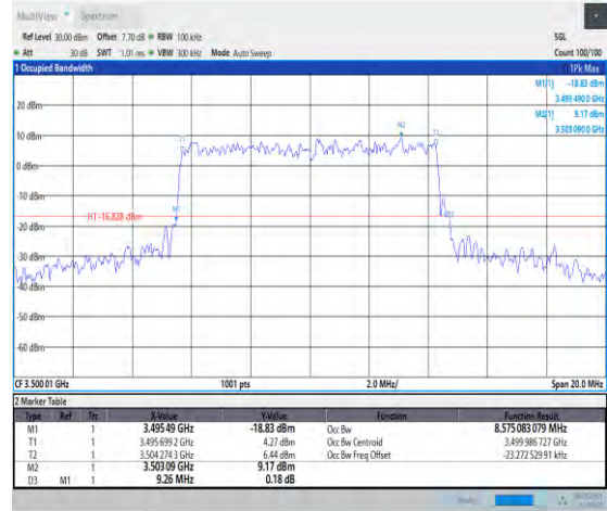
1-N78-3450-3550-30-10-M-9-CP-256QAM-Outer_Ful I-24@0-Ant1-8.575-9.260-≤10-PASS
