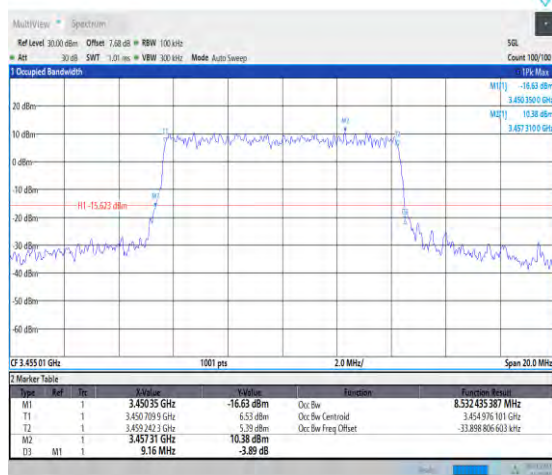
1-N78-3450-3550-30-10-L-5-DFT-256QAM-Outer_Full-24@0-Ant1-8.532-9.160-≤10-PASS
