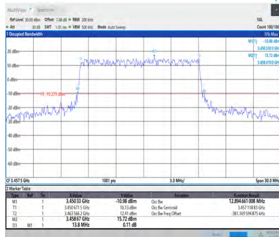
1-N78-3450-3550-30-15-L-3-DFT-16QAM-Outer_Full-36@0-Ant1-12.895-13.800-≤15-PASS
