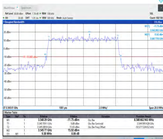
1-N78-3450-3550-30-10-H-1-DFT-QPSK-Outer_Full- 24@0-Ant1-8.581-9.380-≤10-PASS
