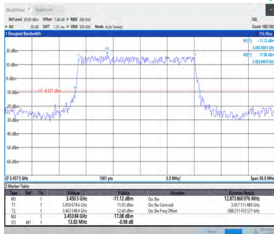
1-N78-3450-3550-30-15-L-2-DFT-PI2BPSK-Outer_Full-36@0-Ant1-12.874-13.830-≤15-PASS
