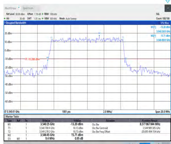
1-N78-3450-3550-30-10-H-2-DFT-PI2BPSK-Outer_F ull-24@0-Ant1-8.578-9.400-≤10-PASS
