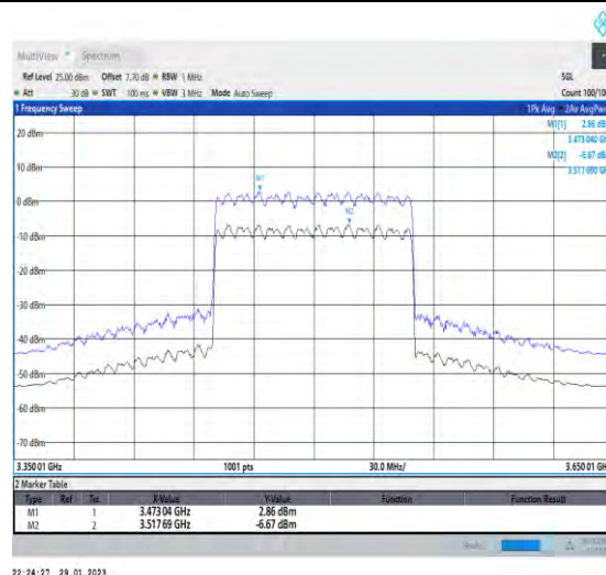
1-N78-3450-3550-30-100-M-2-CP-256QAM-Outer_Full-273@0-Ant1-9.53-100%-0.00-9.53-PASS-≤13
