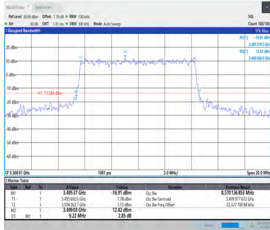
1-N78-3450-3550-30-10-M-8-CP-64QAM-Outer_Full -24@0-Ant1-8.57-9.220-≤10-PASS
