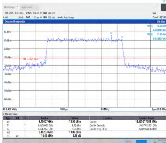
1-N78-3450-3550-30-15-L-6-CP-QPSK-Outer_Full-38@0-Ant1-13.625-14.490-≤15-PASS
