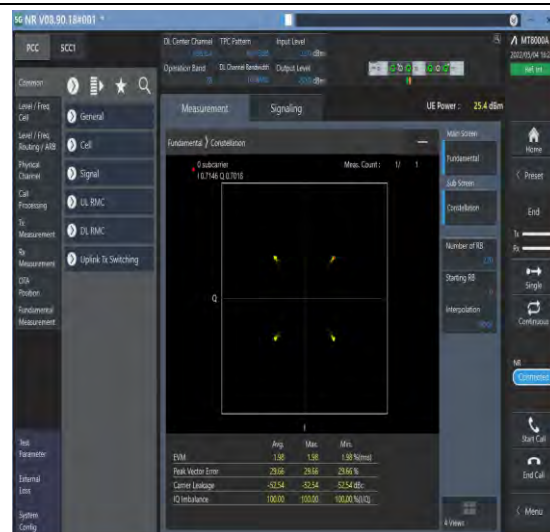
1-N78-3450-3550--30-100-M-2-DFT-QPSK-Outter_Full-270@0-Ant1-see graph-PASS
