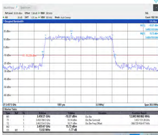
1-N78-3450-3550-30-15-L-4-DFT-64QAM-Outer_Full-36@0-Ant1-12.846-13.920-≤15-PASS
