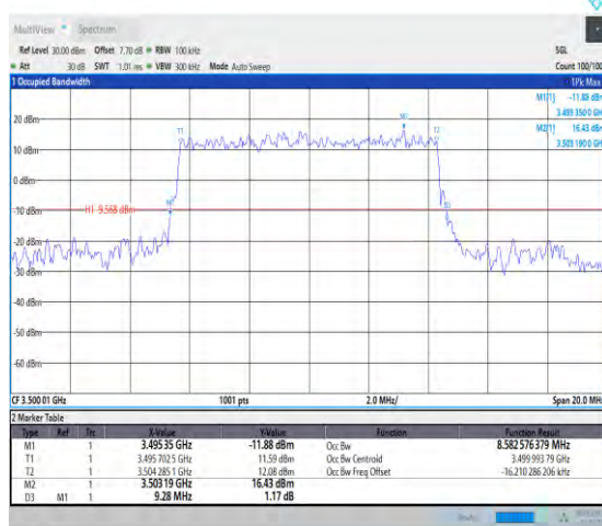
1-N78-3450-3550-30-10-M-2-DFT-PI2BPSK-Outer_ Full-24@0-Ant1-8.583-9.280-≤10-PASS
