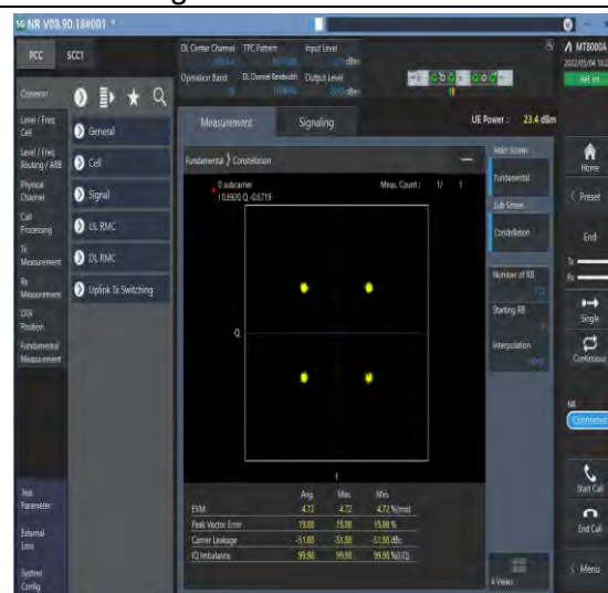
1-N78-3450-3550--30-100-M-6-CP-QPSK-Outer_Full-273@0-Ant1-see graph-PASS
