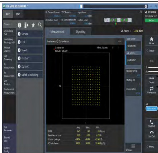
1-N78-3450-3550--30-100-M-5-DFT-256QAM-Outer_Full-270@0-Ant1-see graph-PASS
