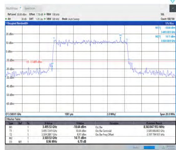
1-N78-3450-3550-30-10-M-3-DFT-16QAM-Outer_Ful I-24@0-Ant1-8.564-8.960-≤10-PASS
