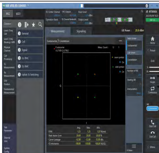
1-N78-3450-3550--30-100-M-1-DFT-PI2BPSK-Outter_Full-270@0-Ant1-see graph-PASS
