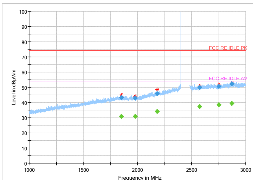
Fig.56 Radiated emission: 8DPSK, Ch0, 1GHz~3GHz
