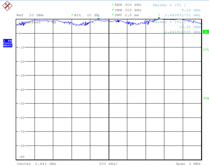
Fig.89 Carrier separation measurement: 8DPSK, Ch39
