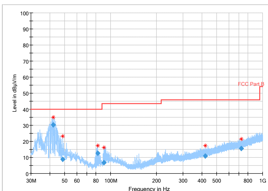
Fig.55 Radiated emission: 8DPSK, Ch0, 30MHz~1GHz
