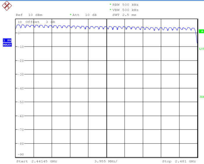
Fig.95 Number of hopping frequency: 8DPSK, Ch40~78
