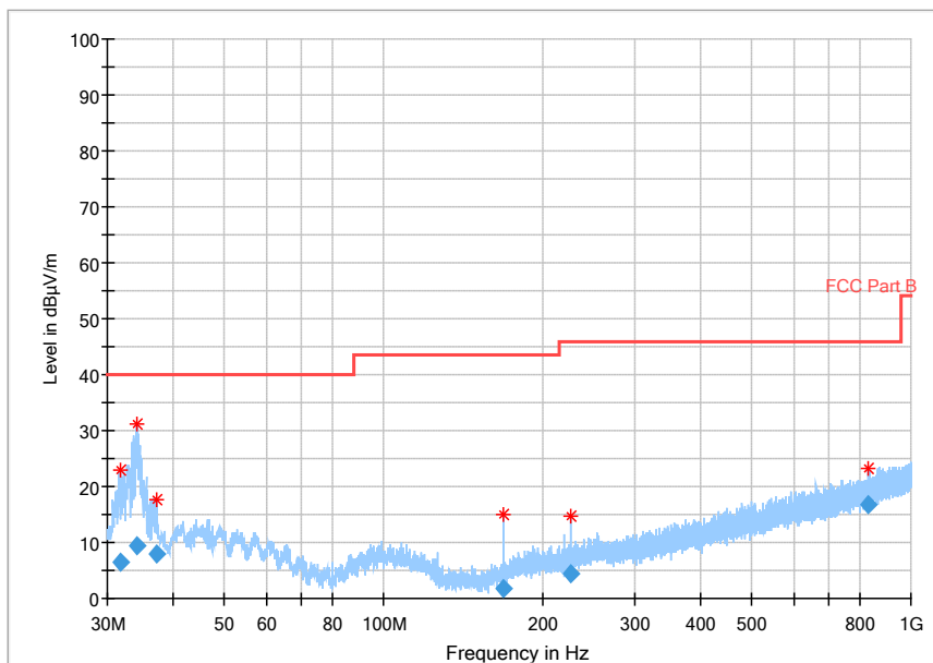
Fig.45 Radiated emission: GFSK, Ch0, 30MHz~1GHz
