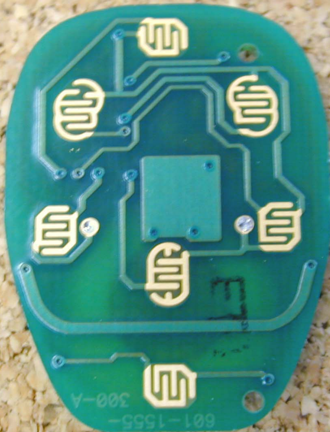
GM04 TX - Bottom (No Battery) - Murata SAW
