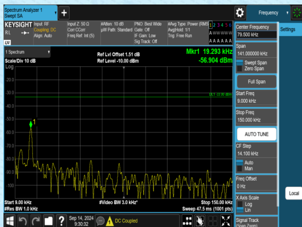
Band5-1.4MHz-QPSK-20643-1RB#0-0.009~0.15-PASS
