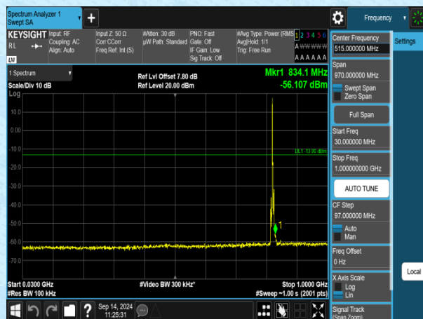
Band5-3MHz-QPSK-20415-1RB#0-30~1000-PASS
