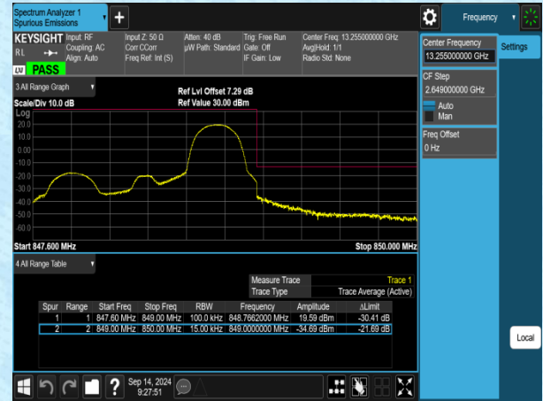
Band5-1.4MHz-16QAM-20643-1RB#5-PASS
