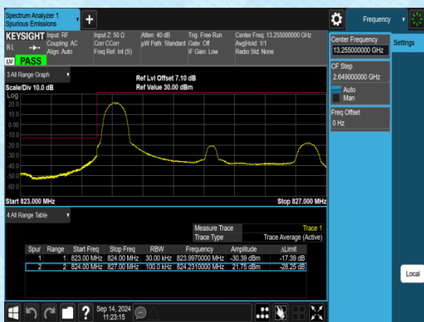
Band5-3MHz-QPSK-20415-1RB#0-PASS
