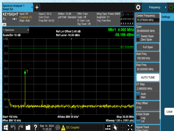
Band5-3MHz-QPSK-20415-1RB#0-0.15~30-PASS
