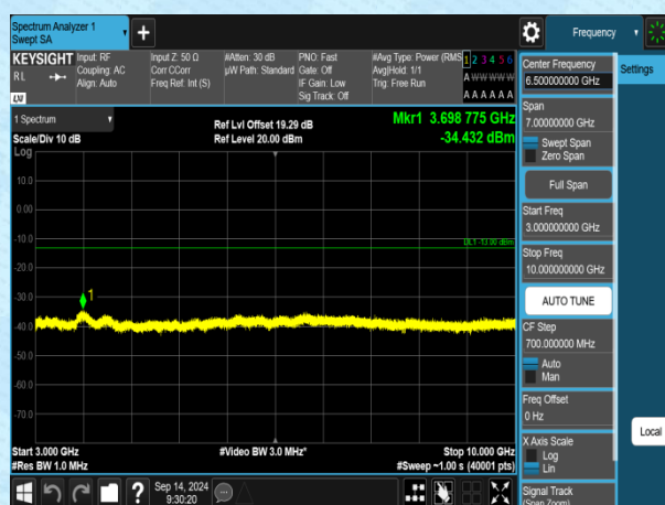
Band5-1.4MHz-QPSK-20525-1RB#0-3000~10000-PASS
