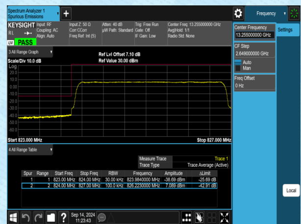
Band5-3MHz-QPSK-20415-15RB#0-PASS
