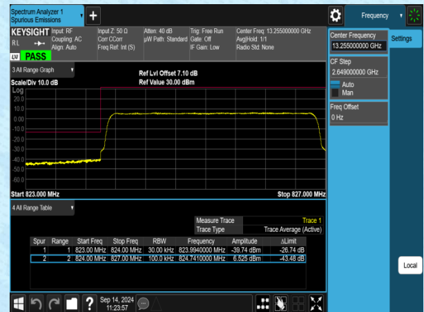
Band5-3MHz-16QAM-20415-15RB#0-PASS
