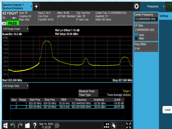
Band5-3MHz-16QAM-20415-1RB#0-PASS
