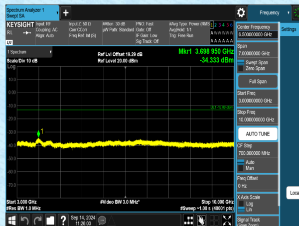
Band5-3MHz-QPSK-20415-1RB#0-3000~10000-PASS
