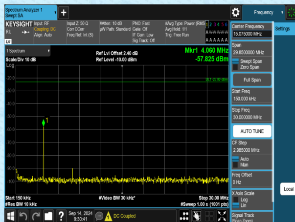
Band5-1.4MHz-QPSK-20643-1RB#0-0.15~30-PASS
