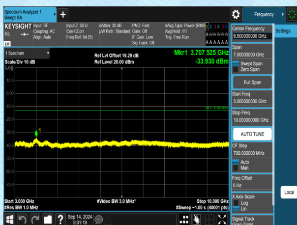
Band5-1.4MHz-QPSK-20643-1RB#0-3000~10000-PASS
