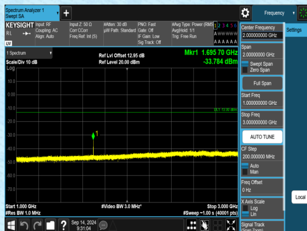
Band5-1.4MHz-QPSK-20643-1RB#0-1000~3000-PASS
