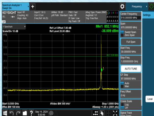
Band5-1.4MHz-QPSK-20643-1RB#0-30~1000-PASS
