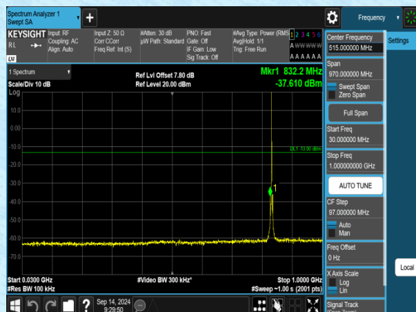
Band5-1.4MHz-QPSK-20525-1RB#0-30~1000-PASS
