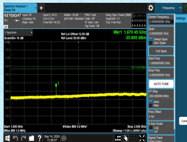
Band5-3MHz-QPSK-20525-1RB#0-1000~3000-PASS
