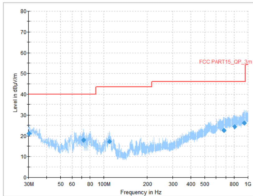
Fig.50 Radiated Spurious Emission (All Channels, 30MHz-1 GHz)
