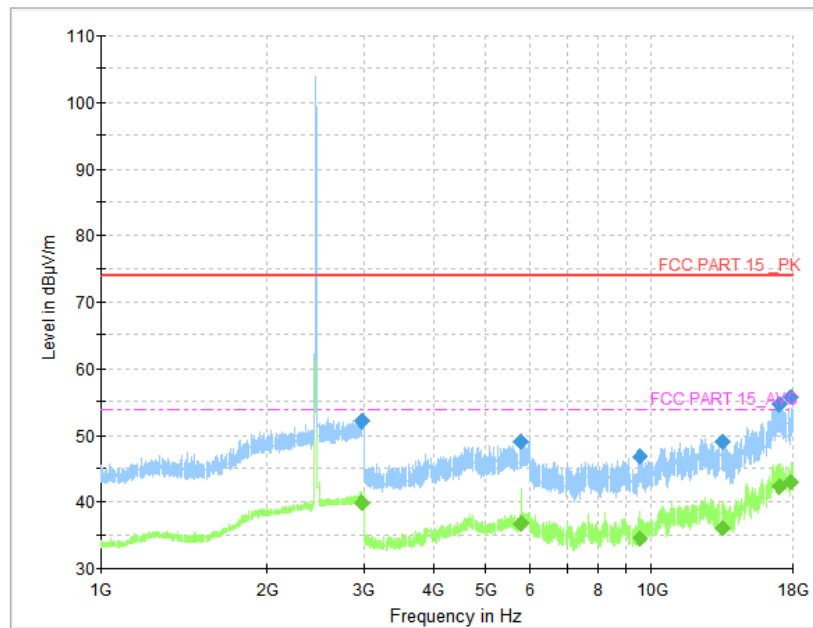
Fig.36 Radiated Spurious Emission (802.11b, CH11, 1 GHz-18GHz)
