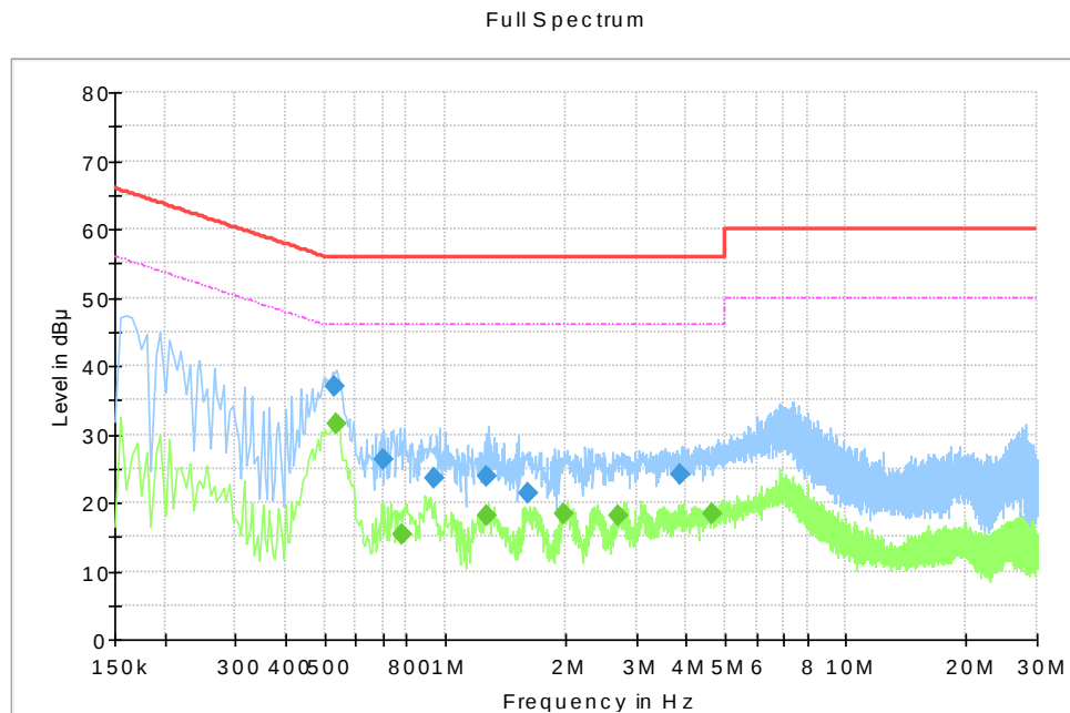
Fig.53 AC Power line Conducted Emission (Idle)
