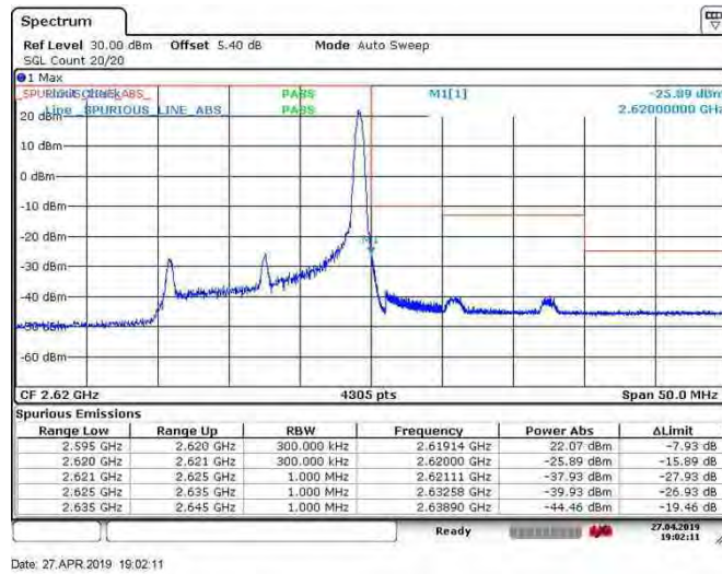
BAND38_15MHz_16QAM_38175_75RB#0
