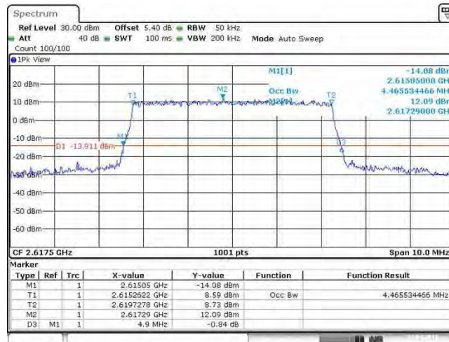
Band38_5MHz_64QAM_38225_25RB#0
