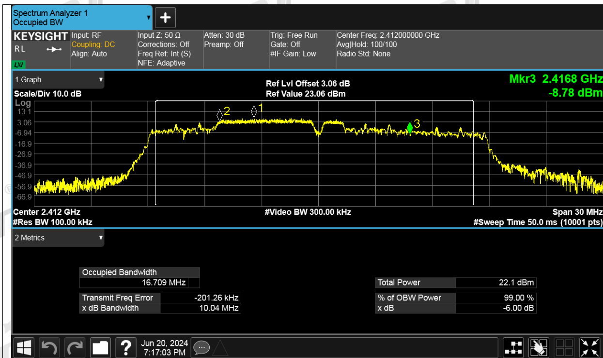
-6dB Bandwidth NVNT be20 52+26RU Index 38+1 2412MHz Ant2
