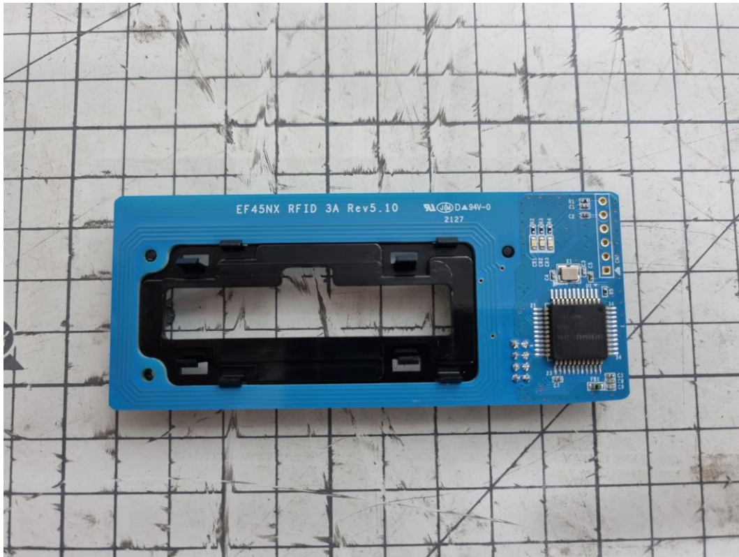
RFID Antenna Board
