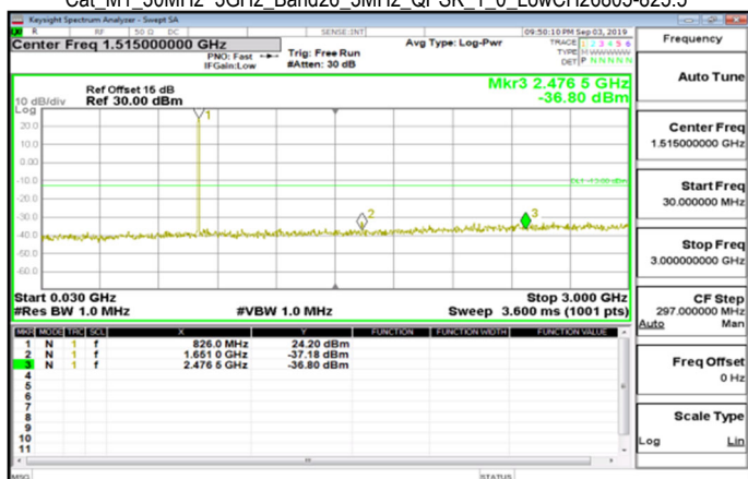
Cat_M1_30MHz~3GHz_Band26_3MHz_QPSK_1_0_LowCH26805-825.5
