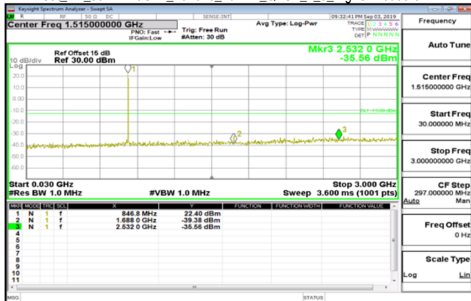
Cat_M1_30MHz~3GHz_Band26_10MHz_QPSK_1_0_HighCH26990-844
