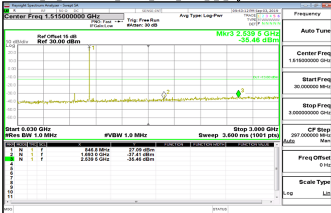
Cat_M1_30MHz~3GHz_Band26_5MHz_QPSK_1_0_HighCH27015-846.5
