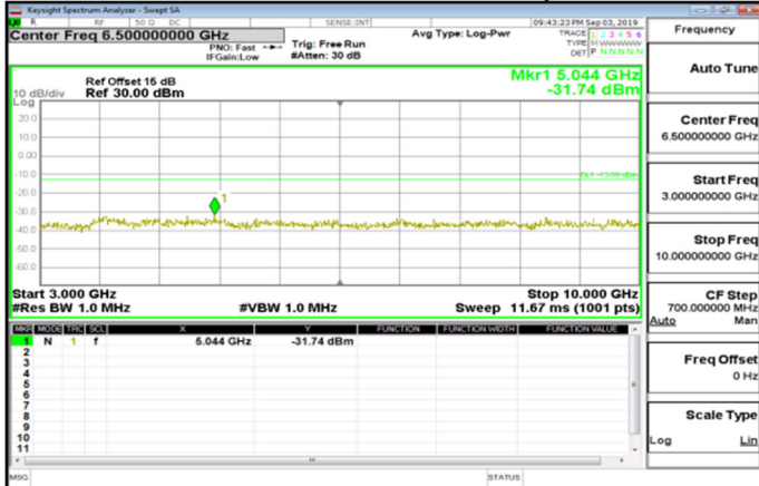
Cat_M1_3GHz~10GHz_Band26_5MHz_QPSK_1_0_HighCH27015-846.5
