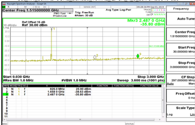
Cat_M1_30MHz~3GHz_Band26_10MHz_QPSK_1_0_LowCH26840-829
