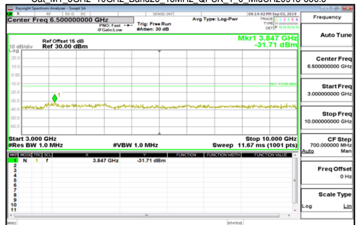
Cat_M1_3GHz~10GHz_Band26_15MHz_QPSK_1_0_MidCH26915-836.5
