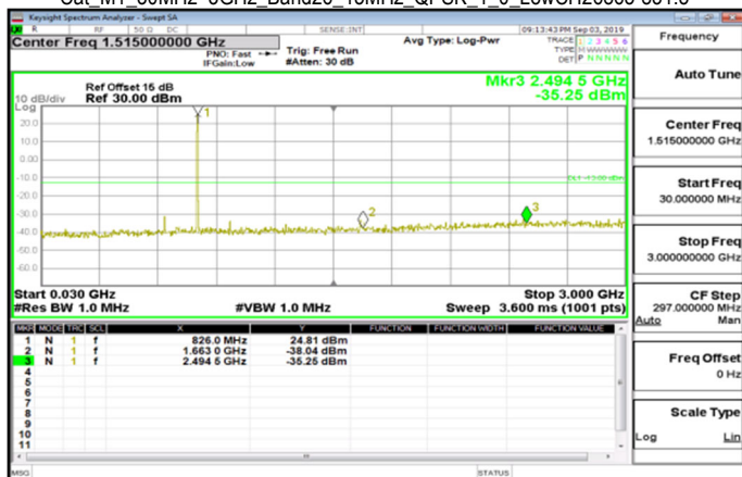
Cat_M1_30MHz~3GHz_Band26_15MHz_QPSK_1_0_LowCH26865-831.5
