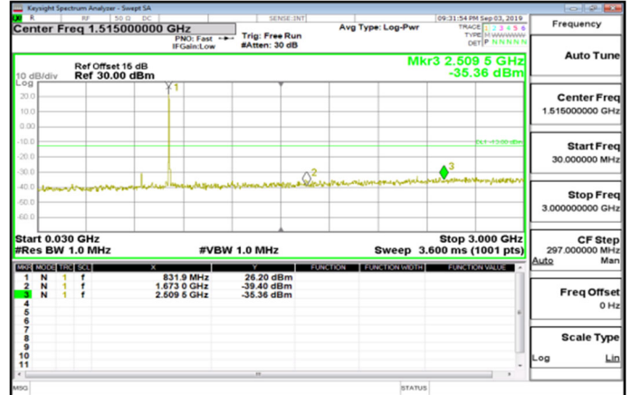
Cat_M1_30MHz~3GHz_Band26_10MHz_QPSK_1_0_MidCH26915-836.5
