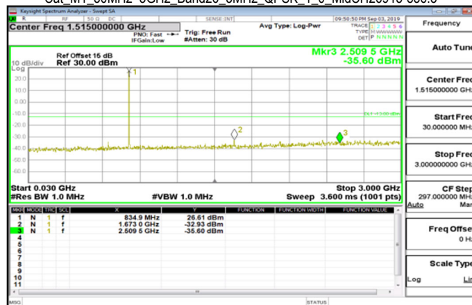
Cat_M1_30MHz~3GHz_Band26_3MHz_QPSK_1_0_MidCH26915-836.5
