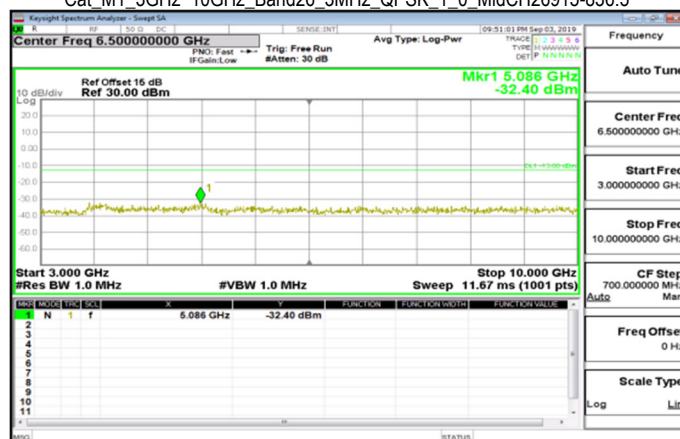
Cat_M1_3GHz~10GHz_Band26_3MHz_QPSK_1_0_MidCH26915-836.5
