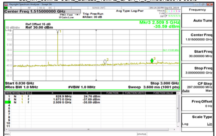
Cat_M1_30MHz~3GHz_Band26_15MHz_QPSK_1_0_MidCH26915-836.5
