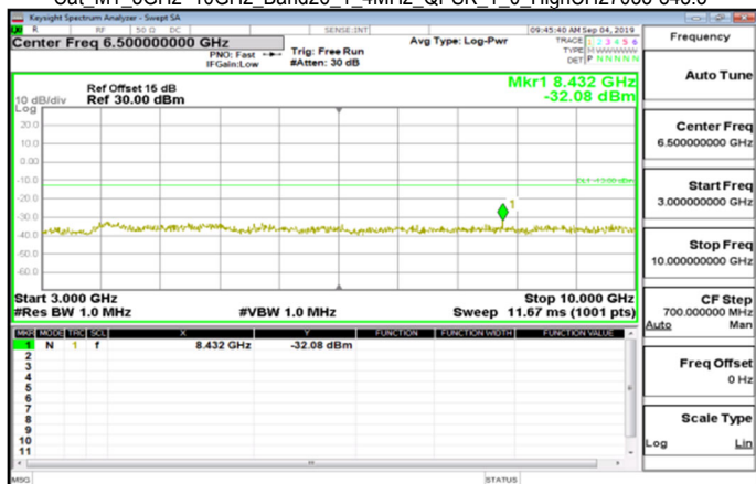
Cat_M1_3GHz~10GHz_Band26_1_4MHz_QPSK_1_0_HighCH27033-848.3
