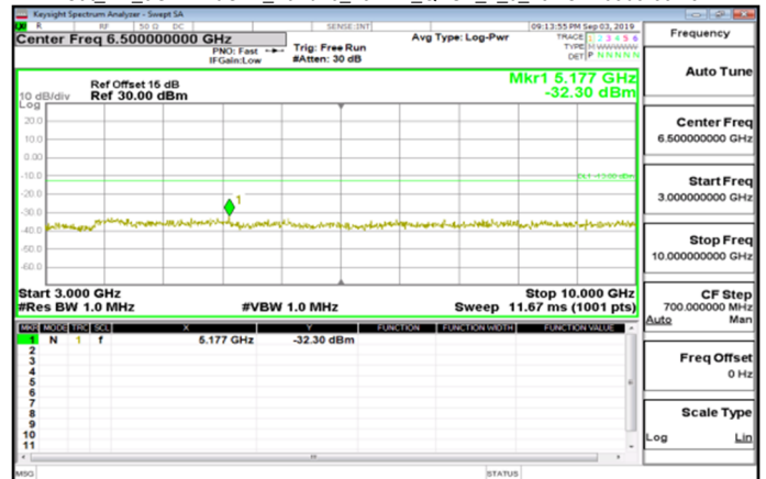
Cat_M1_3GHz~10GHz_Band26_15MHz_QPSK_1_0_LowCH26865-831.5
