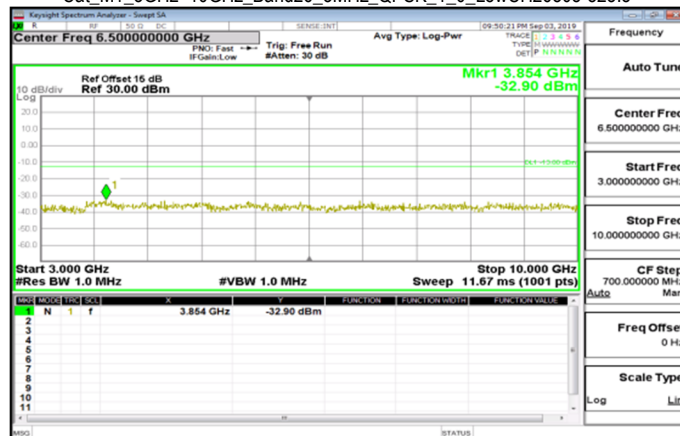
Cat_M1_3GHz~10GHz_Band26_3MHz_QPSK_1_0_LowCH26805-825.5
