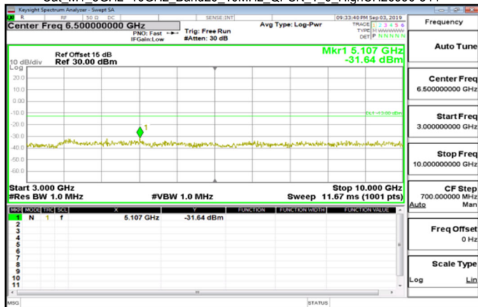
Cat_M1_3GHz~10GHz_Band26_10MHz_QPSK_1_0_HighCH26990-844
