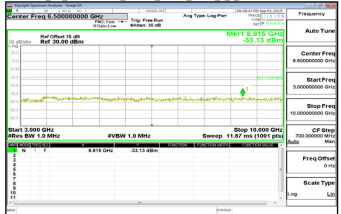
Cat_M1_3GHz~10GHz_Band26_10MHz_QPSK_1_0_LowCH26840-829
