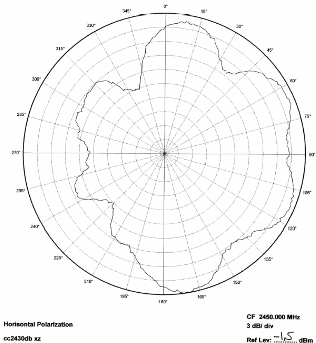
Figure 6. XZ Plane Horizontal Polarization
