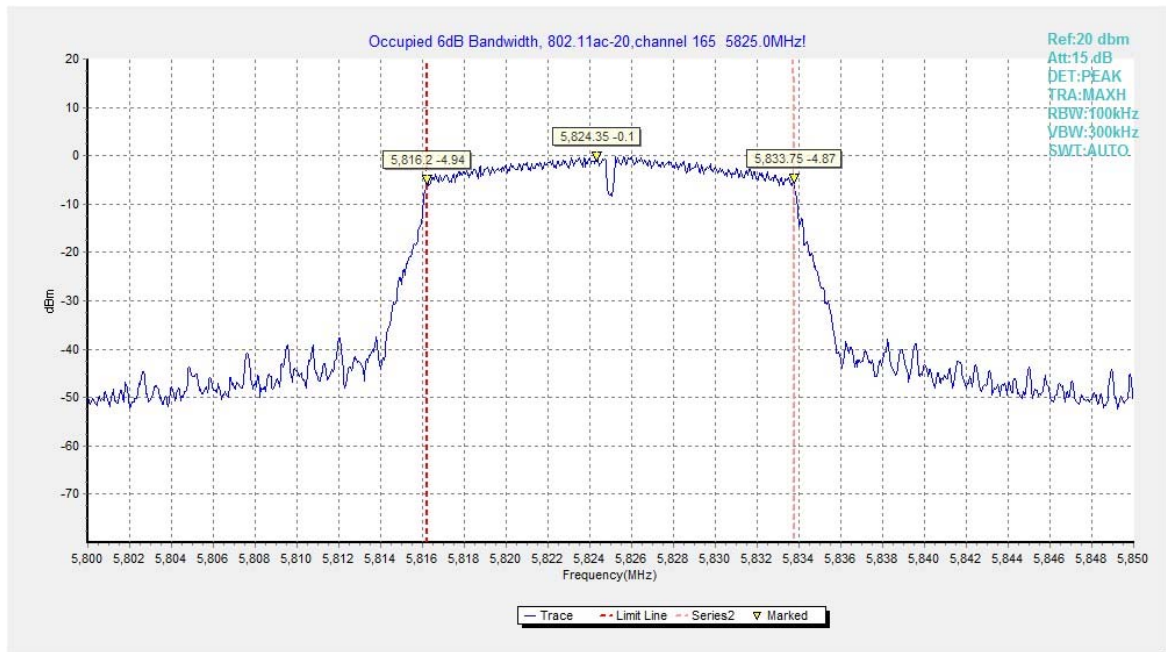
Fig. 6 Occupied 6dB Bandwidth (802.11ac-HT20, Ch 165)
