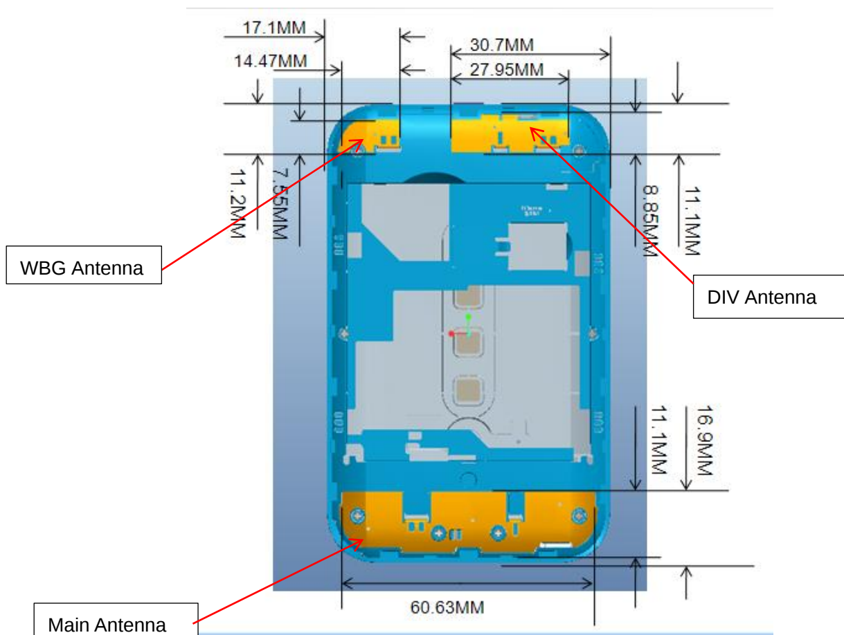
Picture 12.1 Antenna Locations (Back View)
