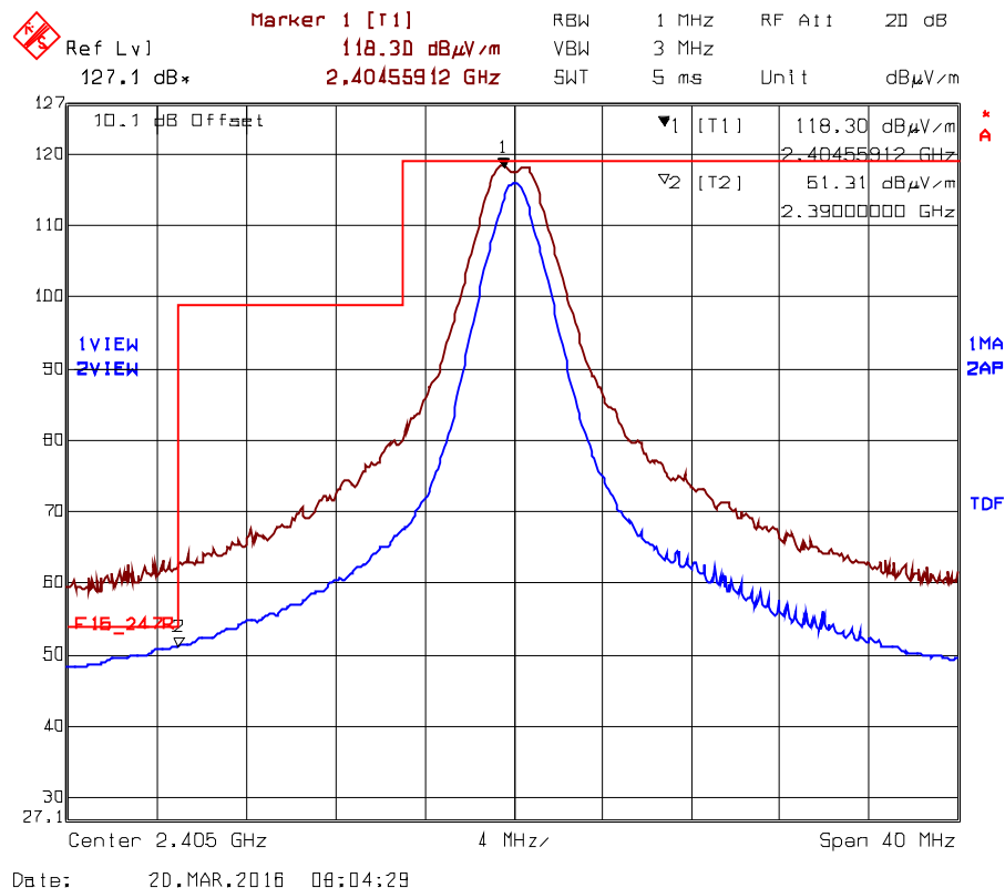
Plot 5.2.4.4.2.1. Band-Edge RF Radiated Emissions at 3 m, Horizontal Polarization Low End of Frequency Band, Ch11- 2405 MHz, QPSK Modulation, Power 8 Mode 1
