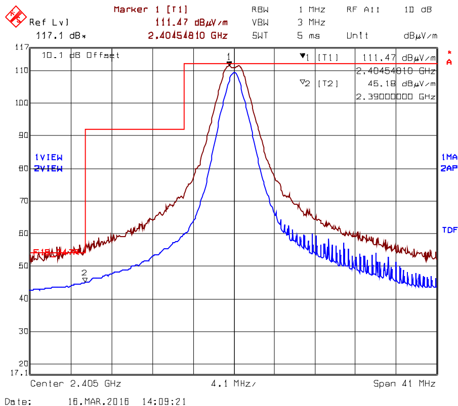
Plot 5.2.4.2.2.1. Band-Edge RF Radiated Emissions at 3 m, Horizontal Polarization Low End of Frequency Band, Ch11- 2405 MHz, QPSK Modulation, Power 8 Mode 1
