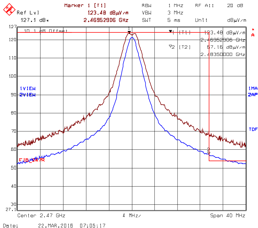
Plot 5.2.4.5.2.4. Band-Edge RF Radiated Emissions at 3 m, Vertical Polarization High End of Frequency Band, Ch24- 2470 MHz, QPSK Modulation, Power 8 Mode 1 @ 66% Duty Cycle
