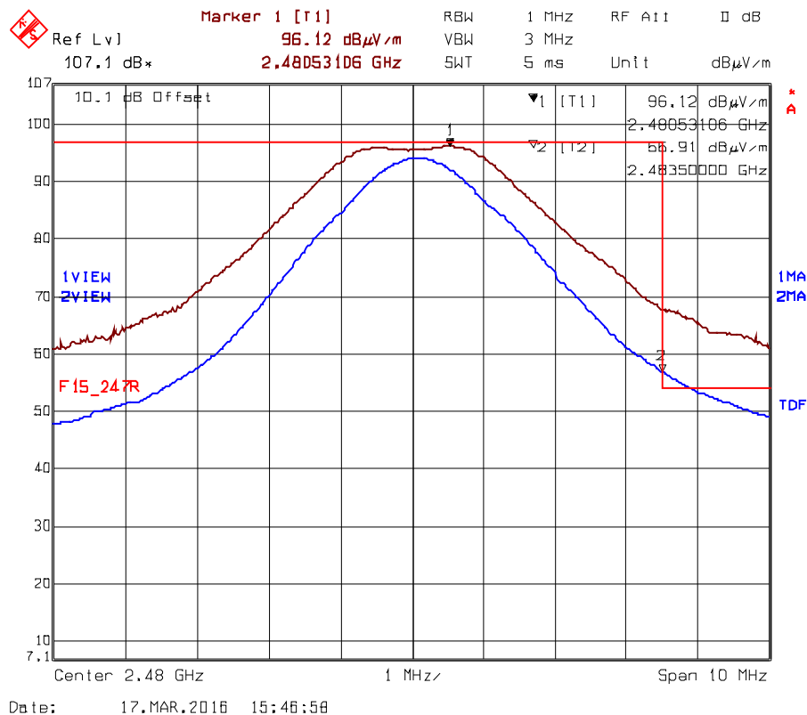
Plot 5.2.4.1.2.5. Band-Edge RF Radiated Emissions at 3 m, Horizontal Polarization Highest End of Frequency Band, Ch26- 2480 MHz, QPSK Modulation, Power -4 Mode 1 @ 66% Duty Cycle
