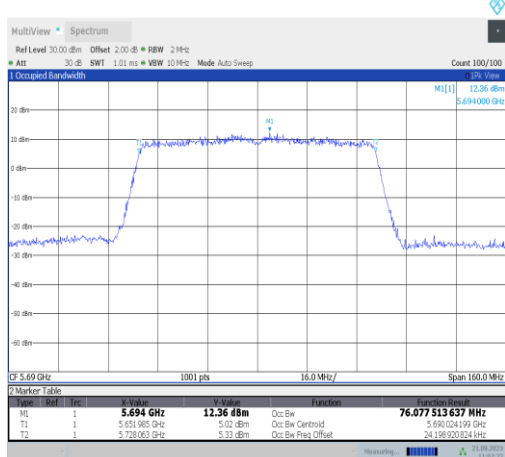
11ac80SISO-Ant23-5690
