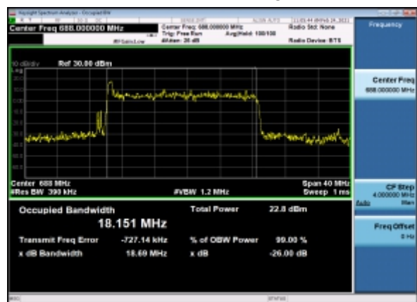
B7_N71(20M)_CP-OFDM_QPSK_Outer_Full High CH
