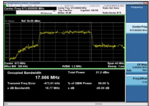
B7_N71(20M)_CP-OFDM_QPSK_Outer_Full_Low_CH
