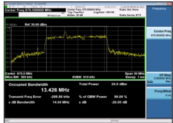
B7_N71(15M)_DFT-s-OFDM_64QAM_Outer_Full_Low_CH
