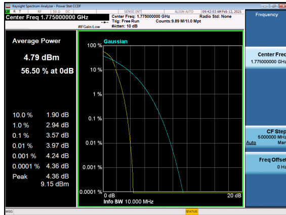
B2_N66(10M)_DFT-s-OFDM_QPSK_Outer_Full_ High_CH
