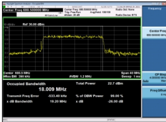
B7_N71(20M)_DFT-s-OFDM_16_QAM_Outer_Full_Mid_CH
