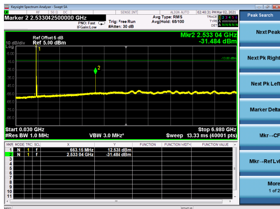
B7_N71(5M)_DFT-s-OFDM_BPSK_Edge_1RB _Left_Low_CH
