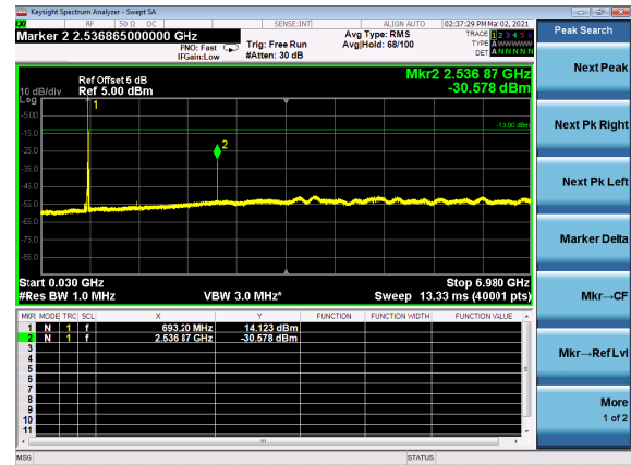
B7_N71(5M)_DFT-s-OFDM_QPSK_Edge_1RB _Left_Mid_CH
