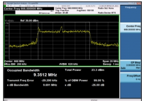
B7_N71(10M)_CP-OFDM_QPSK_Outer_Full_Low_CH
