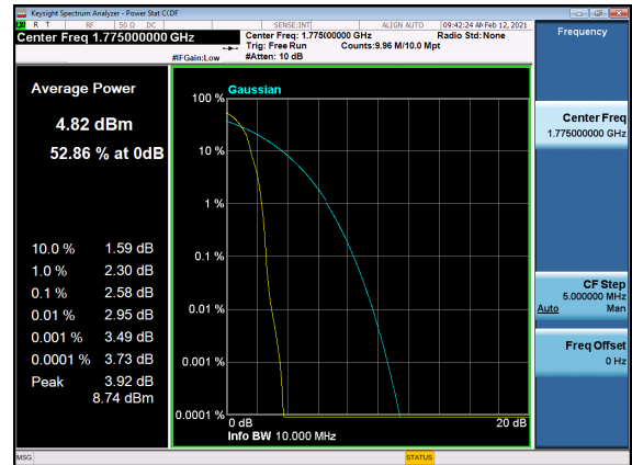
B2_N66(10M)_DFT-s-OFDM_BPSK_Edge_1 RB_Left_High_CH
