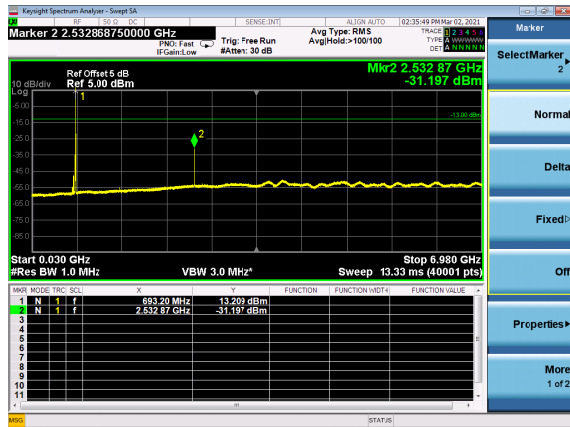
B7_N71(5M)_DFT-s-OFDM_BPSK_Edge_1RB _Left_Mid_CH
