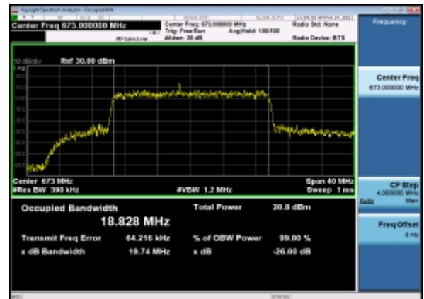
B7_N71(20M)_CP-OFDM_QPSK_Outer_Full_Low_CH
