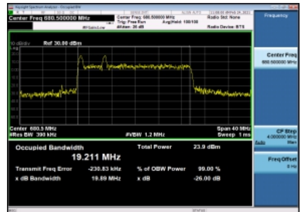
B7_N71(20M)_CP-OFDM_QPSK_Outer_Full_Mid_CH
