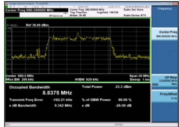
B7_N71(10M)_CP-OFDM_QPSK_Outer_Full_Mid_CH
