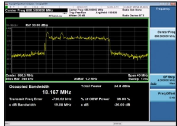
B7_N71(20M)_DFT-s-OFDM_64_QAM_Outer_Full_Mid_CH
