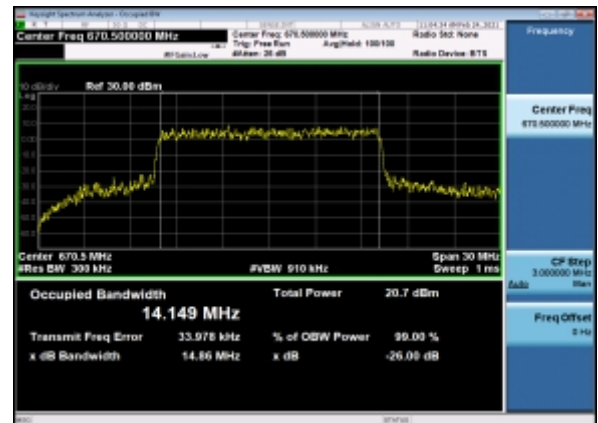
B7_N71(15M)_CP-OFDM_QPSK_Outer_Full_Low_CH
