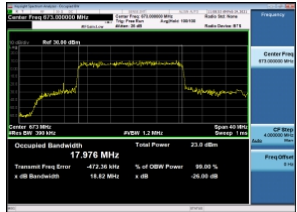
B7_N71(20M)_DFT-s-OFDM_64QAM_Outer_Full_Low_CH
