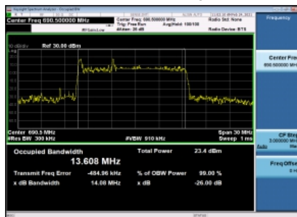
B7_N71(15M)_CP-OFDM_QPSK_Outer_Full High CH
