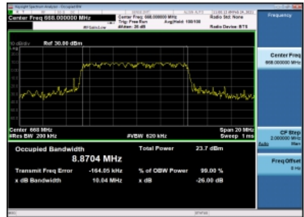
B7_N71(10M)_DFT-s-OFDM_64QAM_Outer_Full_Low_CH
