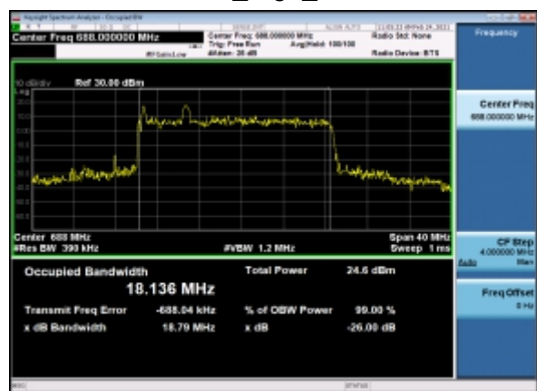
B7_N71(20M)_DFT-s-OFDM_64 QAM Outer Full High CH
