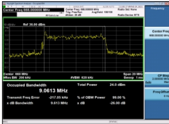
B7_N71(10M)_DFT-s-OFDM_256QAM_Outer_Full_Low_CH
