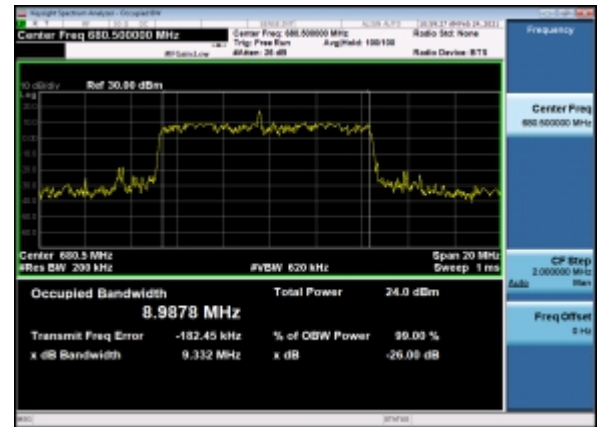
B7_N71(10M)_DFT-s-OFDM_64QAM_Outer_Full_Mid_CH
