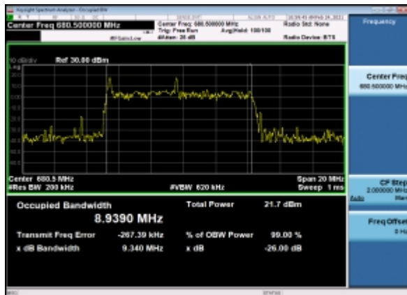
B7_N71(10M)_DFT-s-OFDM_256QAM_Outer_Full_Mid_CH
