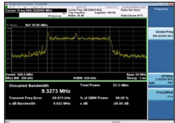
B7_N71(10M)_CP-OFDM_QPSK_Outer_Full_Mid_CH
