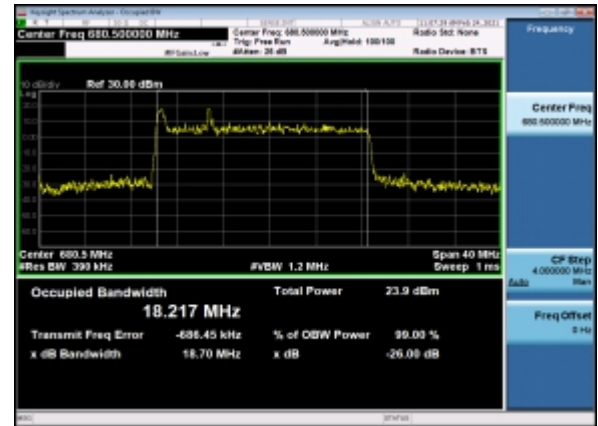
B7_N71(20M)_CP-OFDM_QPSK_Outer_Full_Mid_CH
