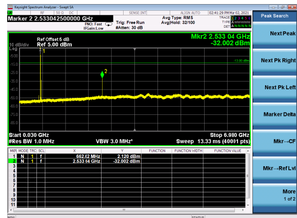
B7_N71(5M)_DFT-s-OFDM_QPSK_Edge_1RB _Left_Low_CH
