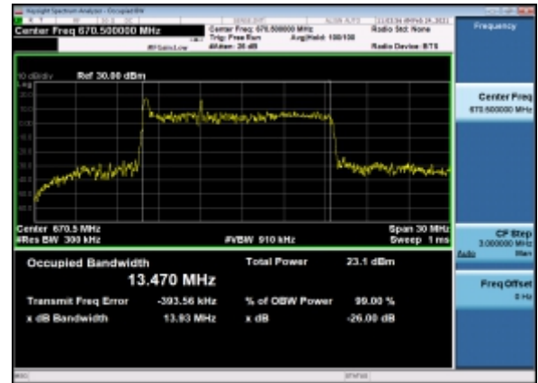
B7_N71(15M)_CP-OFDM_QPSK_Outer_Full_Low_CH
