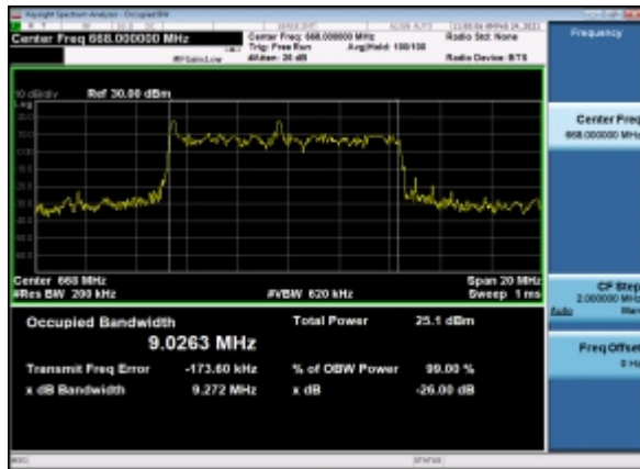
B7_N71(10M)_DFT-s-OFDM_16QAM_Outer_Full_Low_CH
