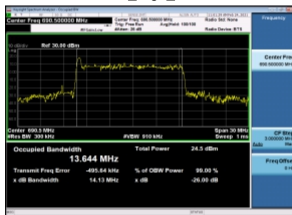
B7_N71(15M)_DFT-s-OFDM_64 QAM Outer Full High CH
