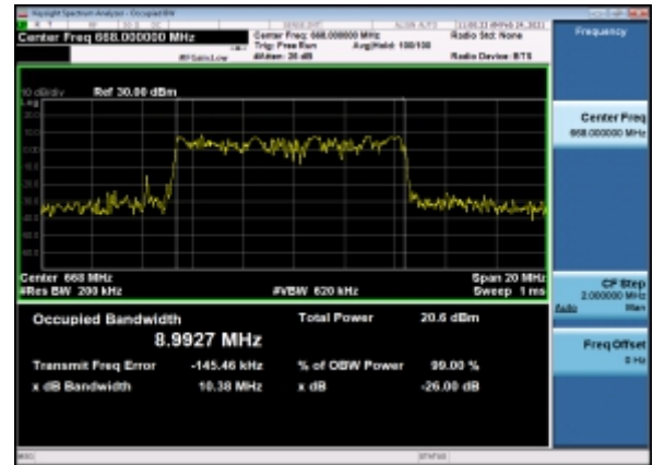
B7_N71(10M)_CP-OFDM_QPSK_Outer_Full_Low_CH
