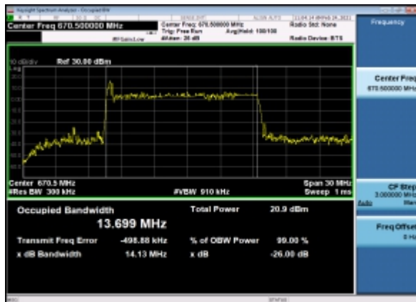
B7_N71(15M)_DFT-s-OFDM_256QAM_Outer_Full_Low_CH
