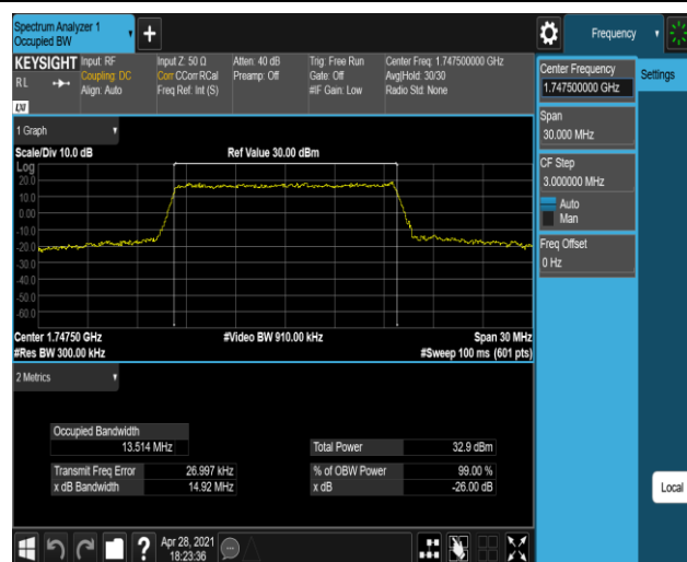
Band4-15MHz-16QAM-20325-75RB#0
