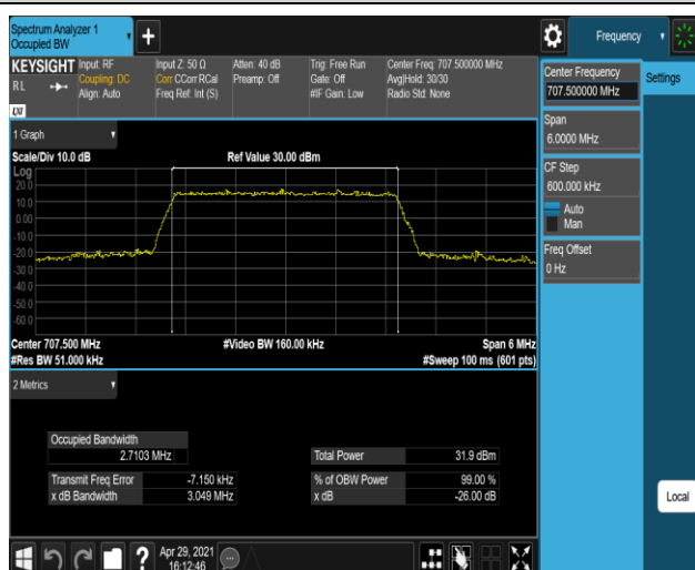
Band12-3MHz-16QAM-23095-15RB#0
