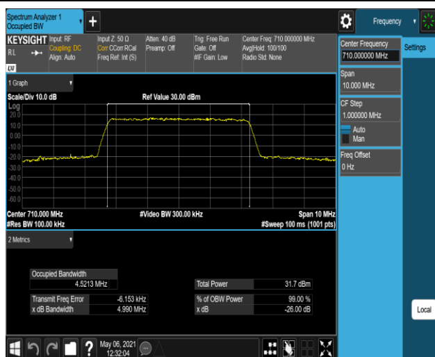
Band17-5MHz-16QAM-23790-25RB#0
