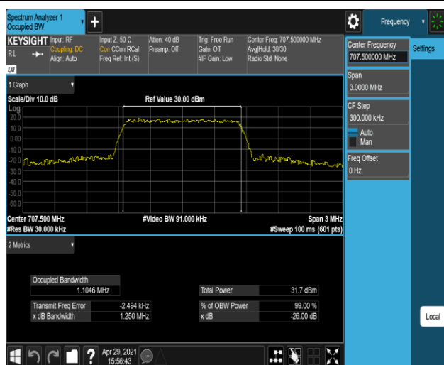
Band12-1.4MHz-16QAM-23095-6RB#0
