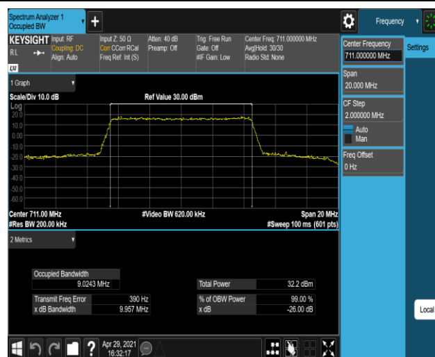
Band12-10MHz-16QAM-23130-50RB#0
