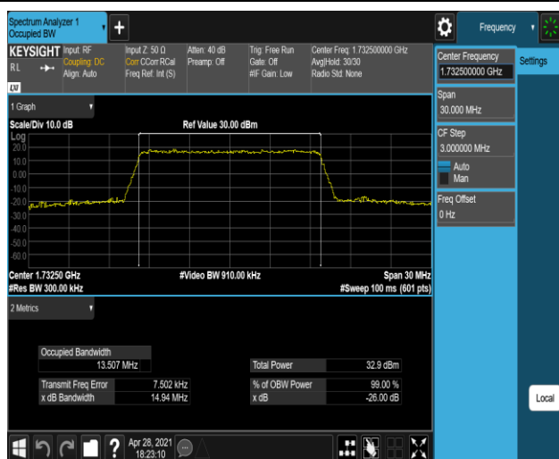
Band4-15MHz-16QAM-20175-75RB#0
