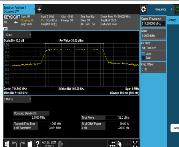
Band12-3MHz-16QAM-23165-15RB#0
