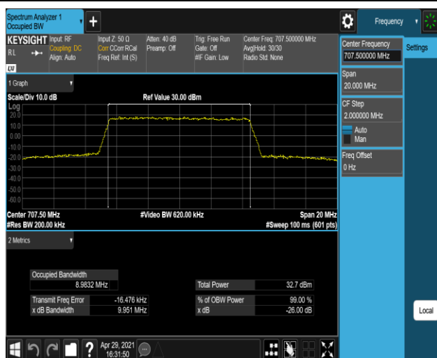
Band12-10MHz-16QAM-23095-50RB#0
