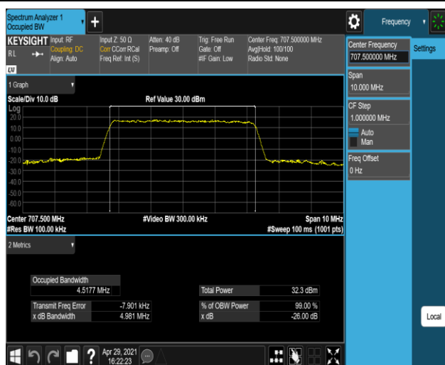
Band12-5MHz-16QAM-23095-25RB#0
