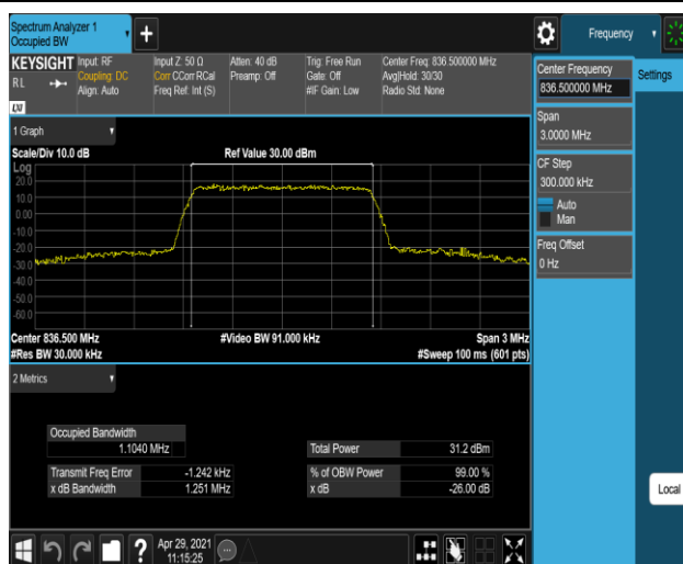
Band5-1.4MHz-16QAM-20525-6RB#0
