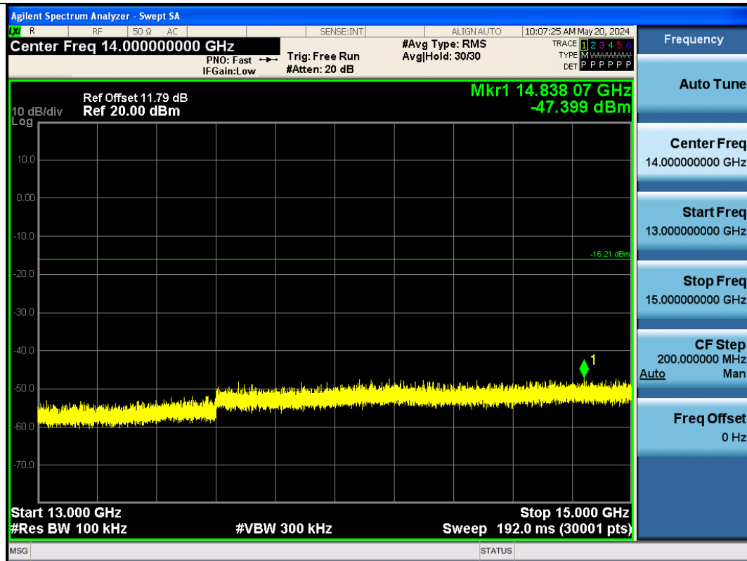
BLE_1M-Ant1-2402-13000~15000-PASS
