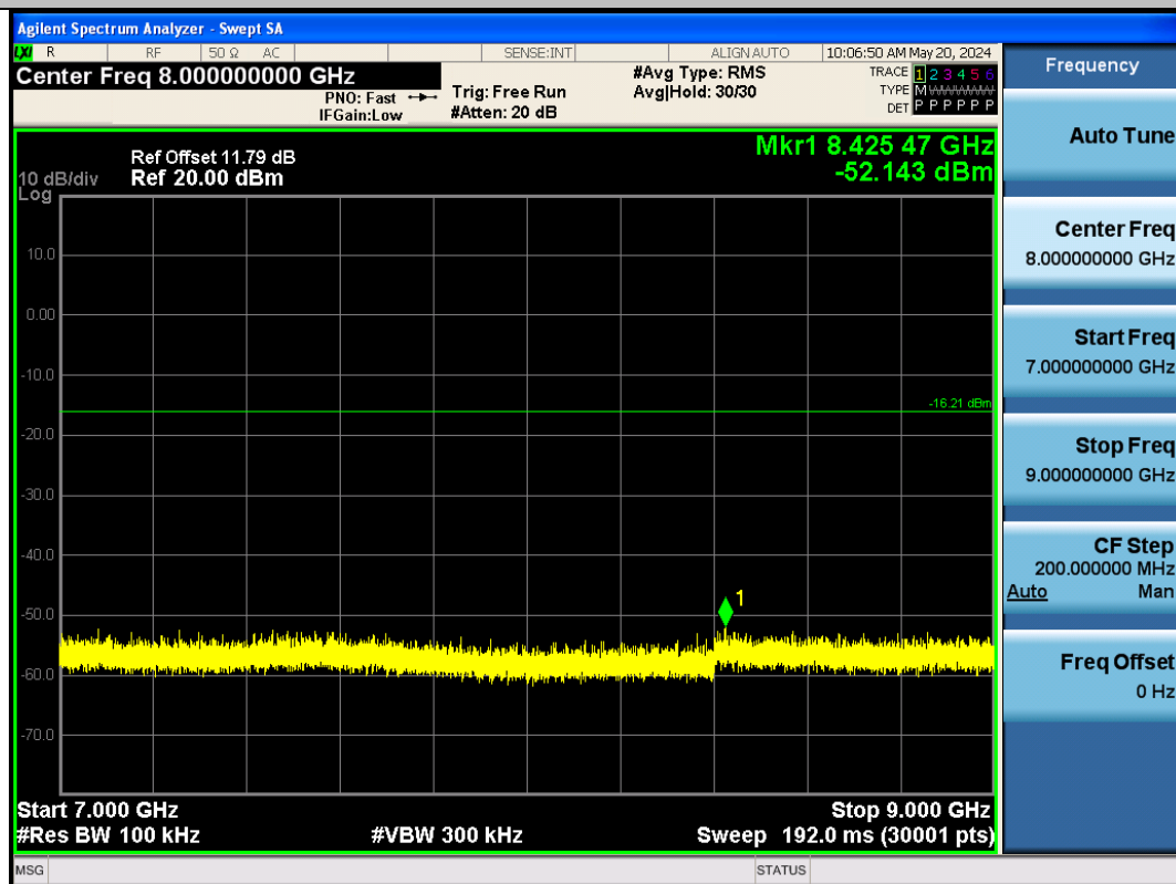
BLE_1M-Ant1-2402-7000~9000-PASS
