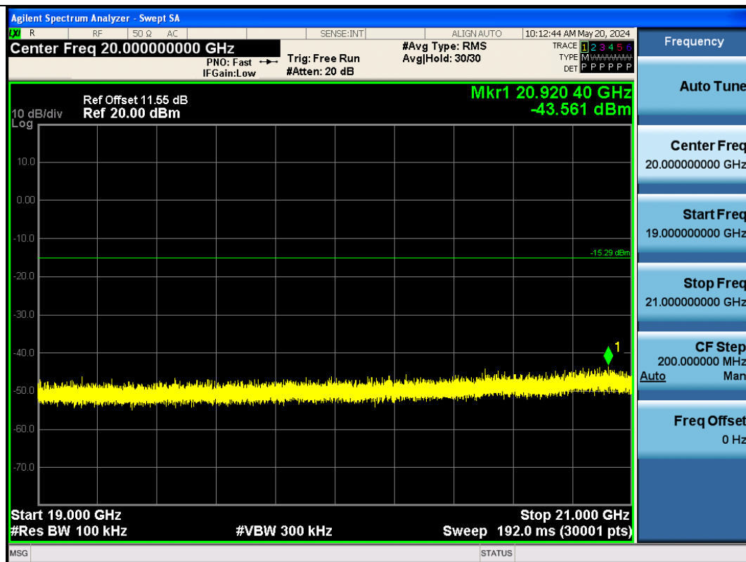
BLE_1M-Ant1-2440-19000~21000-PASS
