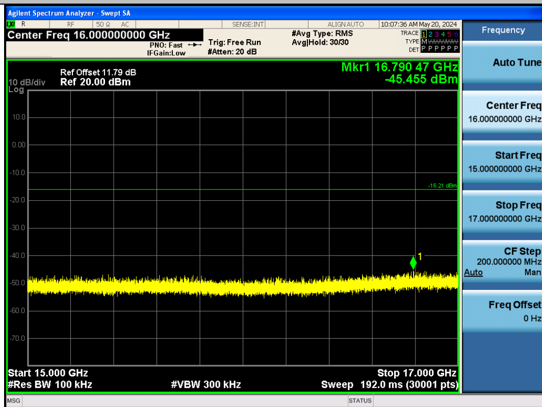
BLE_1M-Ant1-2402-15000~17000-PASS
