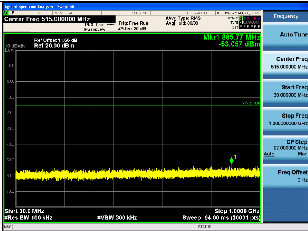
BLE_1M-Ant1-2440-30~1000-PASS
