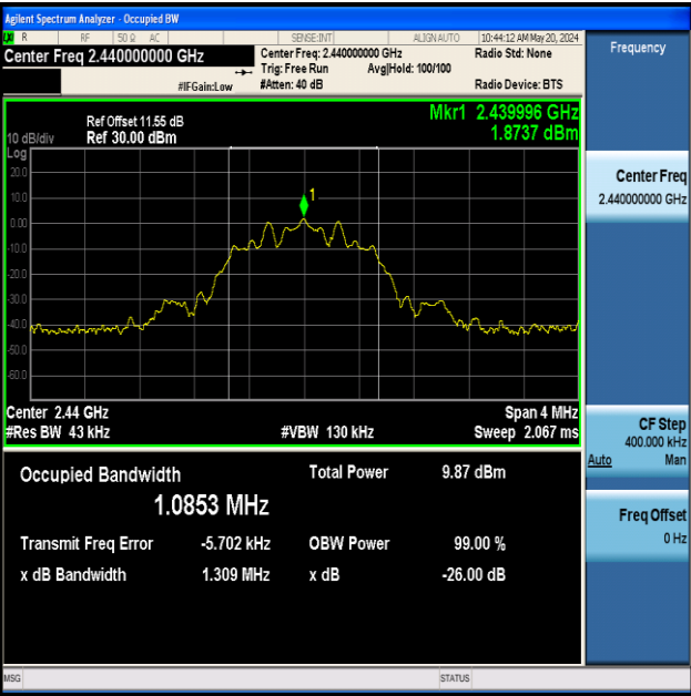
BLE_125K-Ant1-2440
