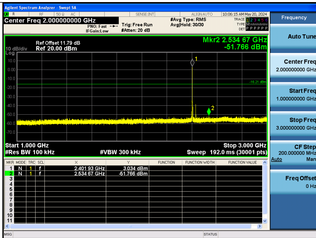
BLE_1M-Ant1-2402-1000~3000-PASS
