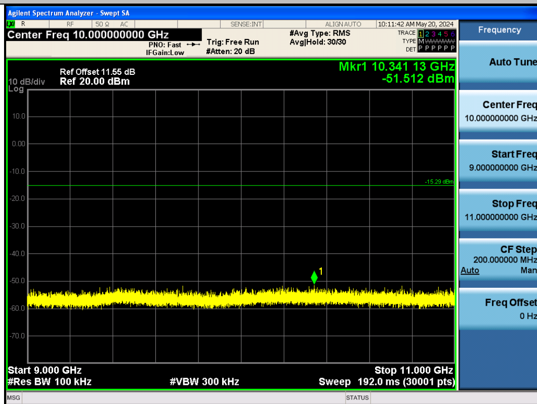
BLE_1M-Ant1-2440-9000~11000-PASS
