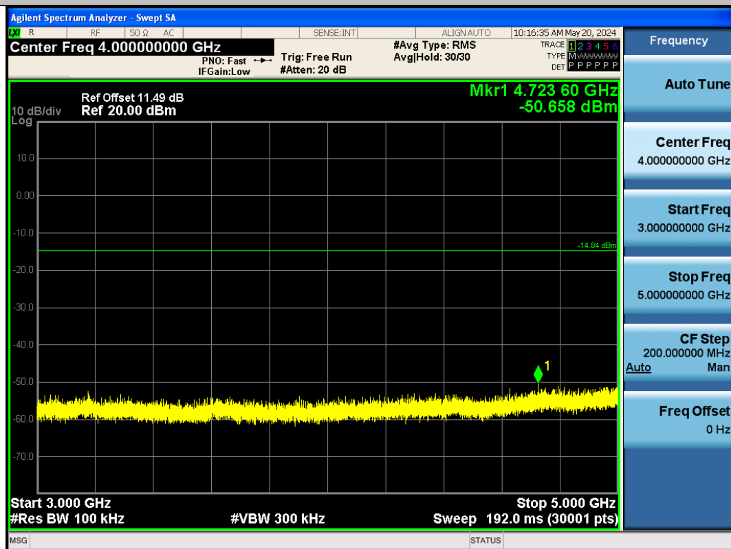
BLE_1M-Ant1-2480-3000~5000-PASS
