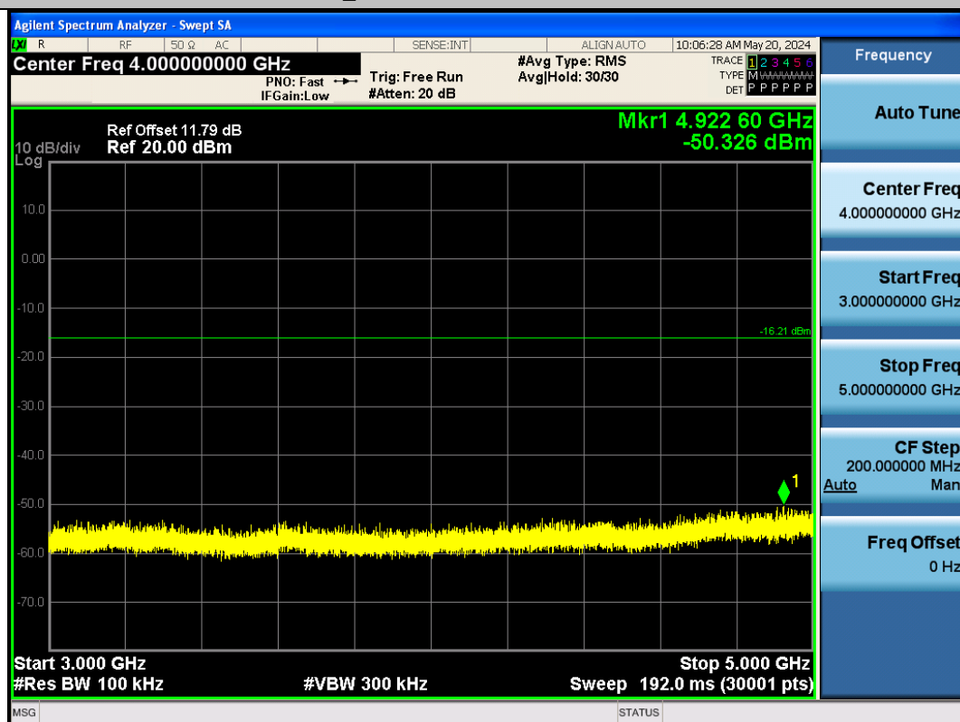
BLE_1M-Ant1-2402-3000~5000-PASS
