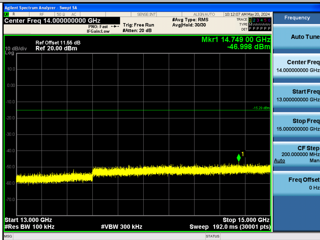
BLE_1M-Ant1-2440-13000~15000-PASS
