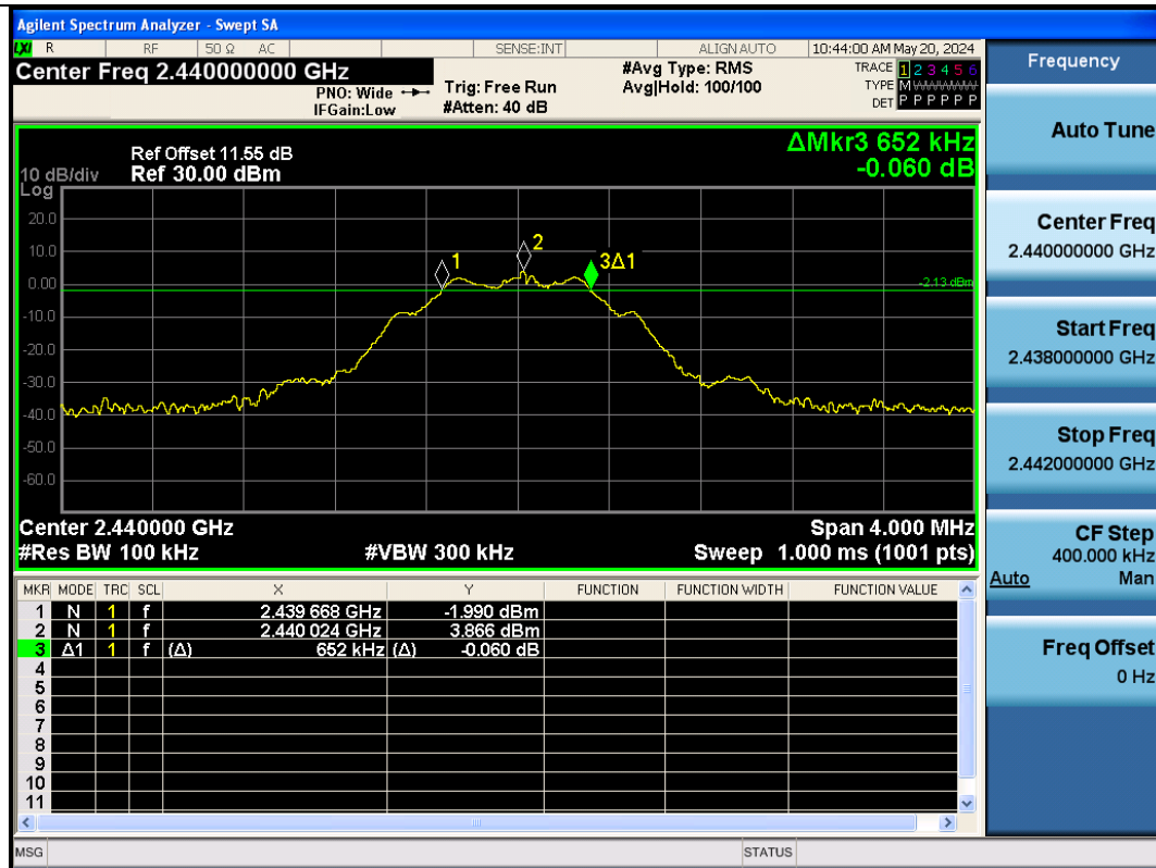
BLE_125K-Ant1-2440-PASS
