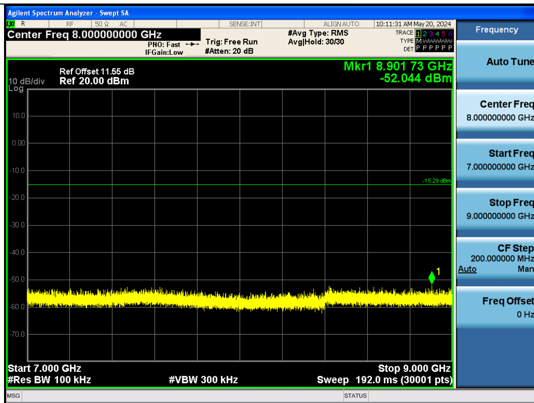
BLE_1M-Ant1-2440-7000~9000-PASS
