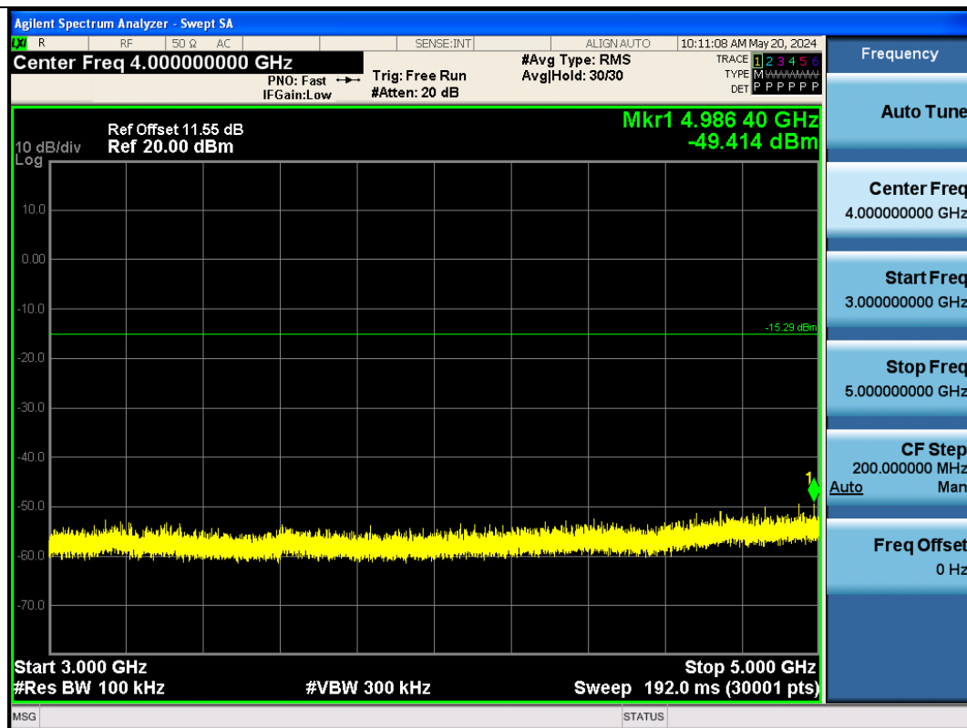
BLE_1M-Ant1-2440-3000~5000-PASS
