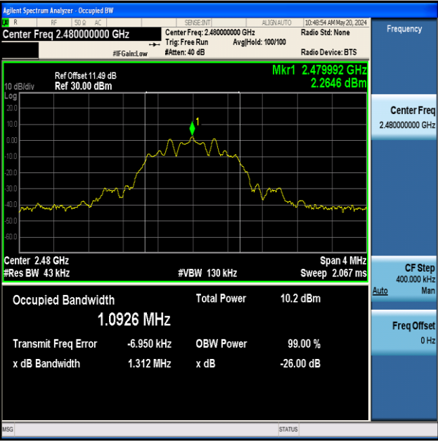
BLE_125K-Ant1-2480
