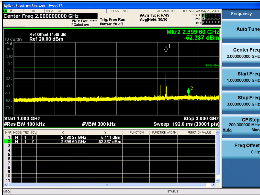
BLE_1M-Ant1-2480-1000~3000-PASS
