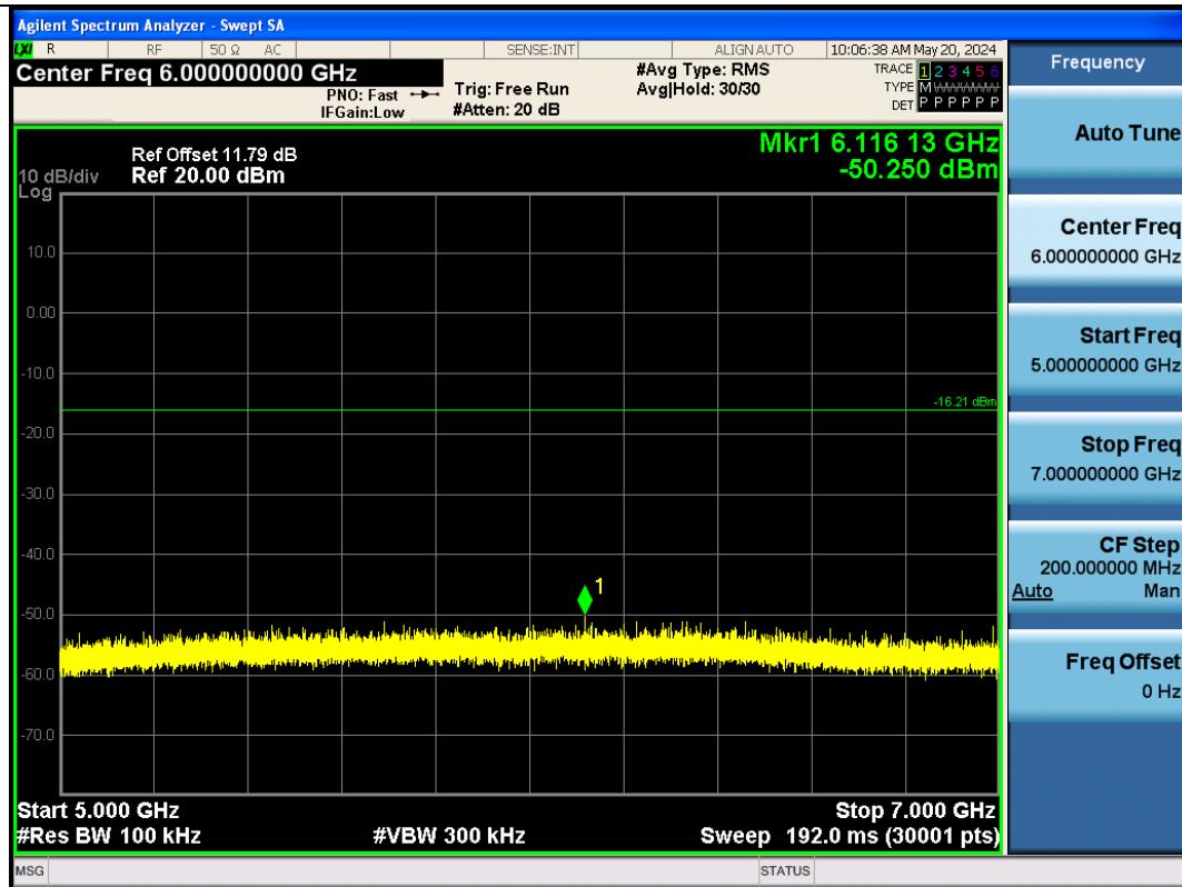
BLE_1M-Ant1-2402-5000~7000-PASS
