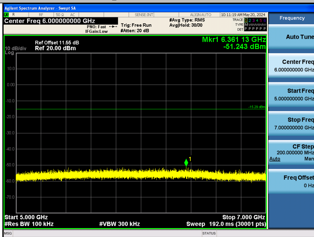
BLE_1M-Ant1-2440-5000~7000-PASS
