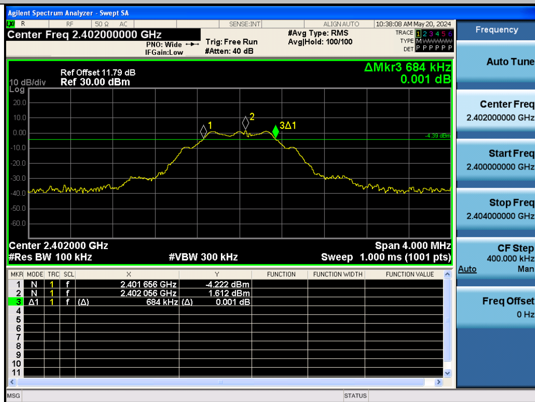
BLE_125K-Ant1-2402-PASS
