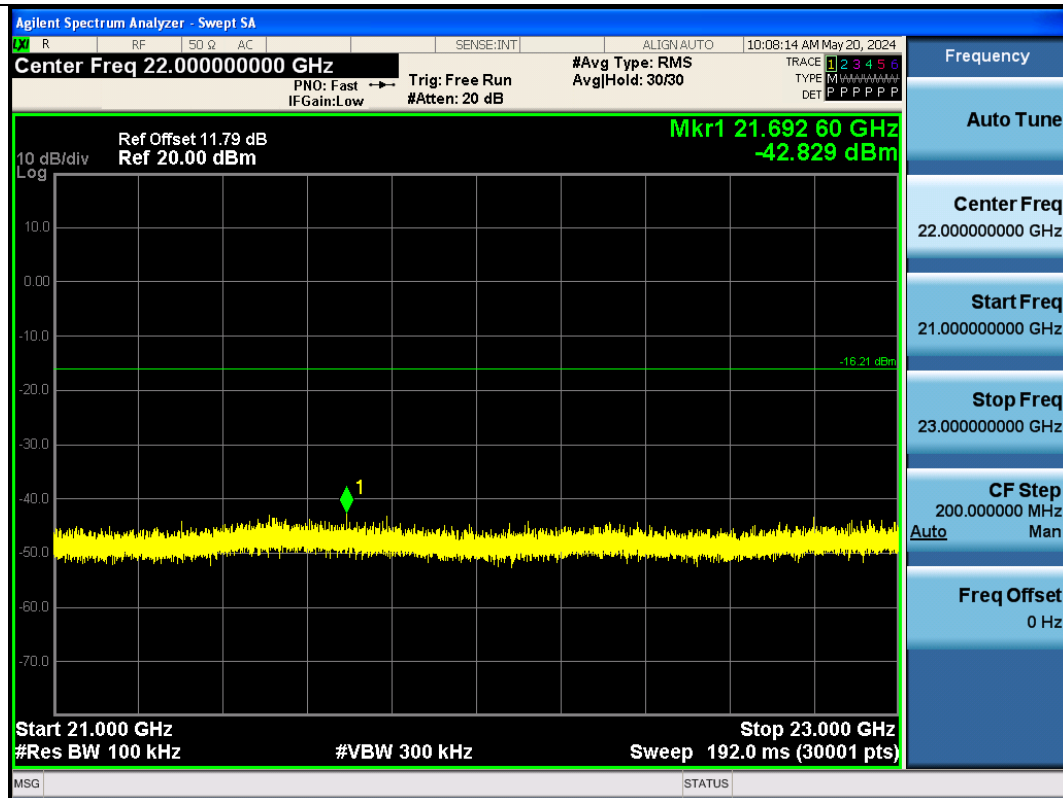
BLE_1M-Ant1-2402-21000~23000-PASS
