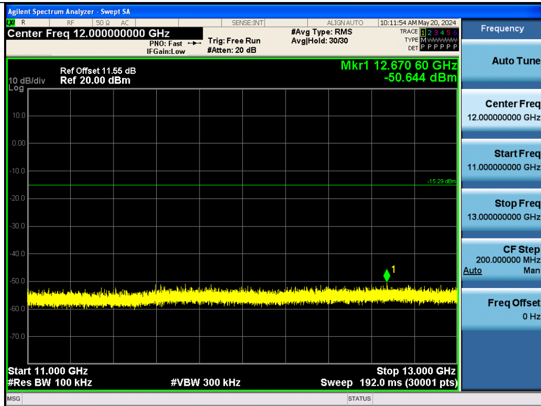
BLE_1M-Ant1-2440-11000~13000-PASS
