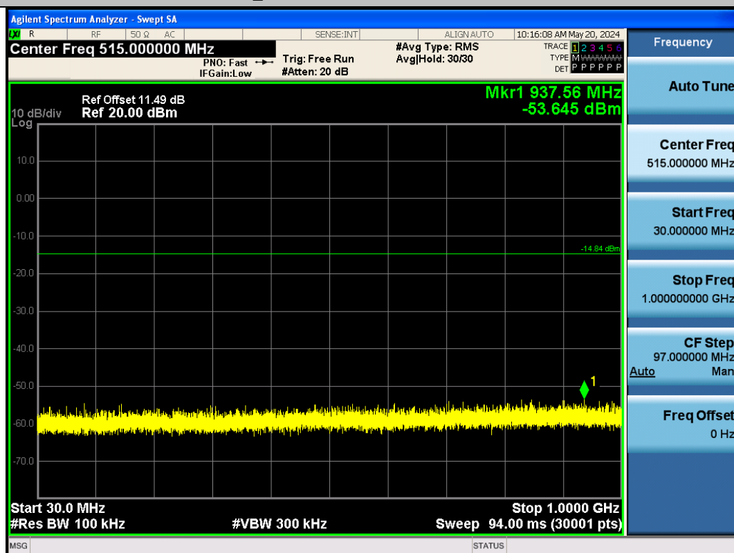
BLE_1M-Ant1-2480-30~1000-PASS
