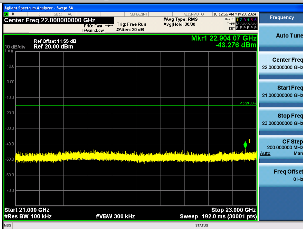
BLE_1M-Ant1-2440-21000~23000-PASS
