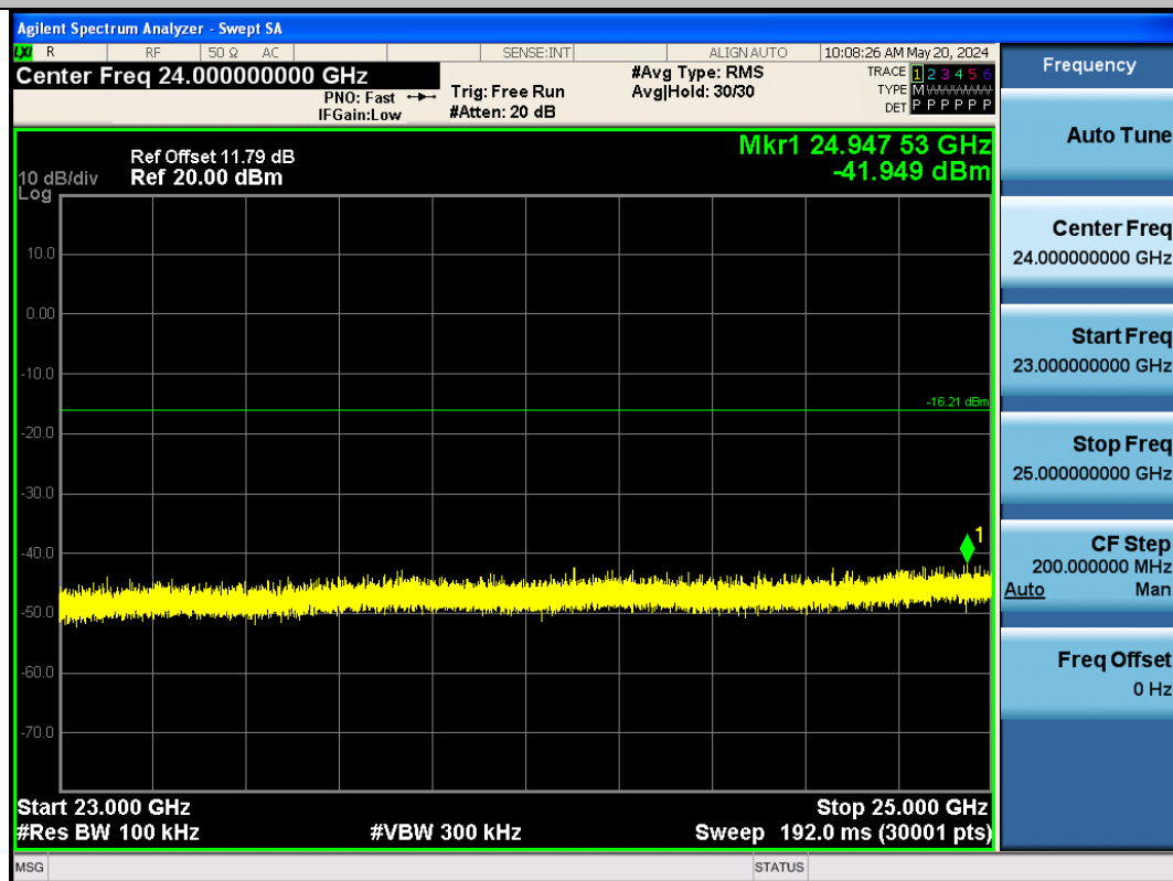
BLE_1M-Ant1-2402-23000~25000-PASS
