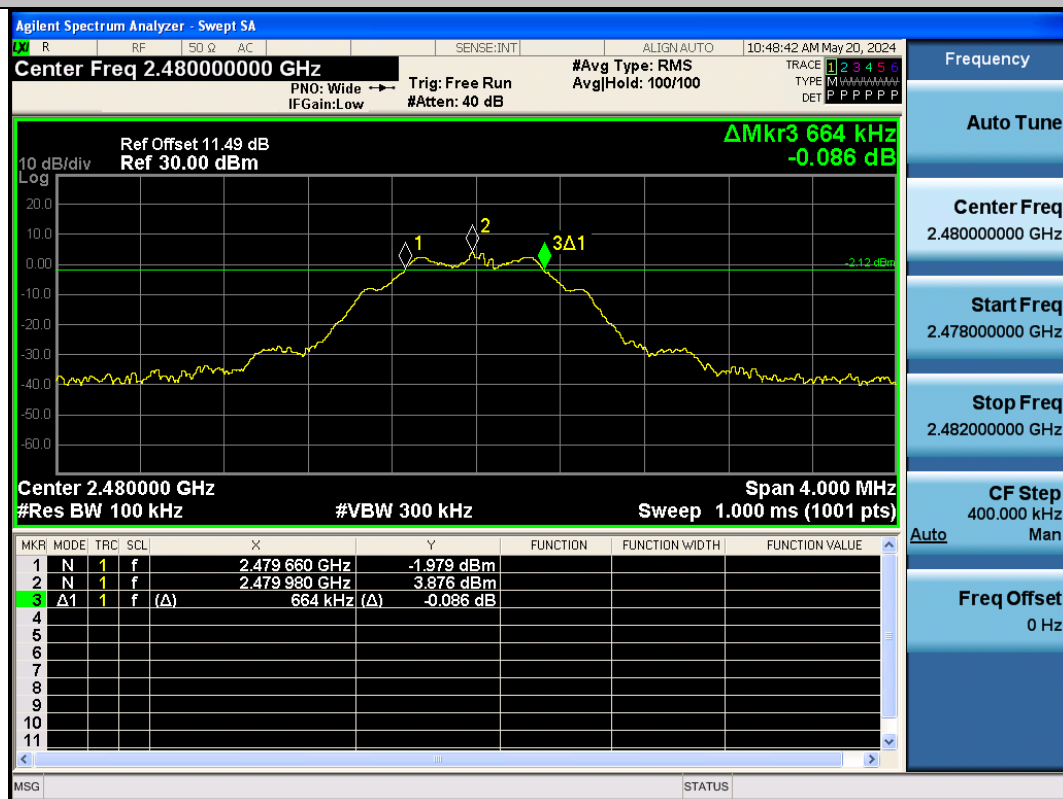
BLE_125K-Ant1-2480-PASS
