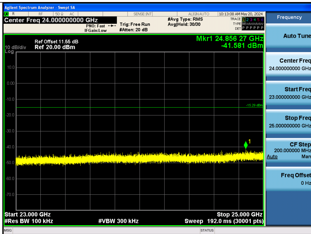
BLE_1M-Ant1-2440-23000~25000-PASS
