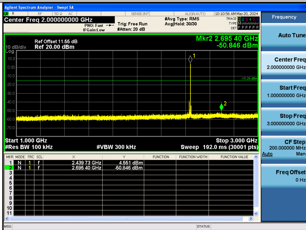
BLE_1M-Ant1-2440-1000~3000-PASS
