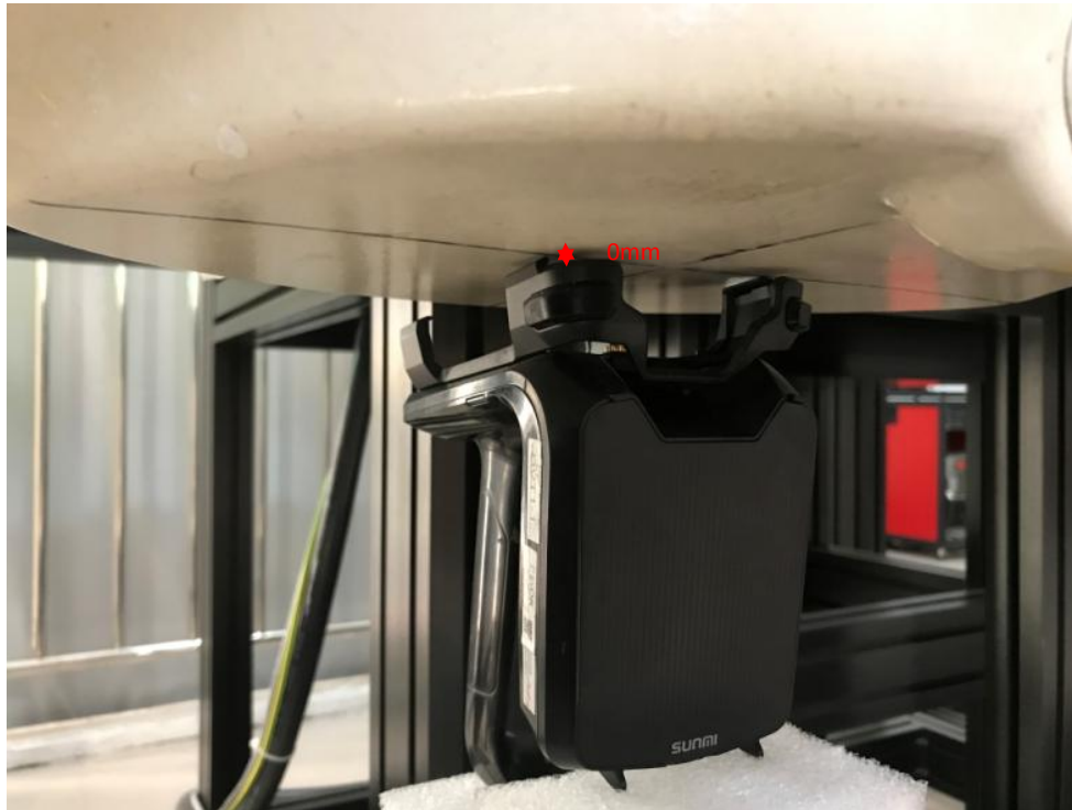
Top Side Setup Photo(0mm)
