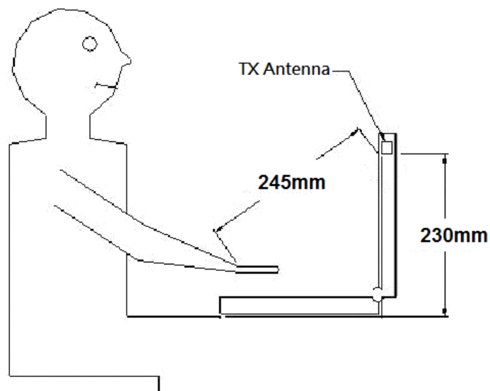
Fig.9 Antenna location of laptop mode - End of Report -
