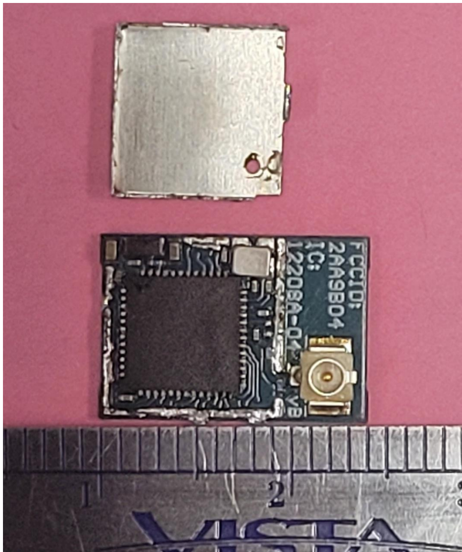
Internal View 1 and PCB Side 1 (Scale in mm)
