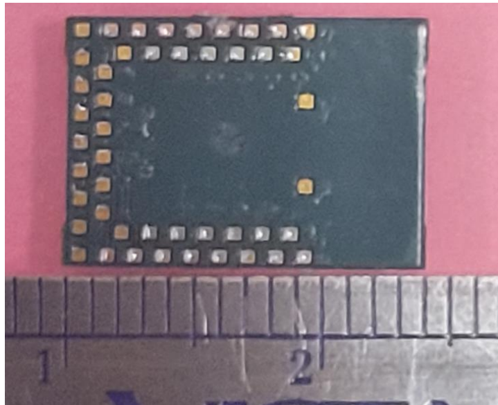
PCB Side 2 (Scale in mm)
