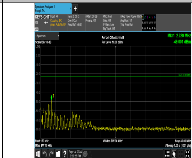
Band26_1.4MHz_QPSK_27033_1RB#5_0.15~30_0.15~30
