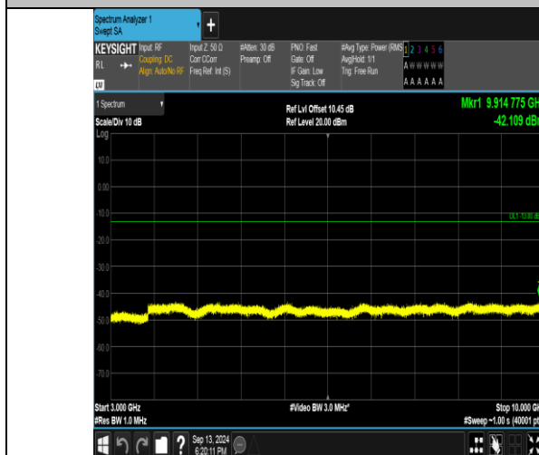
Band26 1.4MHz QPSK 26915 1RB#0 3000~10000 3000~10000
