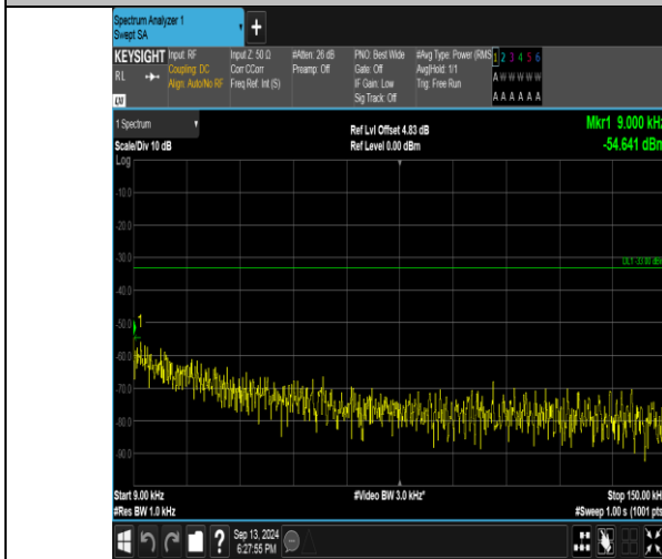
Band26_1.4MHz_QPSK_27033_6RB#0_0.009~0.15_0.009~0.15
