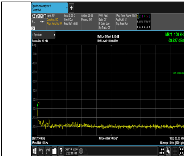
Band26_1.4MHz_16QAM_26915_1RB#0_0.15~30_0.15~30
