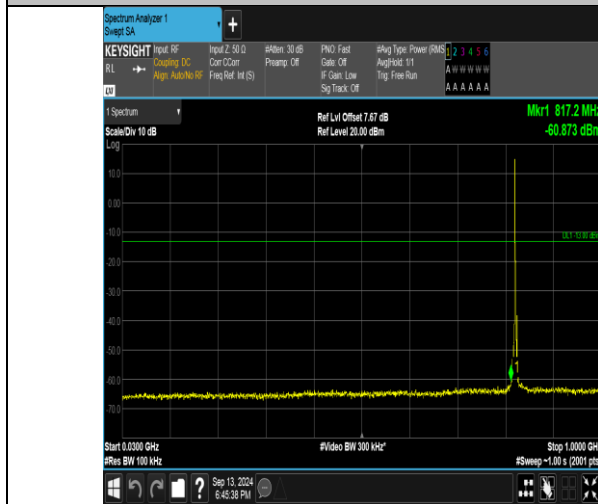
Band26_3MHz_QPSK_26805_1RB#0_30~1000_30~1000
