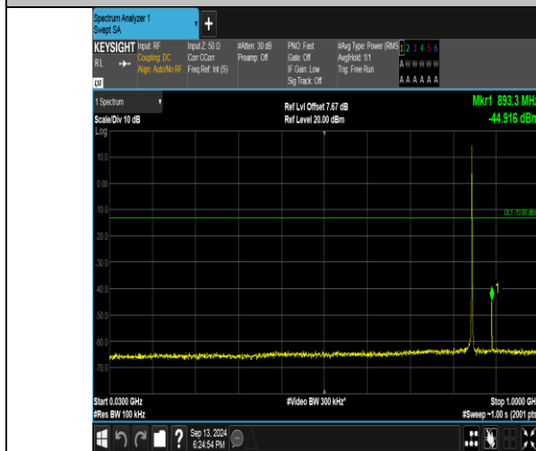
Band26_1.4MHz_QPSK_27033_1RB#0_30~1000_30~1000
