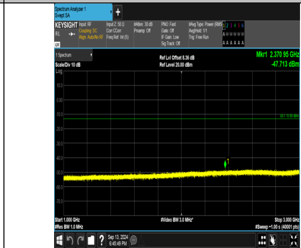
Band26_3MHz_QPSK_26805_1RB#0_1000~3000_1000~3000
