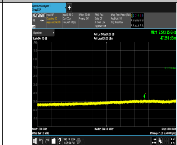
Band26_1.4MHz_QPSK_27033_1RB#0_1000~3000_1000~3000
