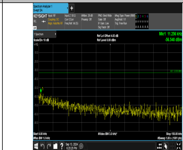
Band26_1.4MHz_16QAM_27033_1RB#0_0.009~0.15_0.009~0.15
