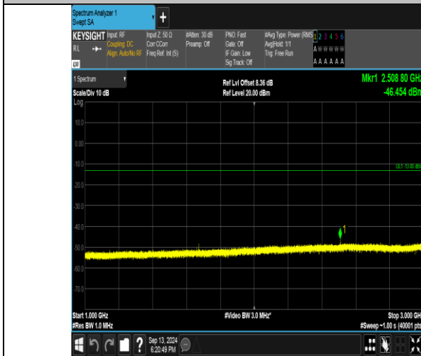
Band26_1.4MHz_16QAM_26915_1RB#0_1000~3000_1000~3000
