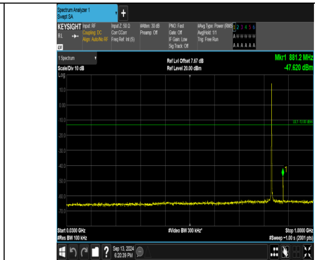
Band26_1.4MHz_16QAM_26915_1RB#0_30~1000_30~1000
