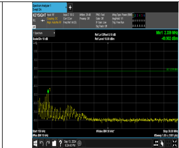
Band26_1.4MHz_QPSK_27033_1RB#0_0.15~30_0.15~30
