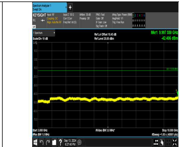
Band26_1.4MHz_16QAM_27033_1RB#5_3000~10000_3000~10000
