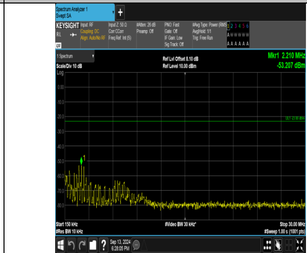
Band26_1.4MHz_QPSK_27033_6RB#0_0.15~30_0.15~30
