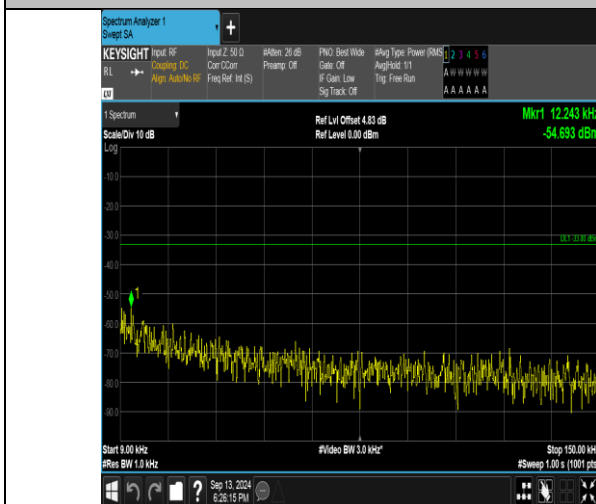
Band26_1.4MHz_QPSK_27033_1RB#5_0.009~0.15_0.009~0.15
