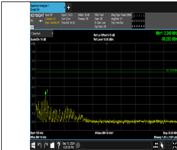
Band26_1.4MHz_16QAM_27033_1RB#0_0.15~30_0.15~30
