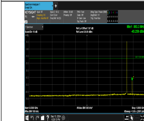
Band26_1.4MHz_QPSK_27033_6RB#0_30~1000_30~1000
