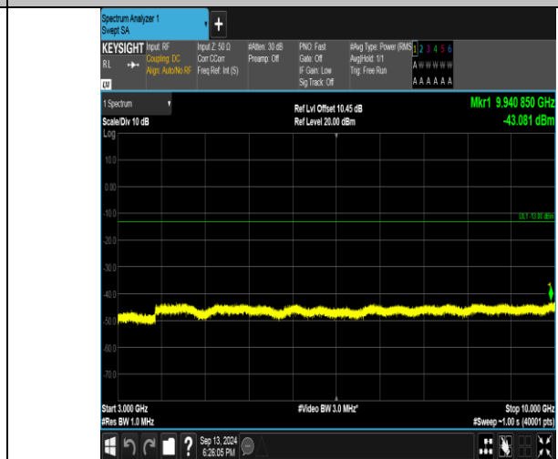
Band26_1.4MHz_16QAM_27033_1RB#0_3000~10000_3000~10000
