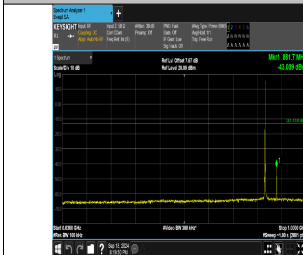
Band26 1.4MHz QPSK 26915 1RB#0 30~1000 30~1000
