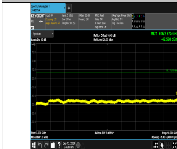
Band26_3MHz_QPSK_26805_1RB#0_3000~10000_3000~10000
