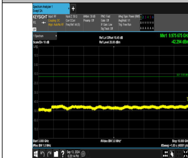
Band26_1.4MHz_QPSK_27033_1RB#0_3000~10000_3000~10000
