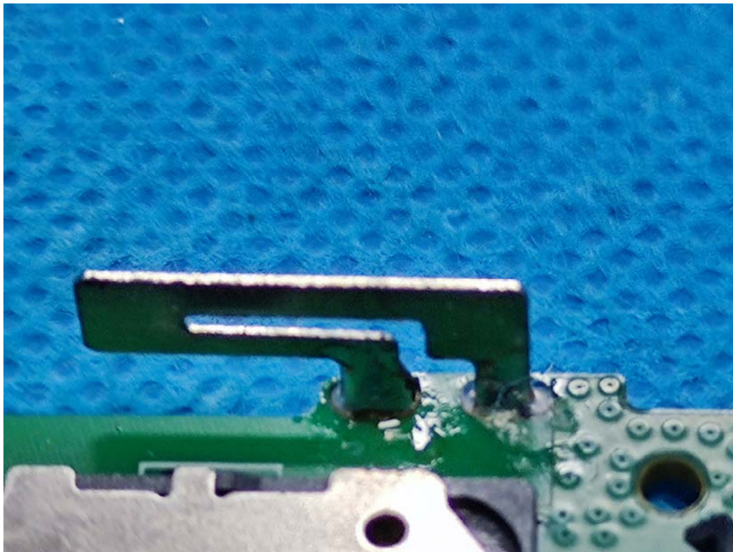
WLAN Antenna
