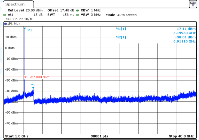
11A-Ant2-5200-1000~40000-PASS
