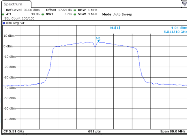
11AC40-CDD-Ant1-5510-PASS
