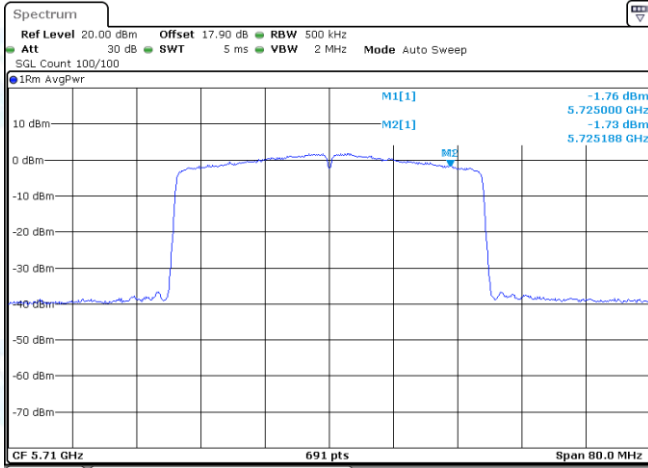
11AX40-CDD-Ant1-5710_UNII-3-PASS
