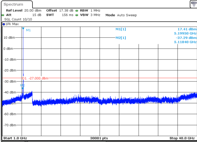
11A-Ant1-5200-1000~40000-PASS
