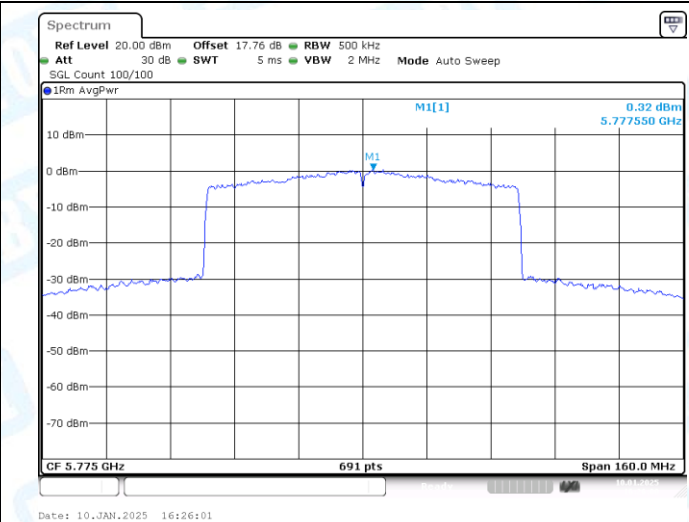
11AX80-CDD-Ant2-5775-PASS
