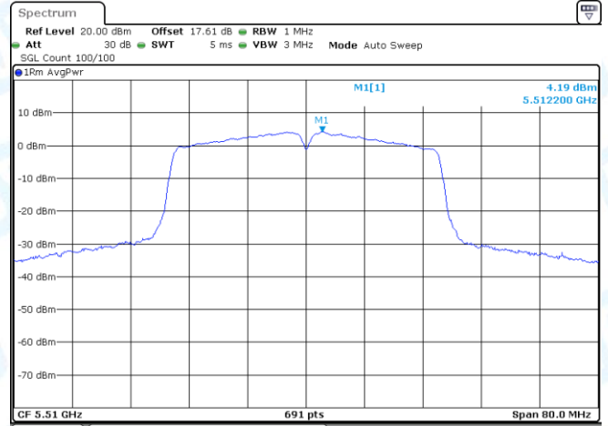
11AC40-CDD-Ant2-5510-PASS
