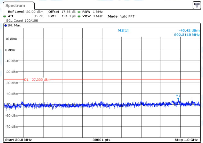
11A-Ant2-5260-30~1000-PASS
