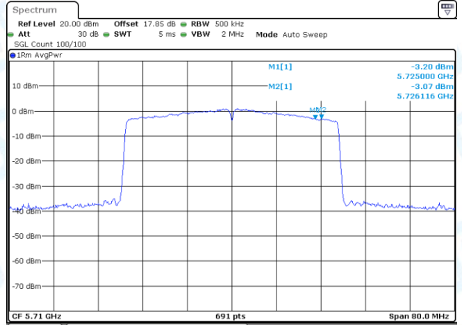
11AX40-CDD-Ant2-5710_UNII-3-PASS
