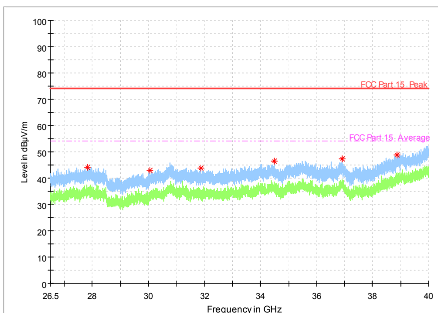
Fig. 62 Radiated emission: 802.11n, (802.11n-HT20, Ch165, 26.5 GHz - 40 GHz)
