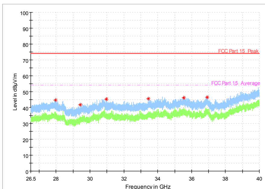
Fig. 42 Radiated emission: 802.11n, (802.11a, Ch157, 26.5 GHz - 40 GHz)
