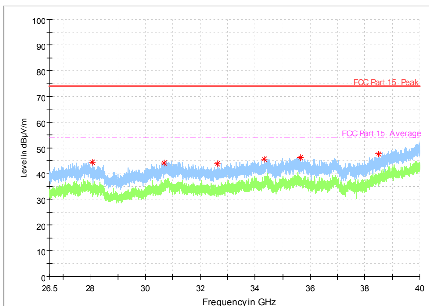
Fig. 37 Radiated emission: 802.11n, (802.11a, Ch149, 26.5 GHz - 40 GHz)
