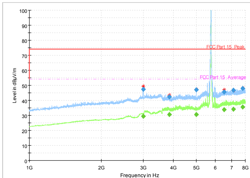
Fig. 74 Radiated Spurious Emission (802.11a, Ch149, 1 GHz-8 GHz)
