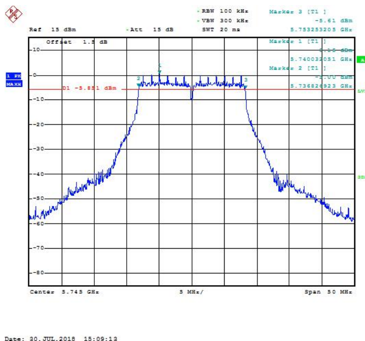
Fig. 1 Occupied 6dB Bandwidth (802.11a, Ch 149)
