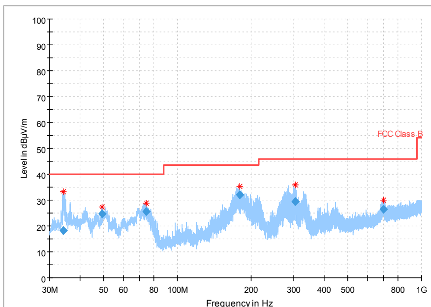
Fig. 78 Radiated Spurious Emission (802.11a, Ch149, 30 MHz-1 GHz)
