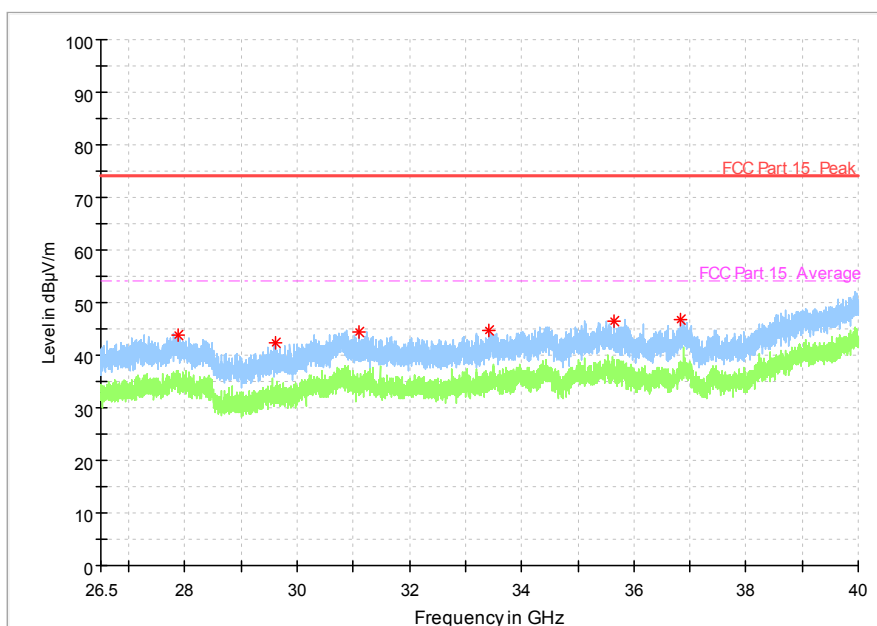
Fig. 47 Radiated emission: 802.11n, (802.11a, Ch165, 26.5 GHz - 40 GHz)
