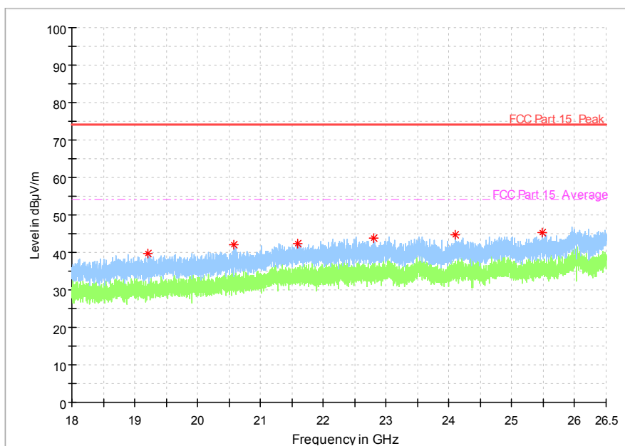
Fig. 36 Radiated Spurious Emission (802.11a, Ch149, 18 GHz-26.5 GHz)
