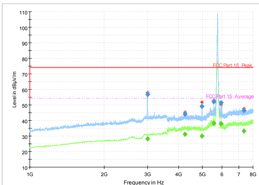
Fig. 49 Radiated Spurious Emission (802.11n-HT20, Ch149, 1 GHz-8 GHz)
