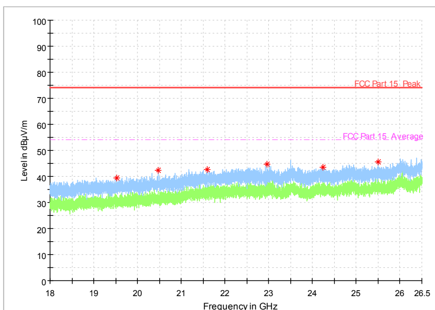
Fig. 46 Radiated Spurious Emission (802.11a, Ch165, 18 GHz-26.5 GHz)
