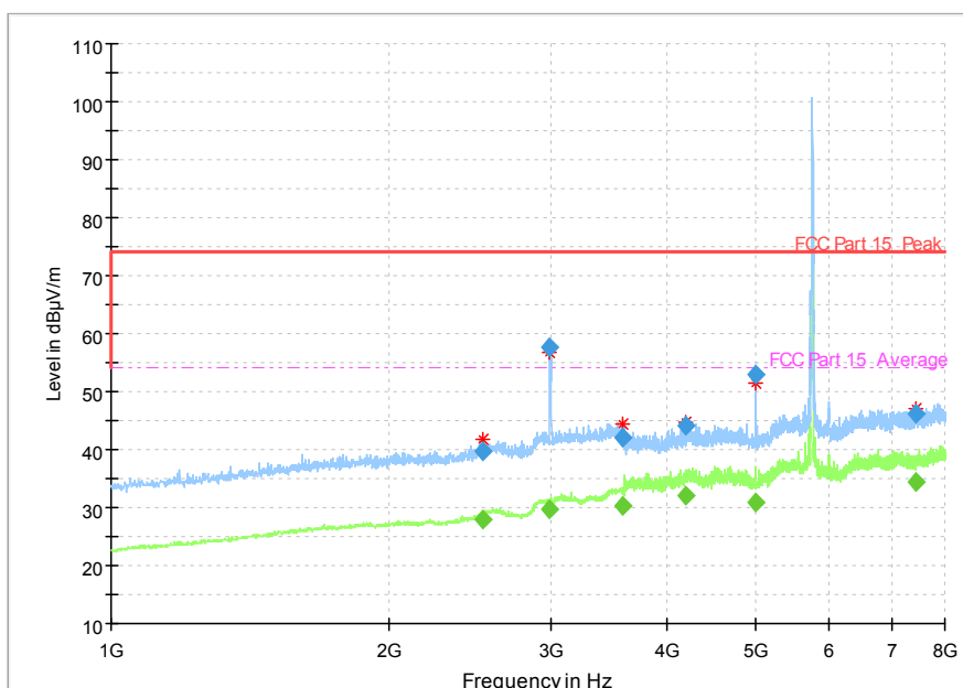
Fig. 79 Radiated Spurious Emission (802.11a, Ch149, 1 GHz-8 GHz)
