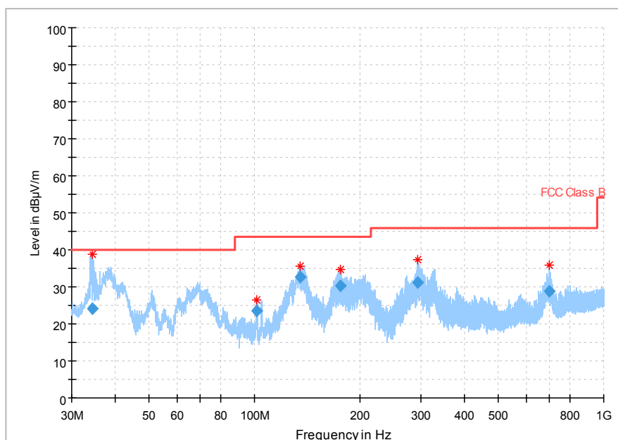
Fig. 68 Radiated Spurious Emission (802.11n-HT40, Ch159, 30 MHz-1 GHz)
