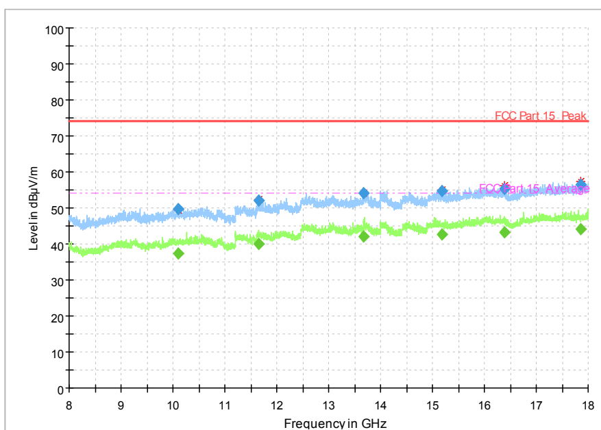
Fig. 50 Radiated Spurious Emission (802.11n-HT20, Ch149, 8 GHz-18 GHz)
