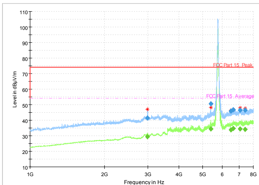
Fig. 64 Radiated Spurious Emission (802.11n-HT40, Ch151, 1 GHz-8 GHz)
