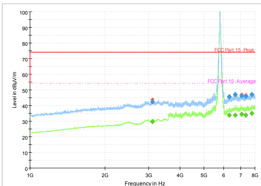
Fig. 69 Radiated Spurious Emission (802.11n-HT40, Ch159, 1 GHz-8 GHz)
