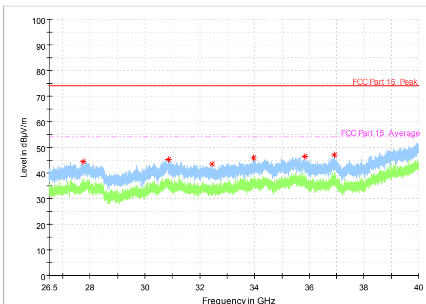
Fig. 77 Radiated Spurious Emission (802.11a, Ch149, 26.5 GHz-40 GHz)
