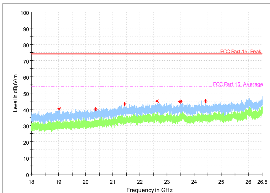
Fig. 56 Radiated Spurious Emission (802.11n-HT20, Ch157, 18 GHz-26.5 GHz)
