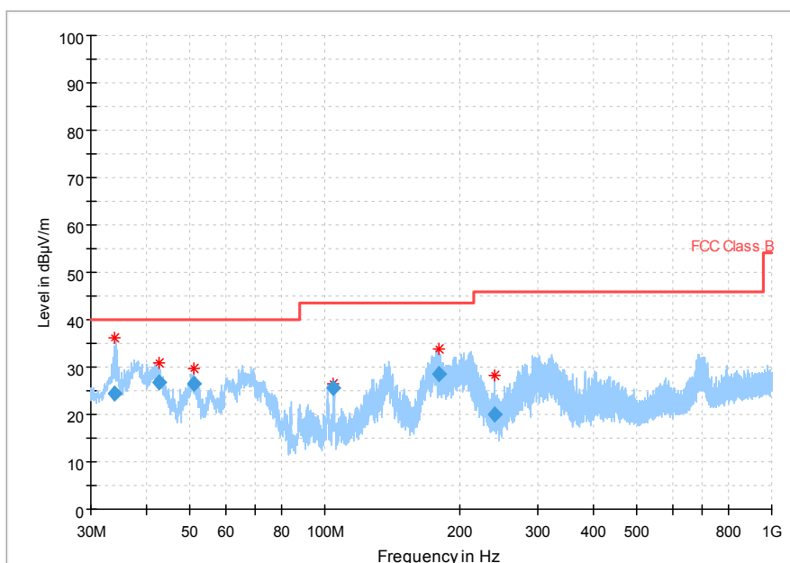
Fig. 38 Radiated Spurious Emission (802.11a, Ch157, 30 MHz-1 GHz)
