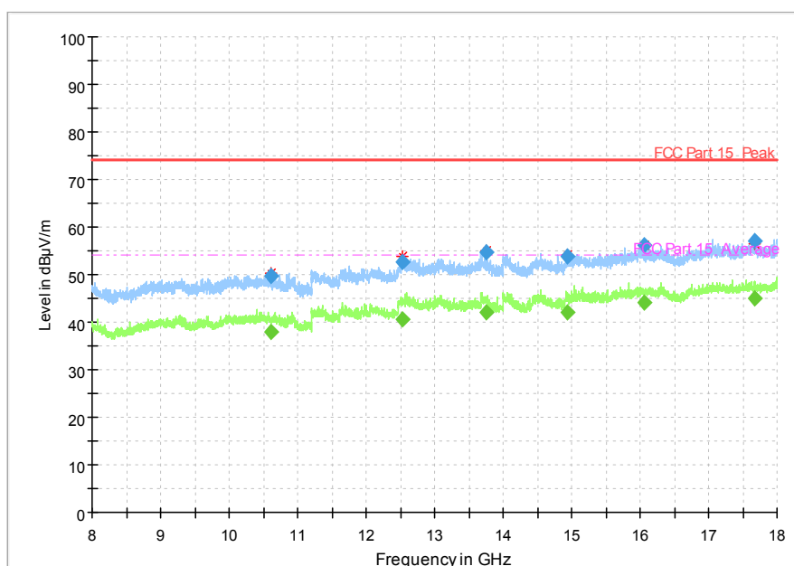
Fig. 40 Radiated Spurious Emission (802.11a, Ch157, 8 GHz-18 GHz)
