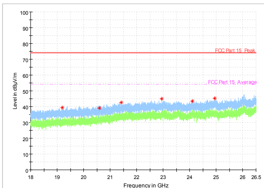
Fig. 41 Radiated Spurious Emission (802.11a, Ch157, 18 GHz-26.5 GHz)
