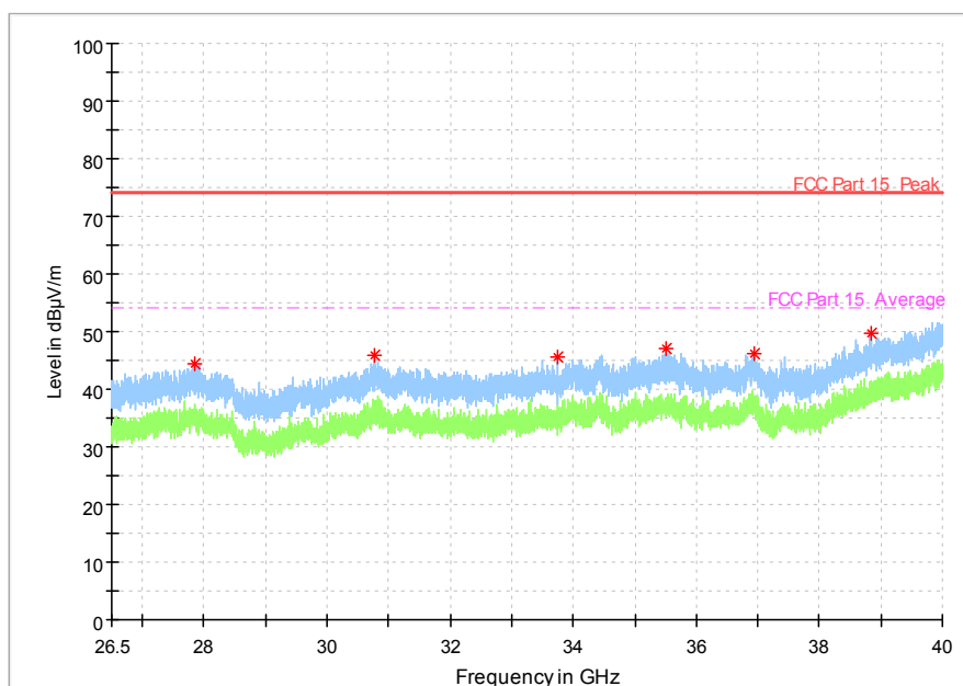
Fig. 67 Radiated emission: 802.11n, (802.11n-HT40, Ch151, 26.5 GHz - 40 GHz)
