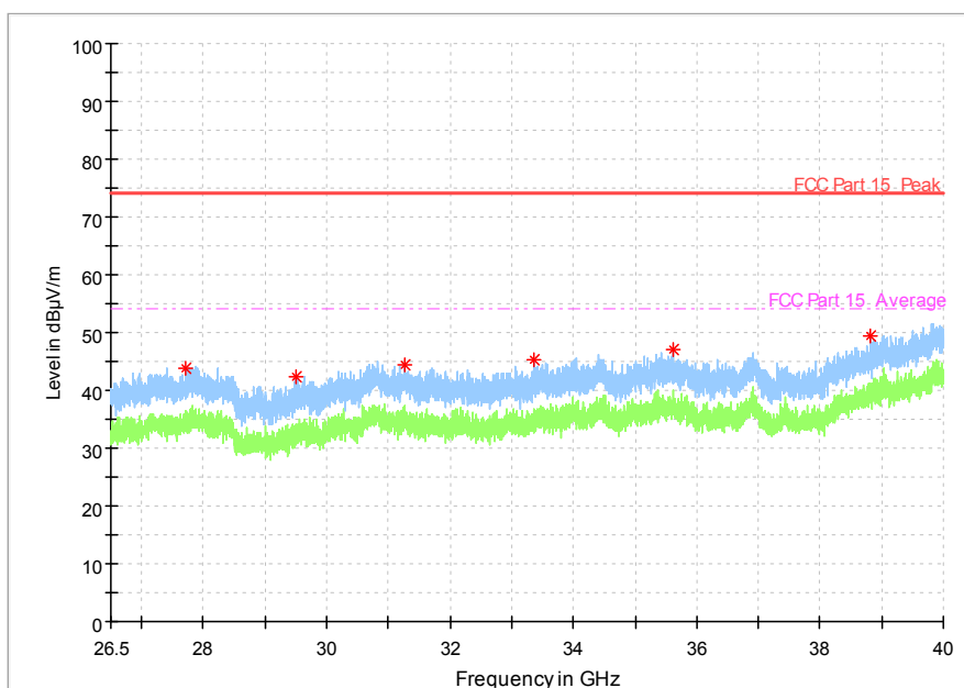
Fig. 57 Radiated emission: 802.11n, (802.11n-HT20, Ch157, 26.5 GHz - 40 GHz)
