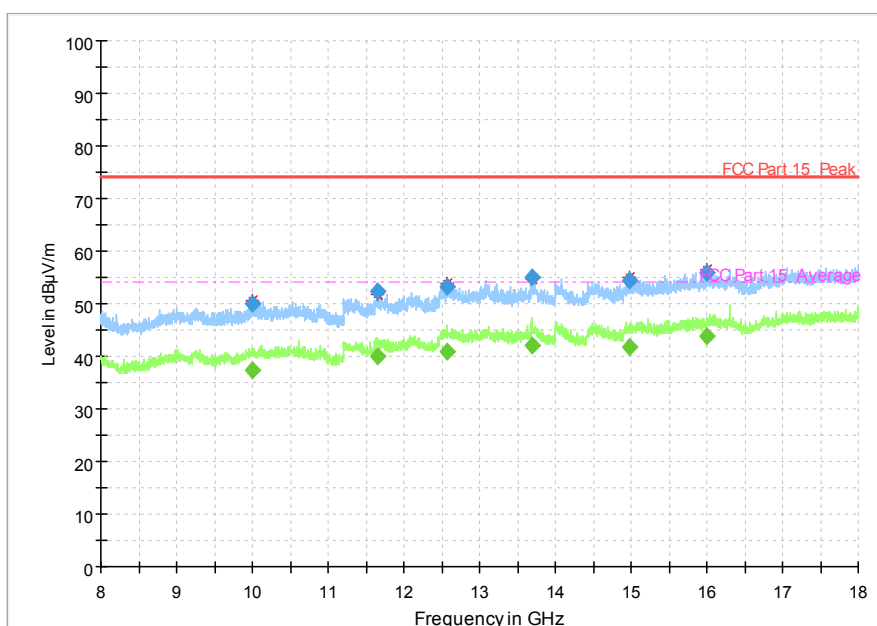
Fig. 60 Radiated Spurious Emission (802.11n-HT20, Ch165, 8 GHz-18 GHz)
