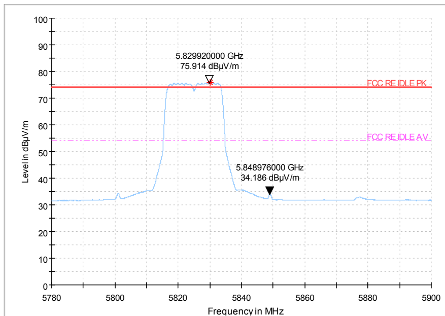
Fig. 86 Band Edges (802.11n-HT20, 5825MHz)
