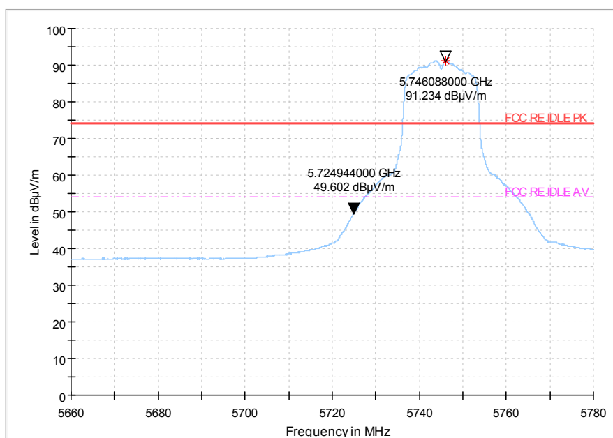
Fig. 90 Band Edges (802.11a, 5745MHz)
