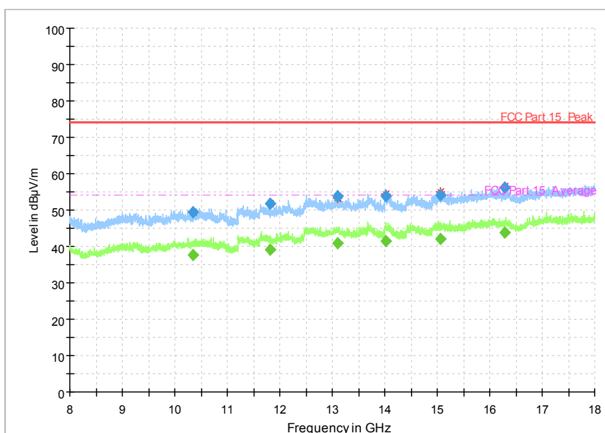
Fig. 80 Radiated Spurious Emission (802.11a, Ch149, 8 GHz-18 GHz)
