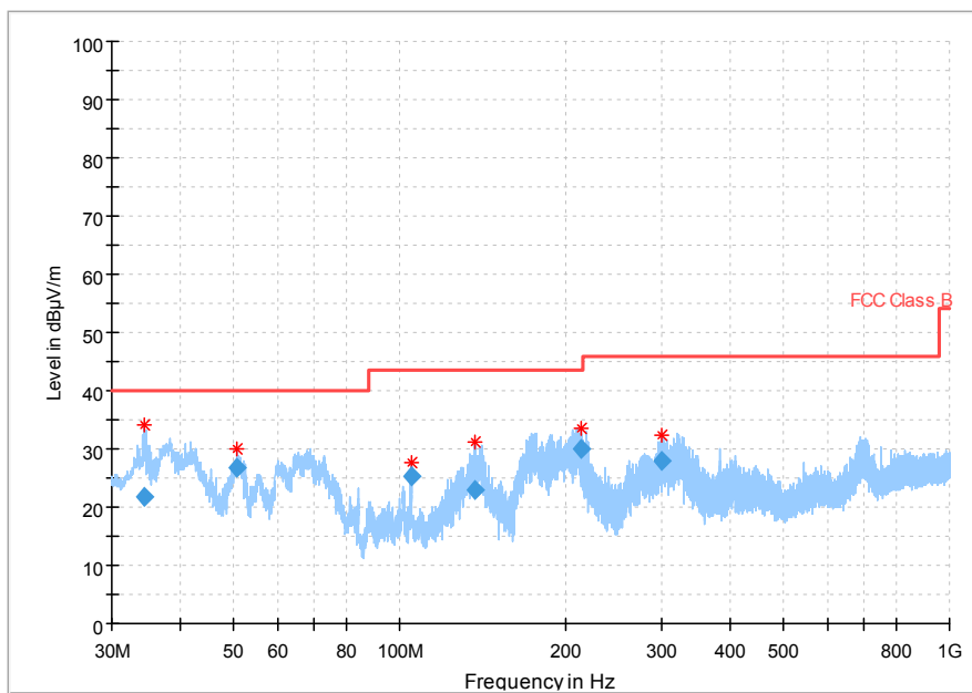
Fig. 58 Radiated Spurious Emission (802.11n-HT20, Ch165, 30 MHz-1 GHz)
