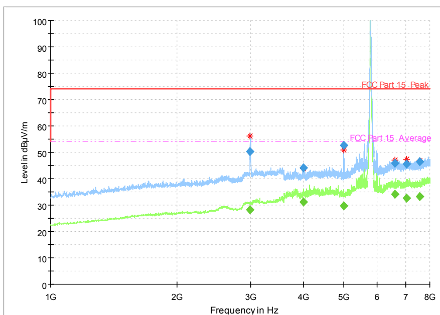
Fig. 54 Radiated Spurious Emission (802.11n-HT20, Ch157, 1 GHz-8 GHz)
