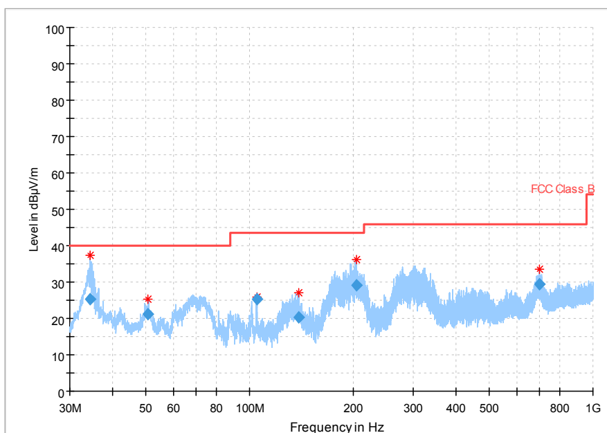
Fig. 53 Radiated Spurious Emission (802.11n-HT20, Ch157, 30 MHz-1 GHz)
