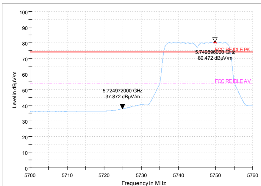
Fig. 89 Band Edges (802.11n20, 5745MHz)
