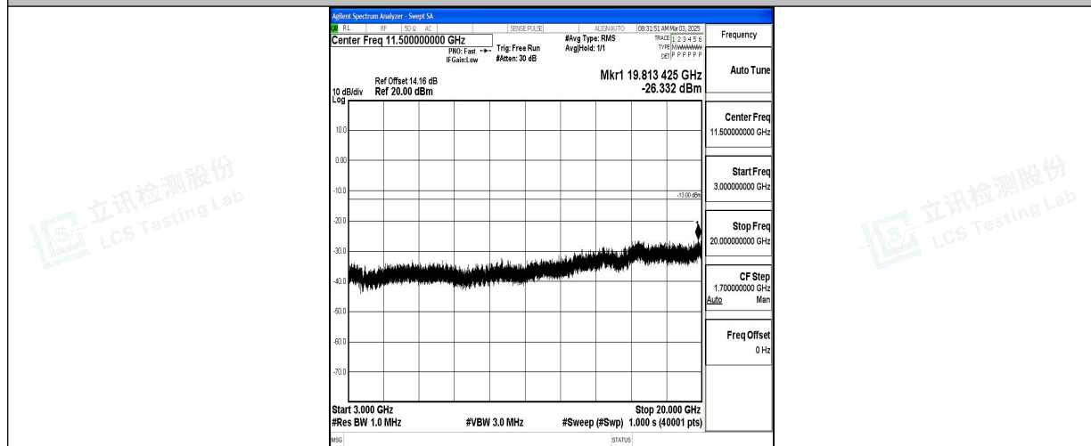
Band66_15MHz_16QAM_132047_1RB#0_3000~20000_3000~20000
