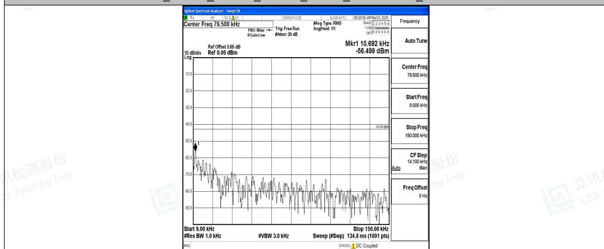
Band66_10MHz_QPSK_132622_1RB#0_0.009~0.15_0.009~0.15
