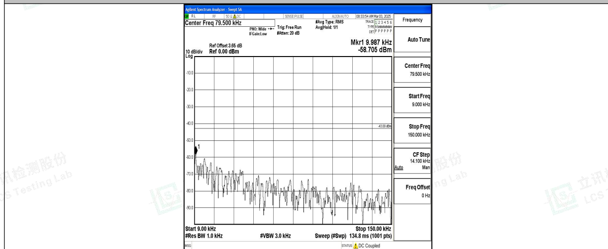
Band66_15MHz_QPSK_132597_1RB#0_0.009~0.15_0.009~0.15
