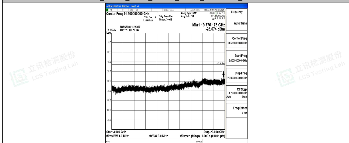
Band66_10MHz_QPSK_132622_1RB#0_3000~20000_3000~20000
