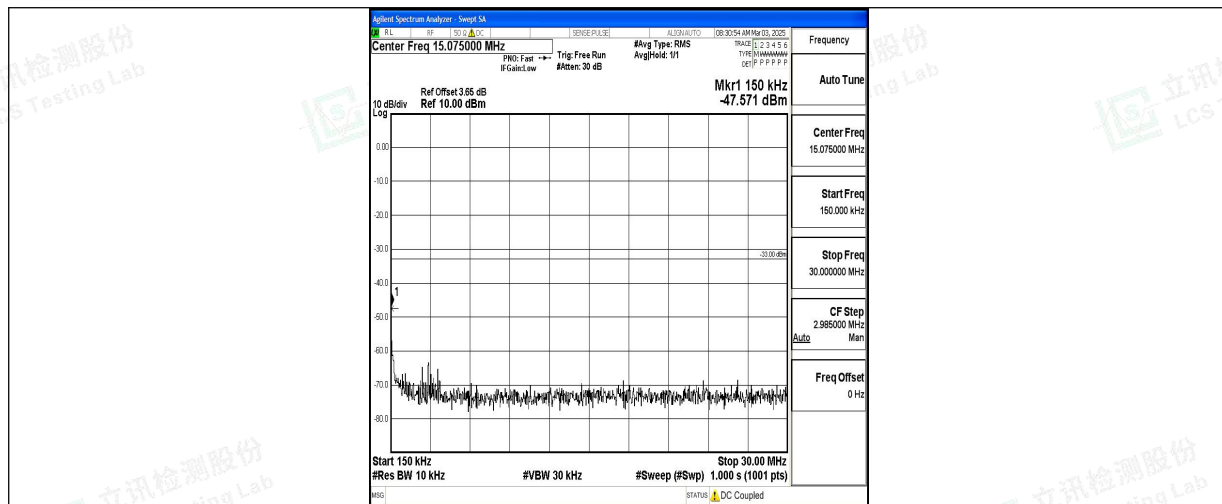
Band66_15MHz_QPSK_132047_1RB#0_0.15~30.015~30.015
