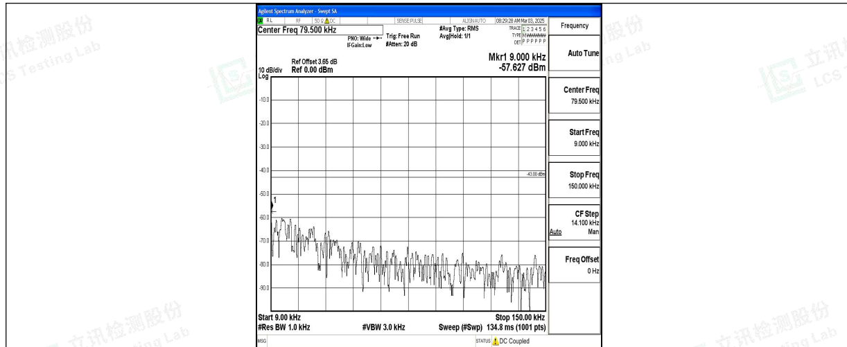
Band66_10MHz_16QAM_132622_1RB#0_0.009~0.15_0.009~0.15
