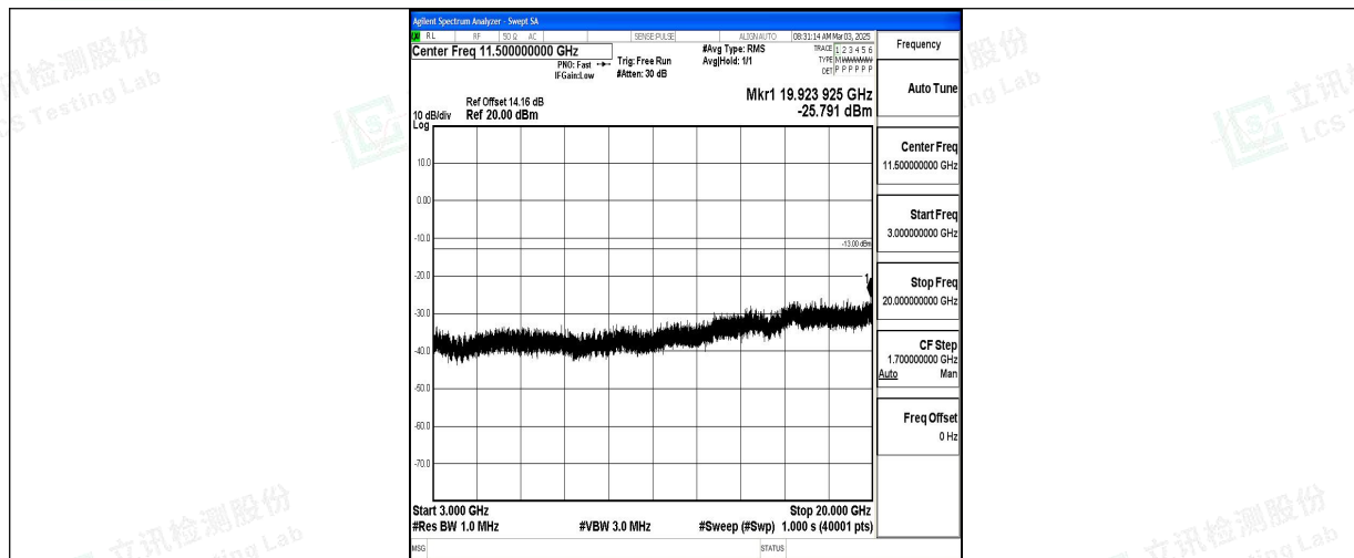
Band66_15MHz_QPSK_132047_1RB#0_3000~20000_3000~20000
