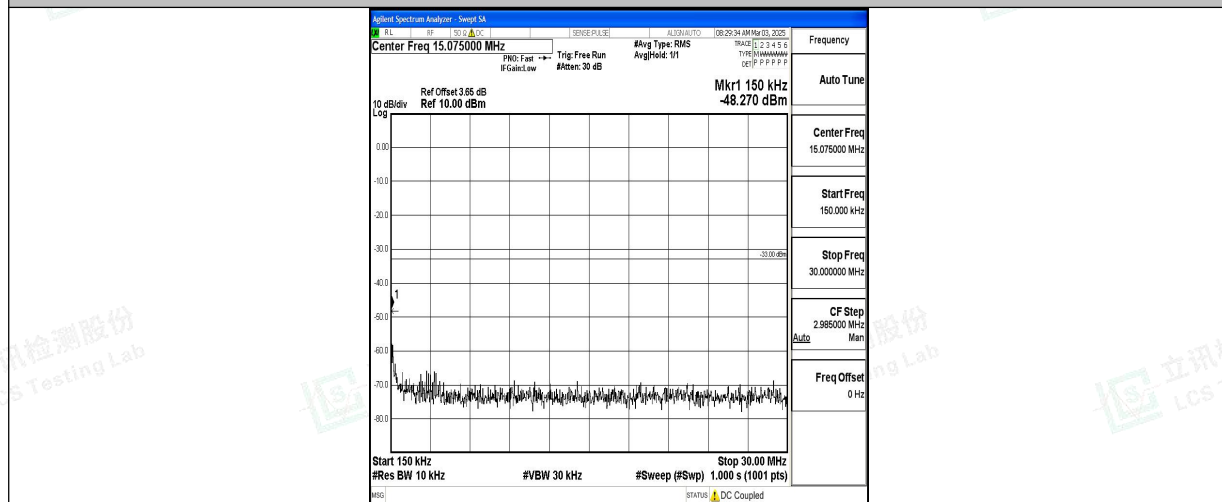
Band66_10MHz_16QAM_132622_1RB#0_0.15~30_0.15~30
