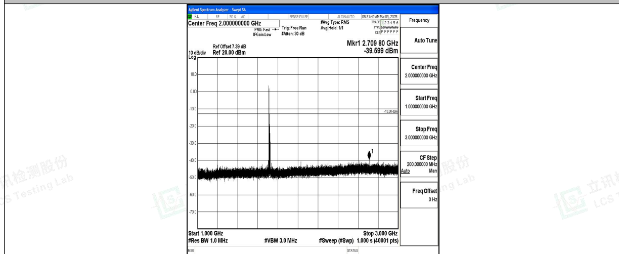
Band66_15MHz_16QAM_132047_1RB#0_1000~3000_1000~3000
