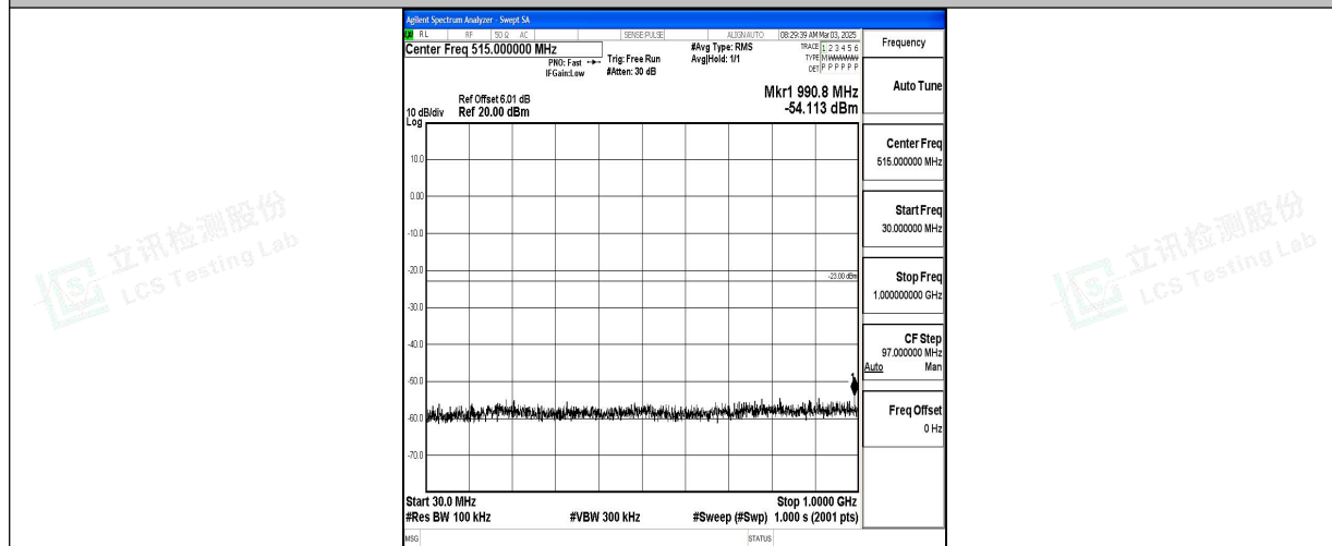
Band66_10MHz_16QAM_132622_1RB#0_30~1000_30~1000
