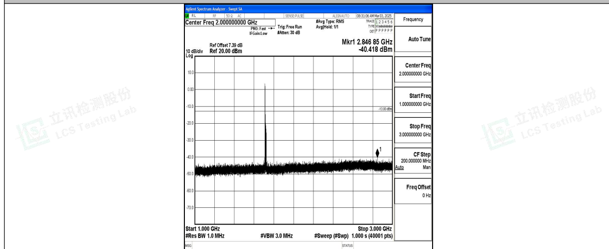
Band66_15MHz_QPSK_132047_1RB#0_1000~3000.1000~3000.1000
