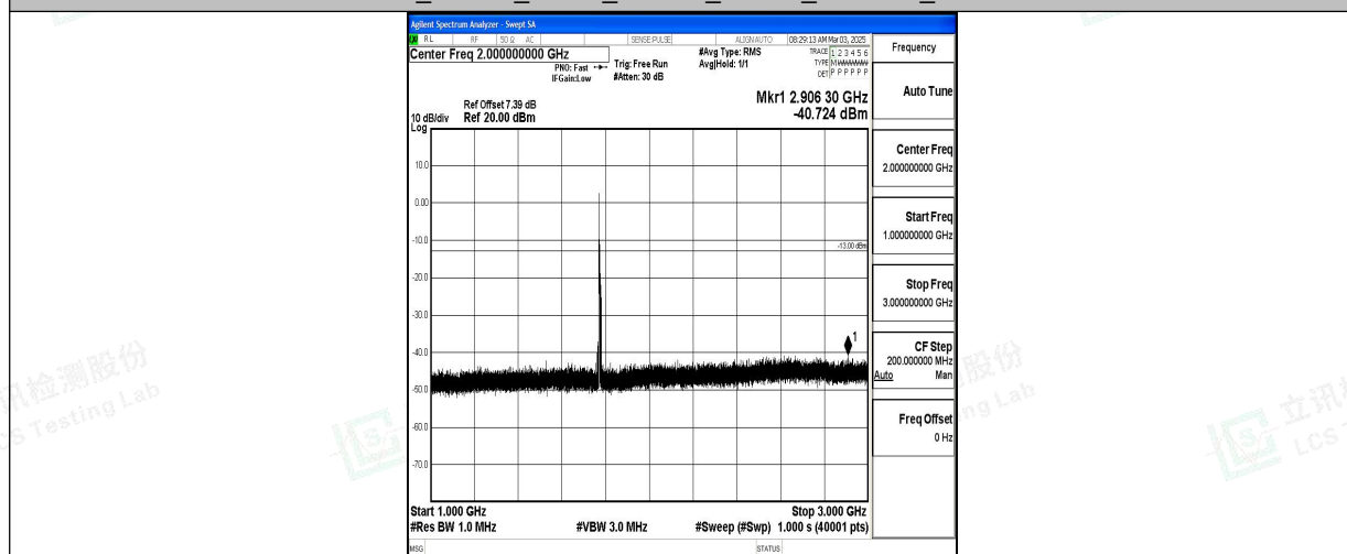
Band66_10MHz_QPSK_132622_1RB#0_1000~3000_1000~3000
