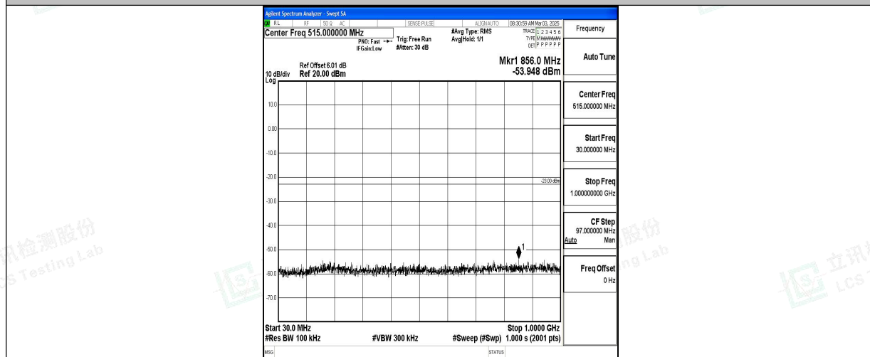
Band66_15MHz_QPSK_132047_1RB#0_30~1000.030~1000.030
