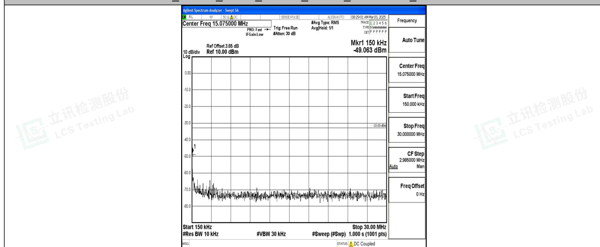
Band66_10MHz_QPSK_132622_1RB#0_0.15~30_0.15~30
