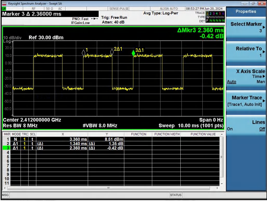
802.11g 2412MHz
