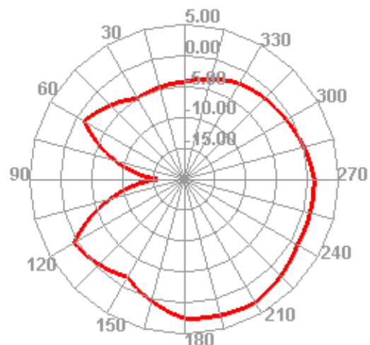
2.4G phi=90deg
