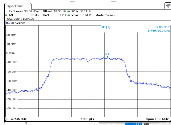
802.11n20_5745MHz_Chain 1
