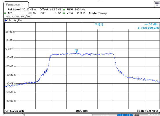
802.11a_5785MHz_Chain 0
