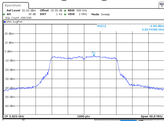
802.11a_5825MHz_Chain 0
