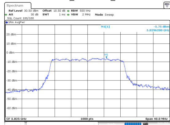
802.11n20_5825MHz_Chain 1
