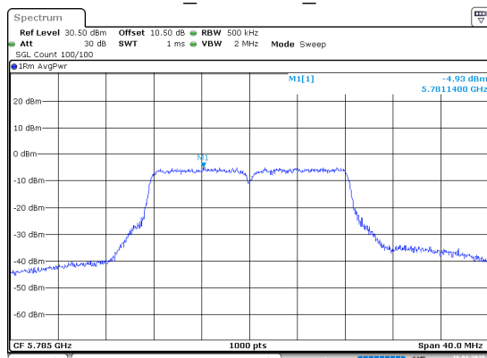
802.11a_5785MHz_Chain 1
