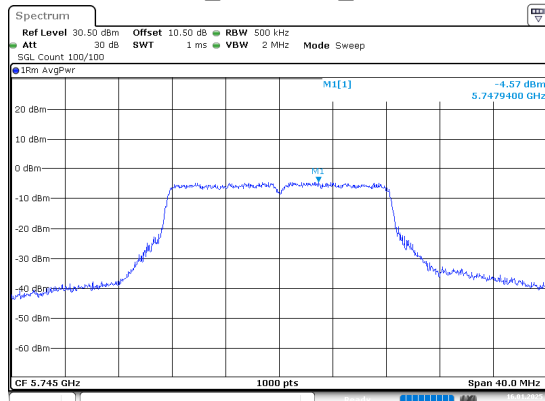
802.11a_5745MHz_Chain 0
