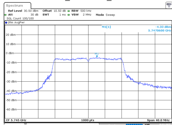
802.11a_5745MHz_Chain 1
