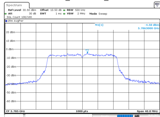
802.11n20_5785MHz_Chain 0
