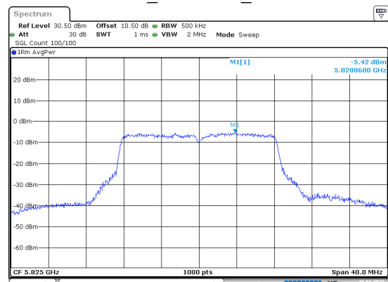
802.11a_5825MHz_Chain 1
