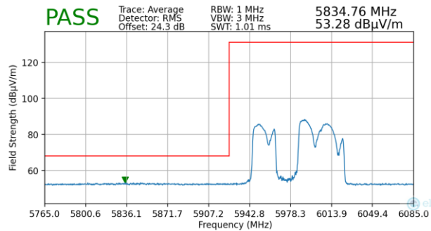
Plot 7-401. Radiated Lower Band Edge Plot MIMO (Average – UNII Band 5 – 996T+484T)
