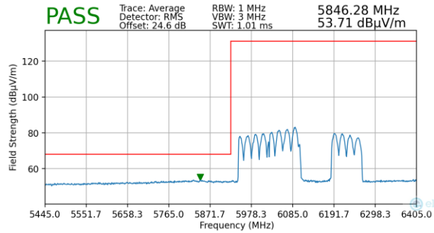
Plot 7-409. Radiated Lower Band Edge Plot MIMO (Average – UNII Band 5 – 2x996T+484T)
