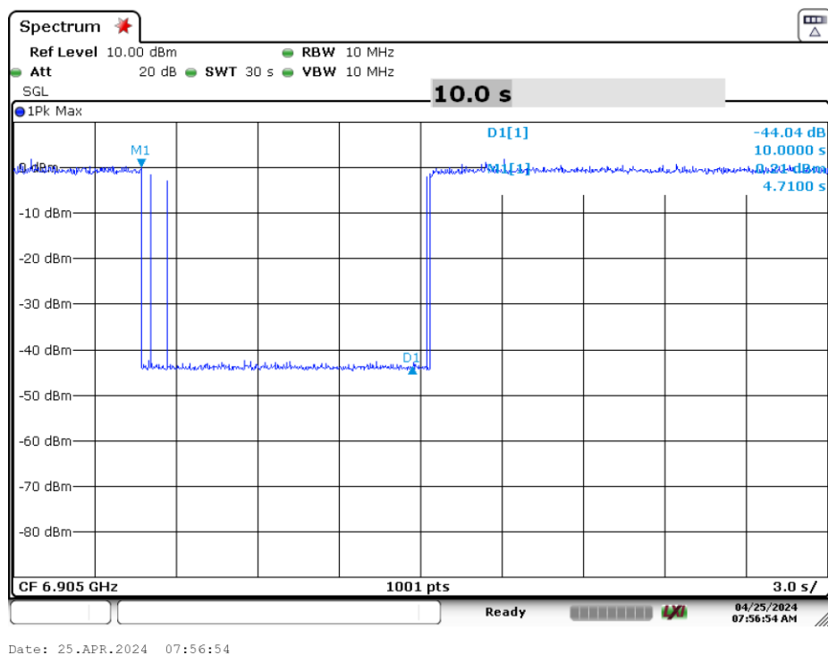
Plot 7-364. Contention Based Protocol Timing Plot (320MHz (UNII Band 8) – Ch. 191 Mid)
