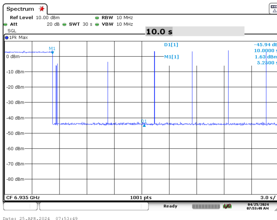
Plot 7-362. Contention Based Protocol Timing Plot (20MHz (UNII Band 8) – Ch. 197)
