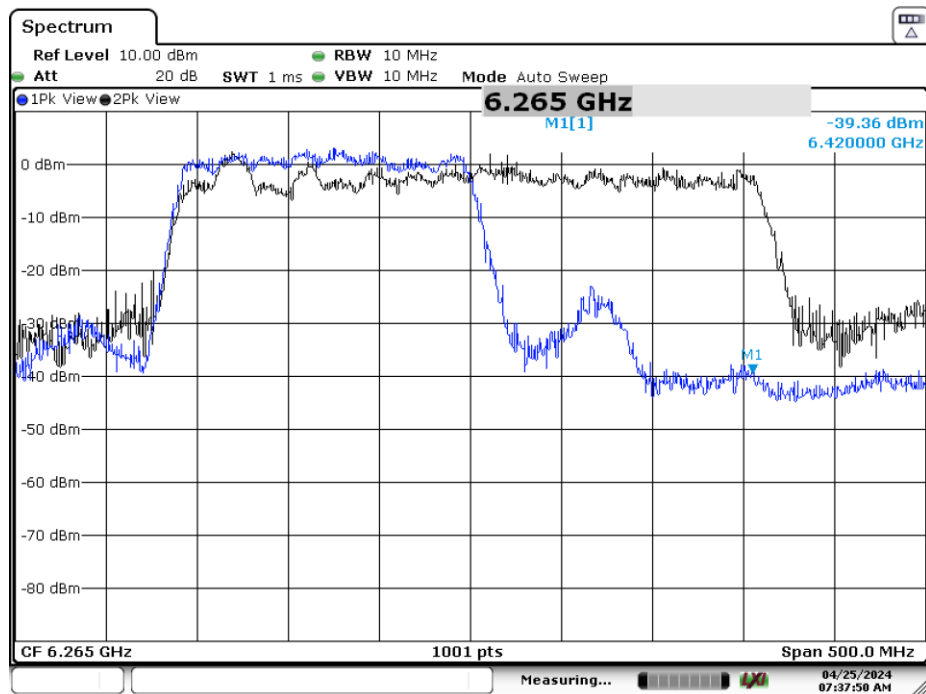
Plot 7-368. CBP 320MHz Channel - Injection Upper Edge – [6420 MHz]
