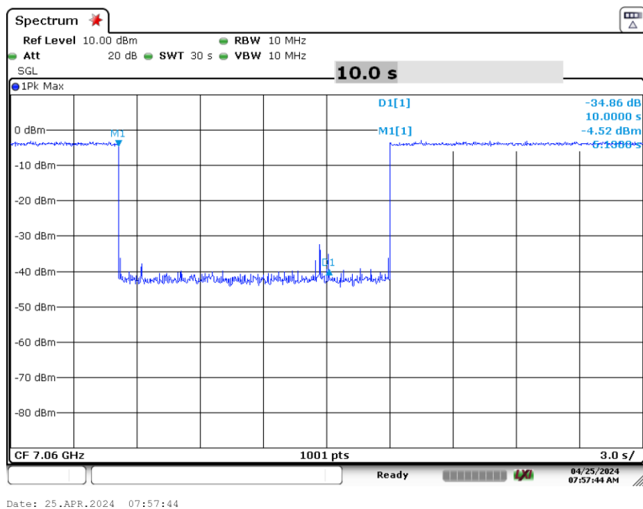
Plot 7-365. Contention Based Protocol Timing Plot (320MHz (UNII Band 8) – Ch. 191 High)
