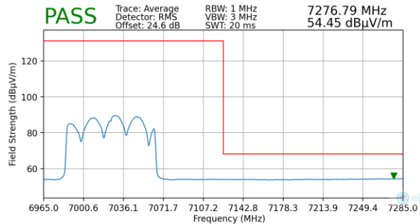
Plot 7-399. Radiated Upper Band Edge Plot MIMO (Average – UNII Band 8 – 996T)
