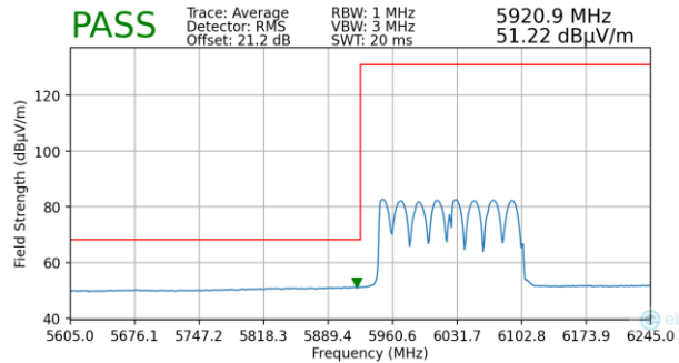
Plot 7-405. Radiated Lower Band Edge Plot MIMO (Average – UNII Band 5 – 2x996T)
