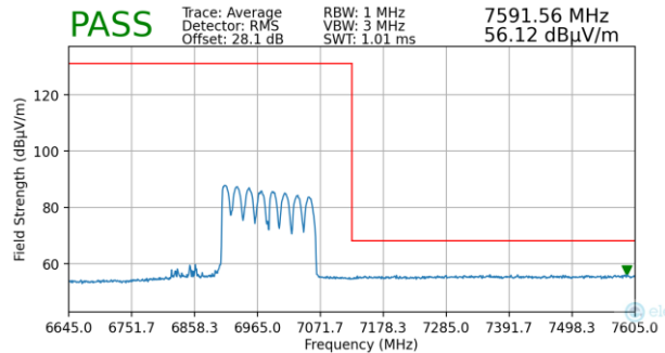
Plot 7-415. Radiated Upper Band Edge Plot MIMO (Average – UNII Band 8 – 2x996T)
