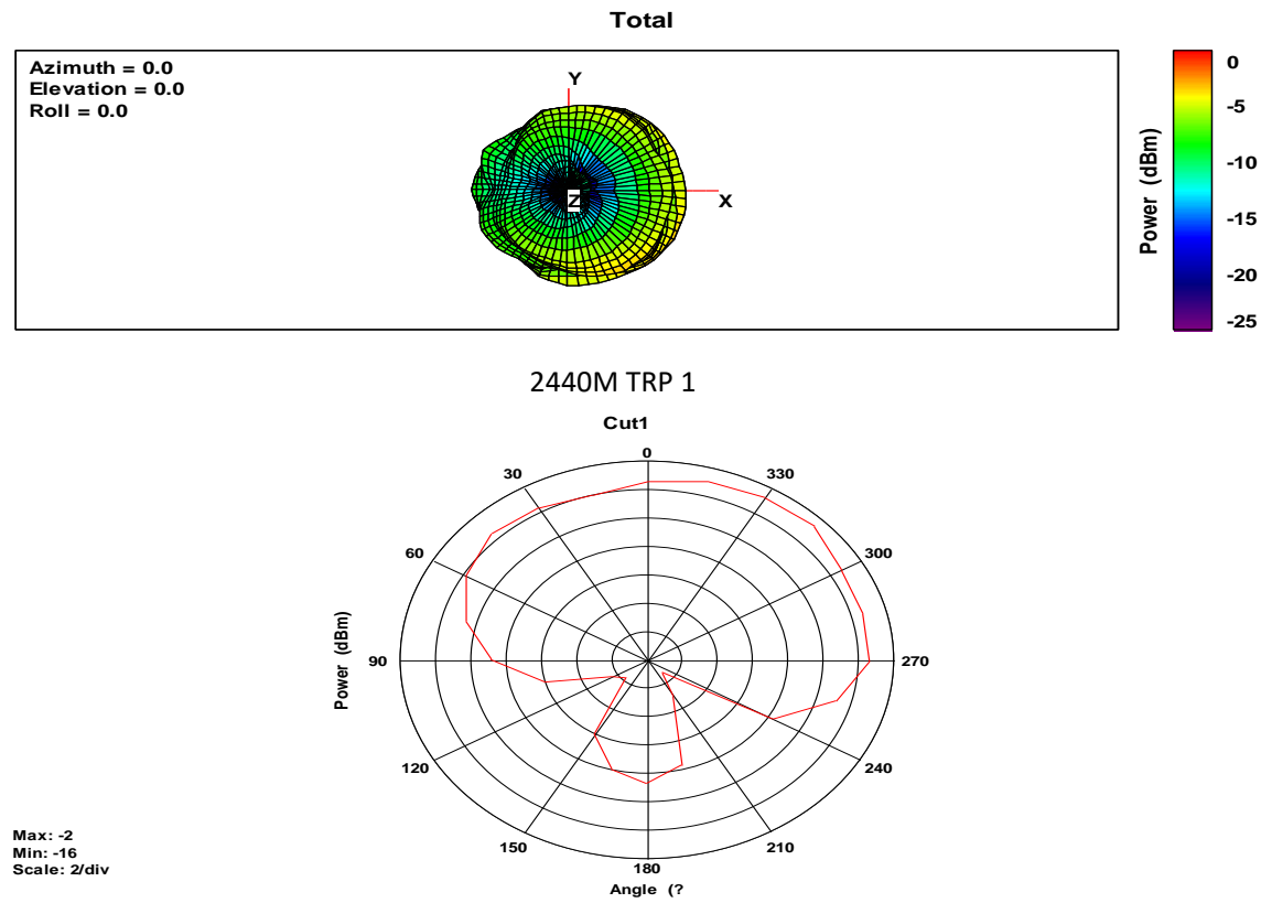
3D and 1D Radiation Patterns
